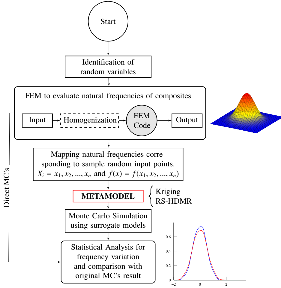
Figure 6: Flowchart of stochastic free vibration analysis of FG-CNTRC plates using Kriging and RS-HDMR metamodelling.
