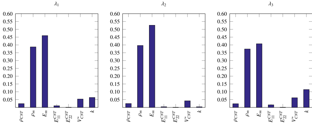
Figure 11: Sensitivity indices with respect to the first three natural frequencies for combined variation of all the variables of CCCC P-FGV plates ( a/b = 1 , h/b = 0.1 , \bar{V}_{CNT}^* = 0.11 , 256 samples).
