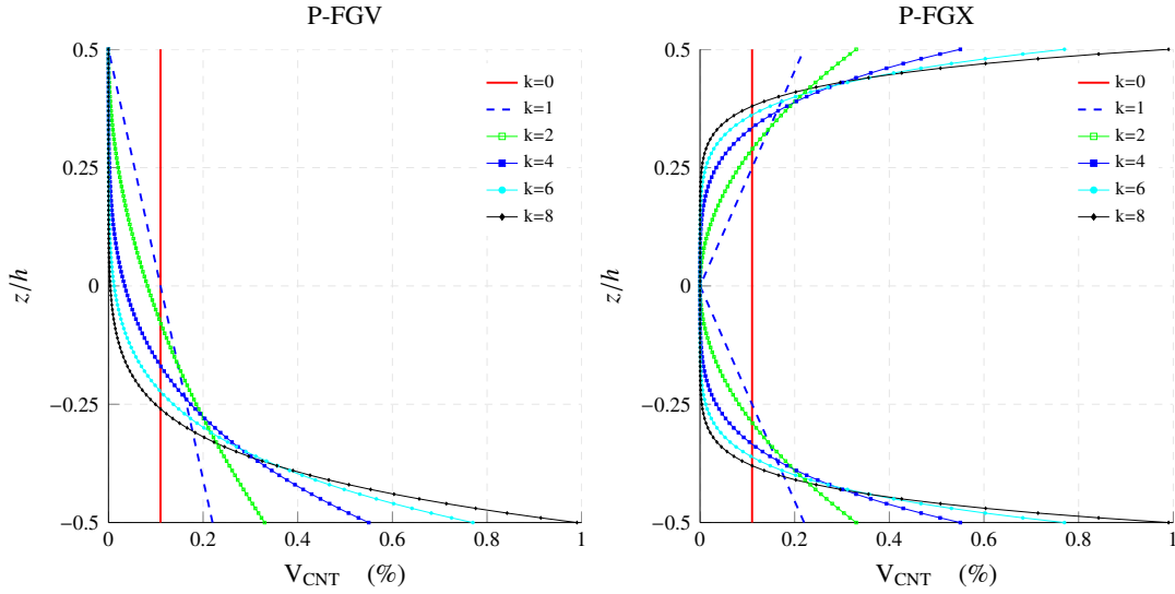
Figure 2: Variation of the CNT volume fraction through the thickness defined by the power-law distribution function for different power law indices k , based on FG-V and FG-X linear distributions, namely P-FGV and P-FGX ( V_{CNT}^* = 0.11 ).
