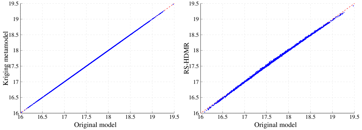
Figure 9: Scatter plot of Kriging and RS-HDMR metamodelling with respect to the original model for the first natural frequency ( \lambda_1 ) for simultaneous variation of the material parameters (CCCC UD-CNTRC plate, a/b = 1 , h/b = 0.1 , \bar{V}_{CNT}^* = 0.11 ).
