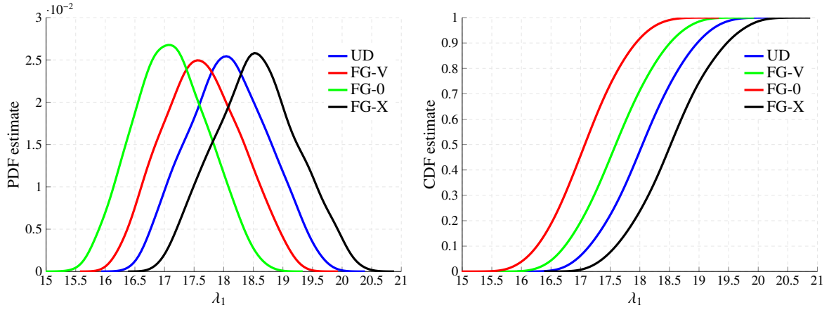
Figure 8: Probability density functions (PDF) and cumulative density functions (CDF) of CCCC FG-CNTRC plates with linear grading profiles and simultaneous variation of the material parameters. ( a/b = 1 , h/b = 0.1 and \bar{V}_{CNT}^* = 0.11 , 10,000 samples).
