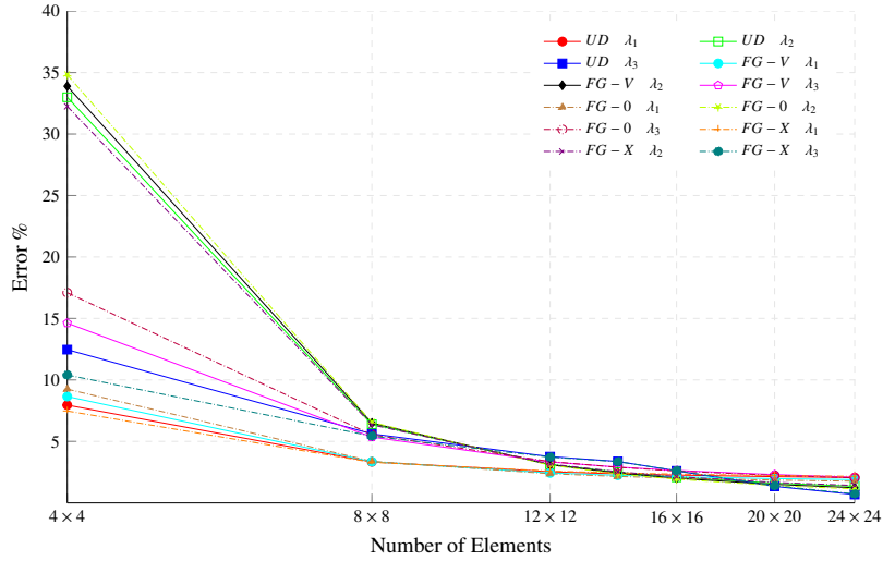
Figure 7: Convergence of errors of the first three frequency parameters ( \lambda_i , i = 1, 2, 3 ) with respect to the results provided by Zhu et al. [11] and to the mesh size ( N \times N ) of CCCC FG-CNTRC plates ( a/b = 1 , h/b = 0.1 and \bar{V}_{CNT}^* = 0.11 ).
