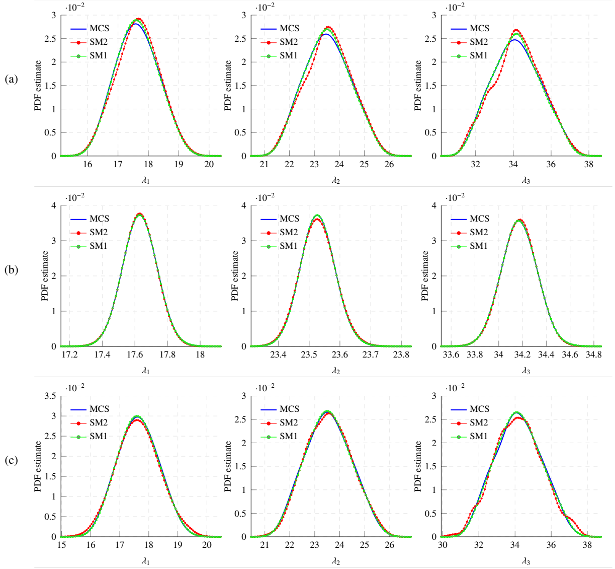
Figure 10: Comparison of the probability density functions (PDF) of the first three natural frequencies of P-FGV CCCC plates obtained by direct MCS (10.000 samples), Kriging (SM1) and RS-HDMR (SM2) metamodels (256 samples). (a) variation of the material parameters with linear reinforcement profile, (b) variation of the reinforcement grading profile and (c) combined variation. ( a/b = 1 , h/b = 0.1 , \bar{V}_{CNT}^* = 0.11 ).
