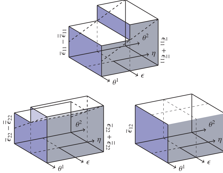
Figure 4: Schematic representation of the piecewise constant extensional strain ( \varepsilon ) approximation.
