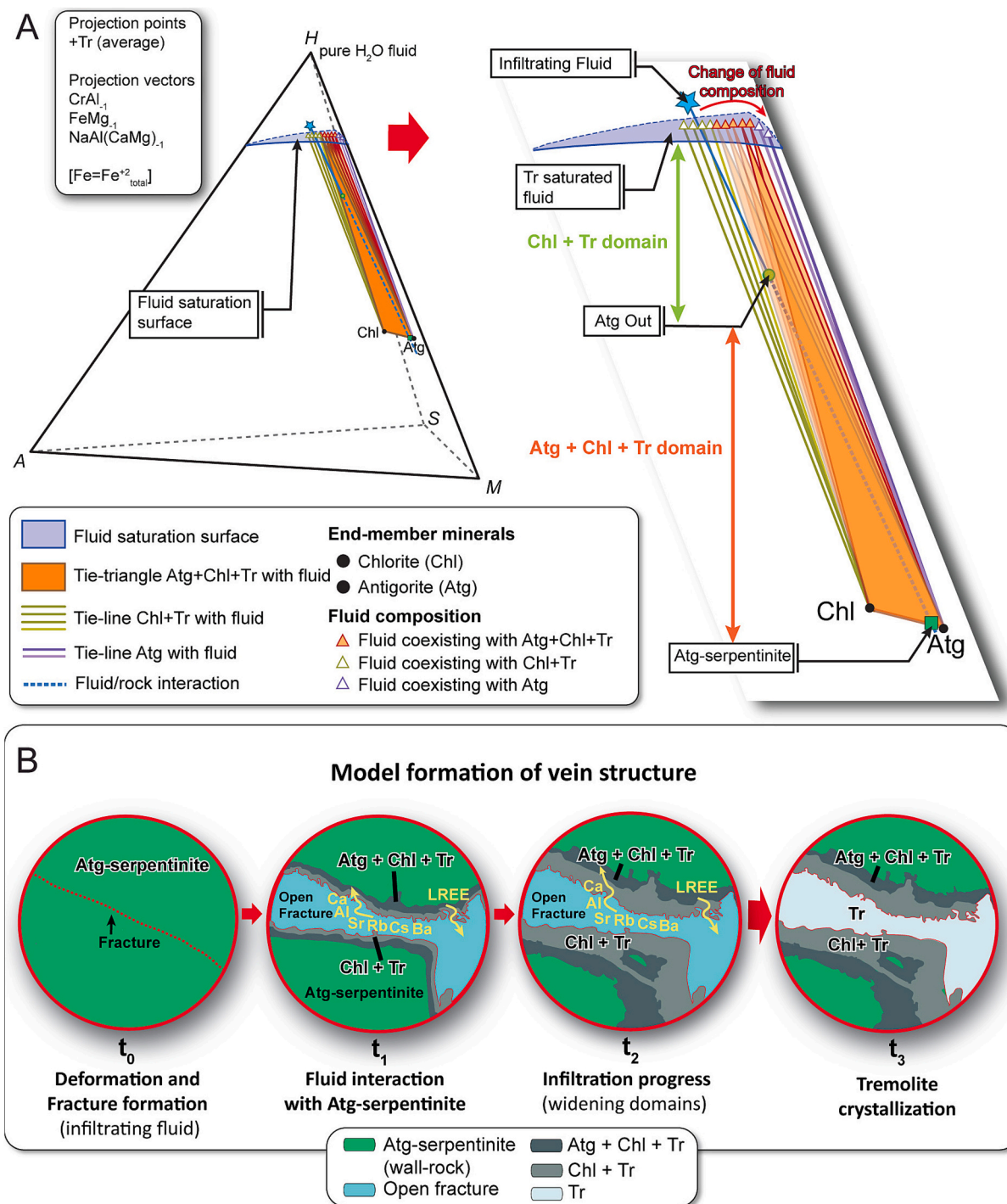
Fig. 9. Model of blackwall assemblage formation. A) Phase diagram in the MASH system showing phase relations and metasomatic zone development. All relations involving the composition of the fluid are hypothetical. The diagram is projected from Tr (average) and exchange vectors. Green tie-lines and orange tie-triangles correspond to the fields of Chl + Tr + Fluid and Atg + Chl + Tr + Fluid, respectively. Note that infiltration of fluid (blue star) in antigorite (Atg + Chl, green square) would drive the bulk composition towards the fluid, with the development of the indicated assemblages as a function of fluid/rock ratio. Reaction progress triggers decrease in Al (as indicated by colored triangles of fluid composition) and Ca (not shown) in the fluid. B) Vein formation events. t 0 : brittle deformation likely triggered by hydrofracturing; t 1 and t 2 : progressive formation of the Atg + Chl + Tr and Chl + Tr domains; t 3 : tremolite crystallization in the open fracture and migration of remaining fluid out of the system. See text for details. (For interpretation of the references to colour in this figure legend, the reader is referred to the web version of this article.)
