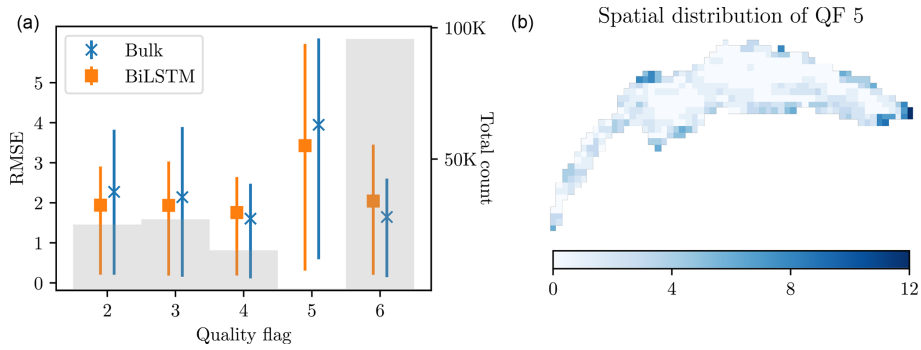
Figure 12. Analysis of BiLSTM performance in the DA run with respect to the different quality flags. (a) LSWT difference with respect to bulk temperature (in blue) and BiLSTM predictions (in orange) as a function of QF. The faint gray bars show the total number of LSWT measurements associated with the QF. (b) Spatial distribution of LSWT measurement availability for QF 5.
