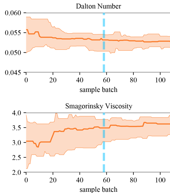
Figure 4. Evolution of the 16 Markov chain parameters. The solid lines indicate the median, and the semi-transparent spreads indicate the 5th–95th percentiles across multiple concurrent chains of the sampler. The vertical dashed blue line indicates the end of the specified burn-in period used to determine the posterior distribution.
