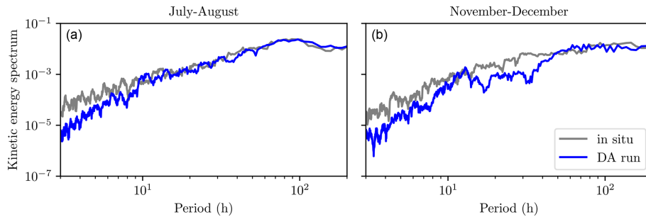
Figure 10. Kinetic energy spectra computed from the ADCP sensors at the LÉXPLORE platform (gray) and from the DA run (blue). Profiles based on 15 m deep dynamics use July–August data for panel (a) and November–December data for panel (b).
