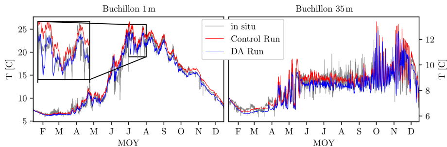
Figure 7. Evolution of temperature at the Buchillon station for the 1 m (left) and 35 m (right) sensors for the year 2019. The gray line is the in situ measurement, the red line corresponds to the control run, and the blue line is the data-assimilated prediction. The small inset on the left shows the improvement from the assimilated run for the 1 m sensor in greater detail for July.
