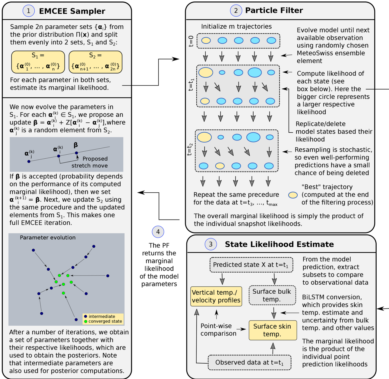
Figure 2. A simplified visualization of the data assimilation framework that we use in this paper. The EMCEE sampler proposes 2n walkers (also called chains in SPUX), whose marginal likelihood is then evaluated using the particle filter (PF). The PF resamples trajectories via deletion/replication with respect to their dataset and observational error model.
