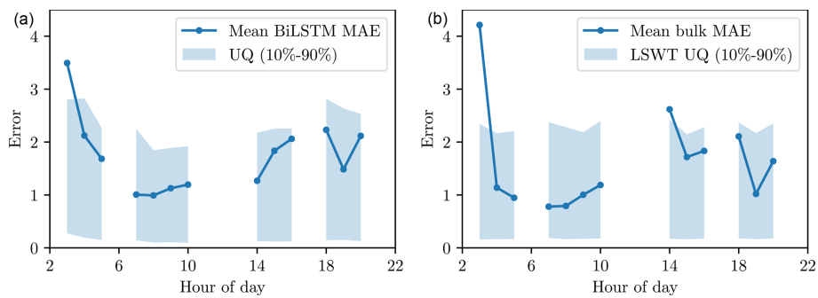
Figure 13. (a) Mean BiLSTM prediction error (dark blue line) and the 10th–90th percentiles of the uncertainties predicted by BiLSTM (shaded areas) for the different hours of the day. (b) Mean bulk temperature prediction error (dark blue line) and the 10%–90% uncertainty estimates based on Lieberherr and Wunderle (2018).
