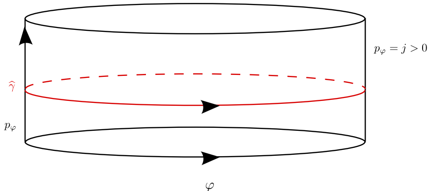
FIG. 2. Phase space (\varphi, j) for j > 0 corresponding to different trajectories \hat{\gamma} .
