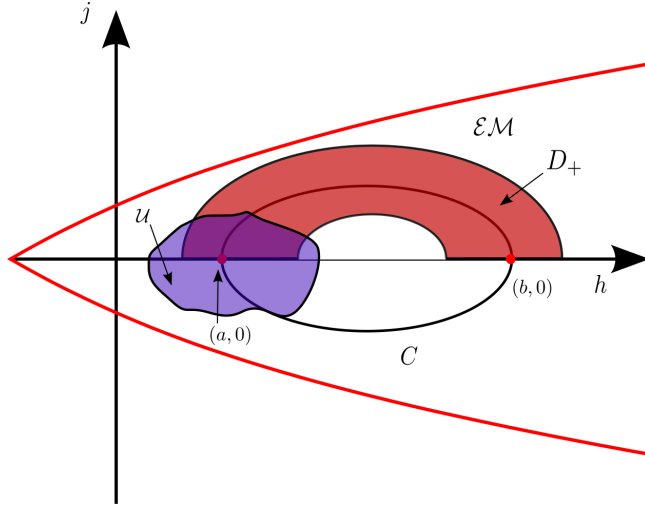
FIG. 6. Domain D_+ in a neighbourhood of C \cap \{j > 0\} , and neighbourhood of (a, 0) , \mathcal{U} , in which the actions \tilde{I}_1 and \tilde{I}_2 , are smooth functions of (h, j) .
