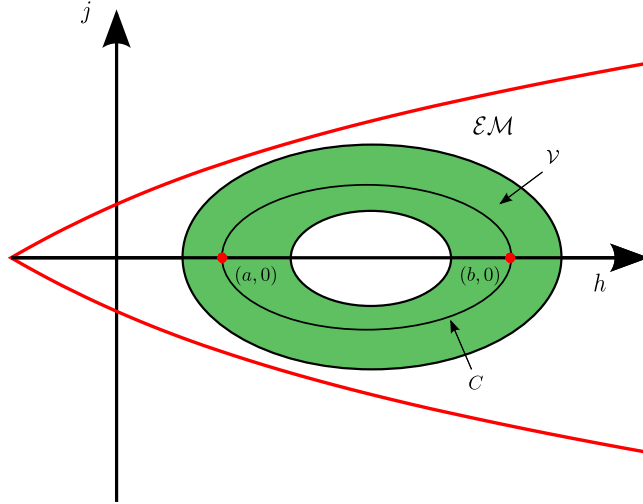
FIG. 7. Neighborhood of C , \mathcal{V} , where the action variables \mathcal{I}_i = \mathcal{I}_i(h, j) , with i = 1, 2 are defined.
