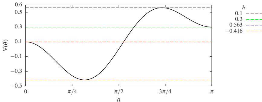
FIG. 11. Interaction potential V(\theta) = 1.1 \cos^3 \theta + 0.2 \cos^2 \theta - 1.2 \cos \theta , the horizontal lines represent the energies at the singular points at j = 0 .
