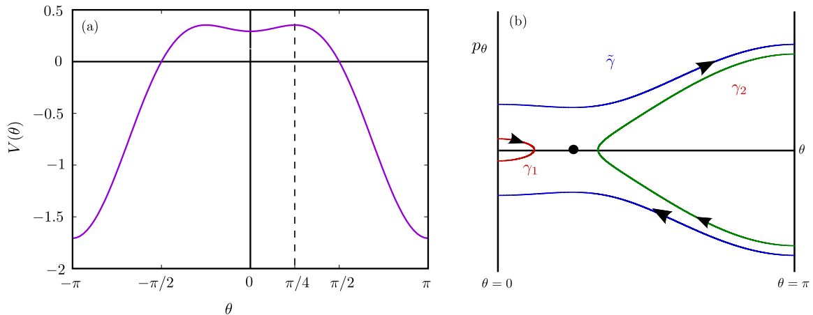
FIG. 3. (a) Potential V(\theta) = \cos \theta - \frac{\sqrt{2}}{2} \cos^2 \theta as a function of \theta , and (b) the orbits \gamma_1 and \gamma_2 with h_1 in the interval V(0) < h_1 < V(\pi/4) , and \tilde{\gamma} with h_2 satisfying h_2 > V(\pi/4) as a function of \theta . The orbit \tilde{\gamma} corresponds to motions through a meridian of the sphere.
