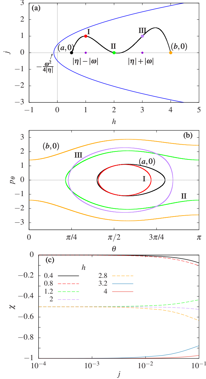
FIG. 9. For the modified spherical pendulum with \omega = -1 and \eta = -2 , (a) the energy momentum plane \mathcal{EM} and tori \text{I}=(1,1) , \text{II}=(2,0) and \text{III}=(3,1) (full points) along a path connecting (a,0) = (0.5,0) and (b,0) = (4,0) , (b) projections of the tori on the plane (\theta, p_\theta) , and (c) \chi(h, j) as a function of j for several values of h .
