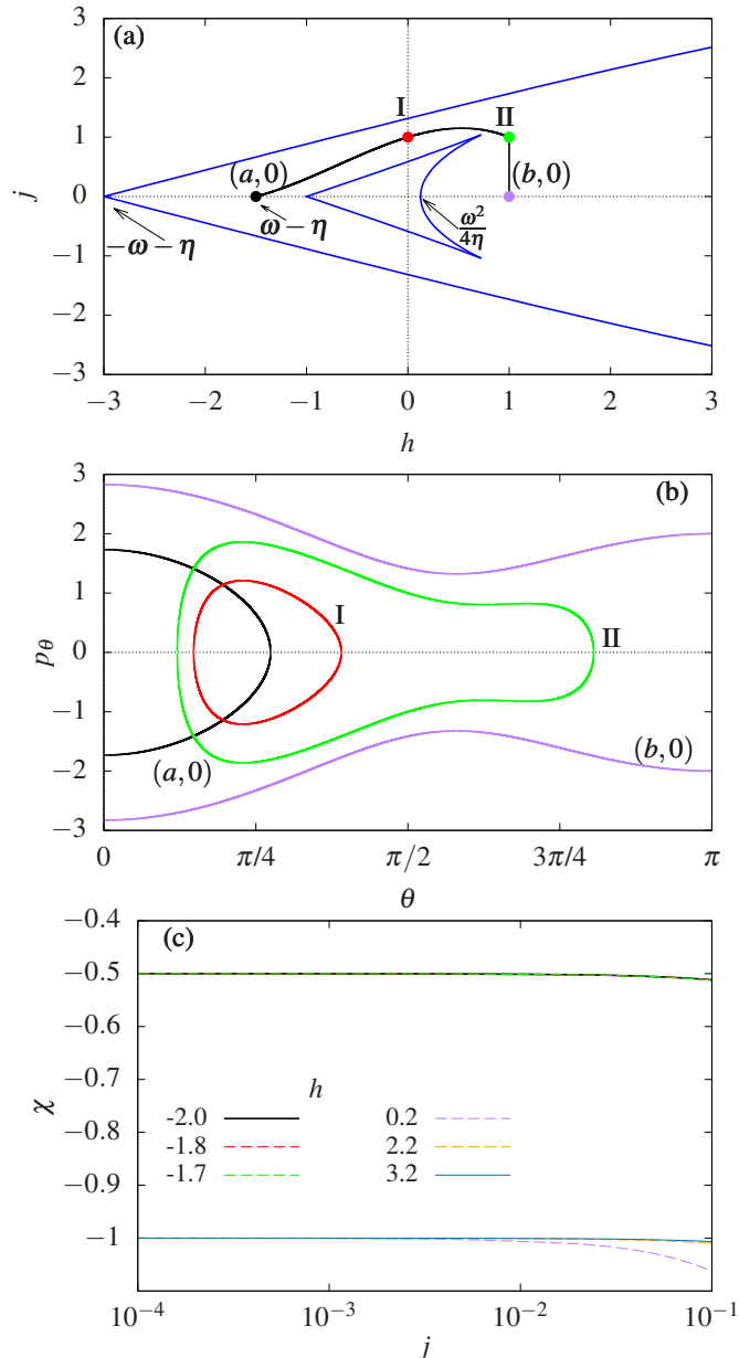
FIG. 10. For the modified spherical pendulum with \omega = 1 and \eta = 2 , (a) the energy momentum plane \mathcal{EM} and tori I=(0, 1) and II=(1, 1) (full points) along a path connecting (a, 0) = (-1.5, 0) and (b, 0) = (1, 0) , (b) projections of the tori on the plane (\theta, p_\theta) , and (c) \chi(h, j) as a function of j for several values of h .
