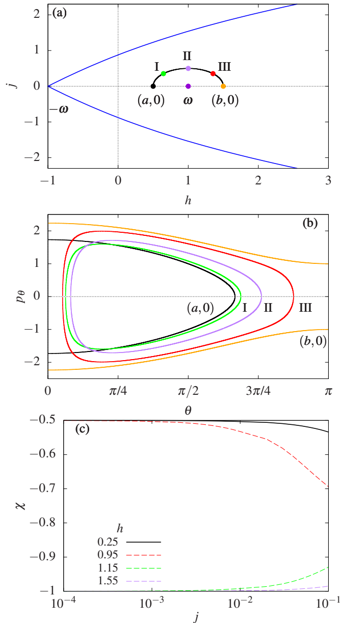
FIG. 8. For the spherical pendulum with \omega = 1 , (a) the energy momentum plane \mathcal{EM} and tori I= (1 - \frac{\sqrt{2}}{4}, \frac{\sqrt{2}}{4}) , II= (1, \frac{1}{2}) and III= (1 + \frac{\sqrt{2}}{4}, \frac{\sqrt{2}}{4}) (full points) along a path connecting (a, 0) = (\frac{1}{2}, 0) and (b, 0) = (\frac{3}{2}, 0) around the singular point (0, \omega) (b) projections of the tori on the plane (\theta, p_\theta) , and (c) \chi(h, j) as a function of j for several values of h .
