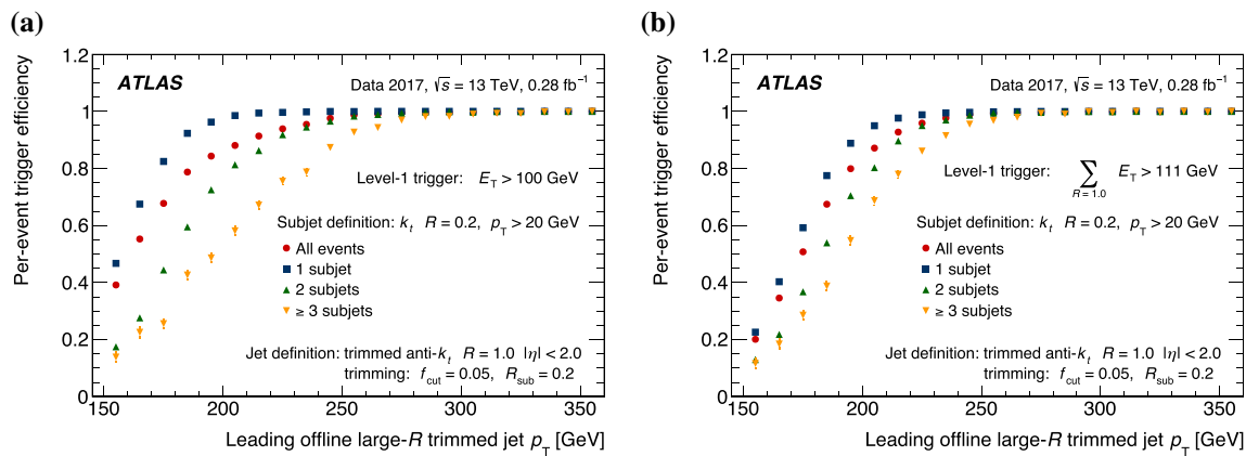
Fig. 10 Trigger efficiency curves as a function of the leading offline trimmed jet p_T [30] for events with jets of one, two or more than two subjets selected using a the standard jet sliding-window algorithm and b the L1Topo simple cone algorithm
