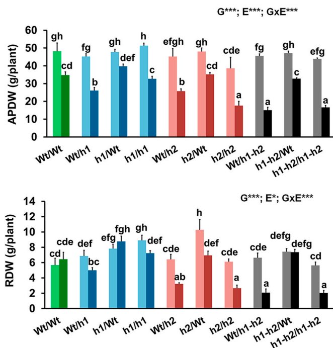
Fig. 3. Growth expressed as aerial part dry weight (APDW) and root dry weight (RDW) in reciprocal rootstock/scion combinations with non-silenced (Wt), single RNAi-silenced lines for SchHKT1;1 (h1) and SchHKT1;2 (h2), as well as double-silenced lines at both loci (h1-h2) grown under control and saline conditions. Grafted combinations were cultivated in vermiculite in 17L pots irrigated with 1x Hoagland solution and treated for 60 d with 0 mM NaCl (clear bars) and 70 mM NaCl (dark bars) under natural greenhouse conditions during the fall-spring season (November–April). Values represent mean \pm standard error of six different samples. Data were analyzed by two-way ANOVA using genotype (G), salt treatment (E) and their interaction (GxE) as sources of variation. Their significance was evaluated (P-value, not significant, ns, *P < 0.05, **P < 0.01, ***P < 0.001). Significant differences are indicated by different letters according to Fisher's LSD test (P < 0.05).
