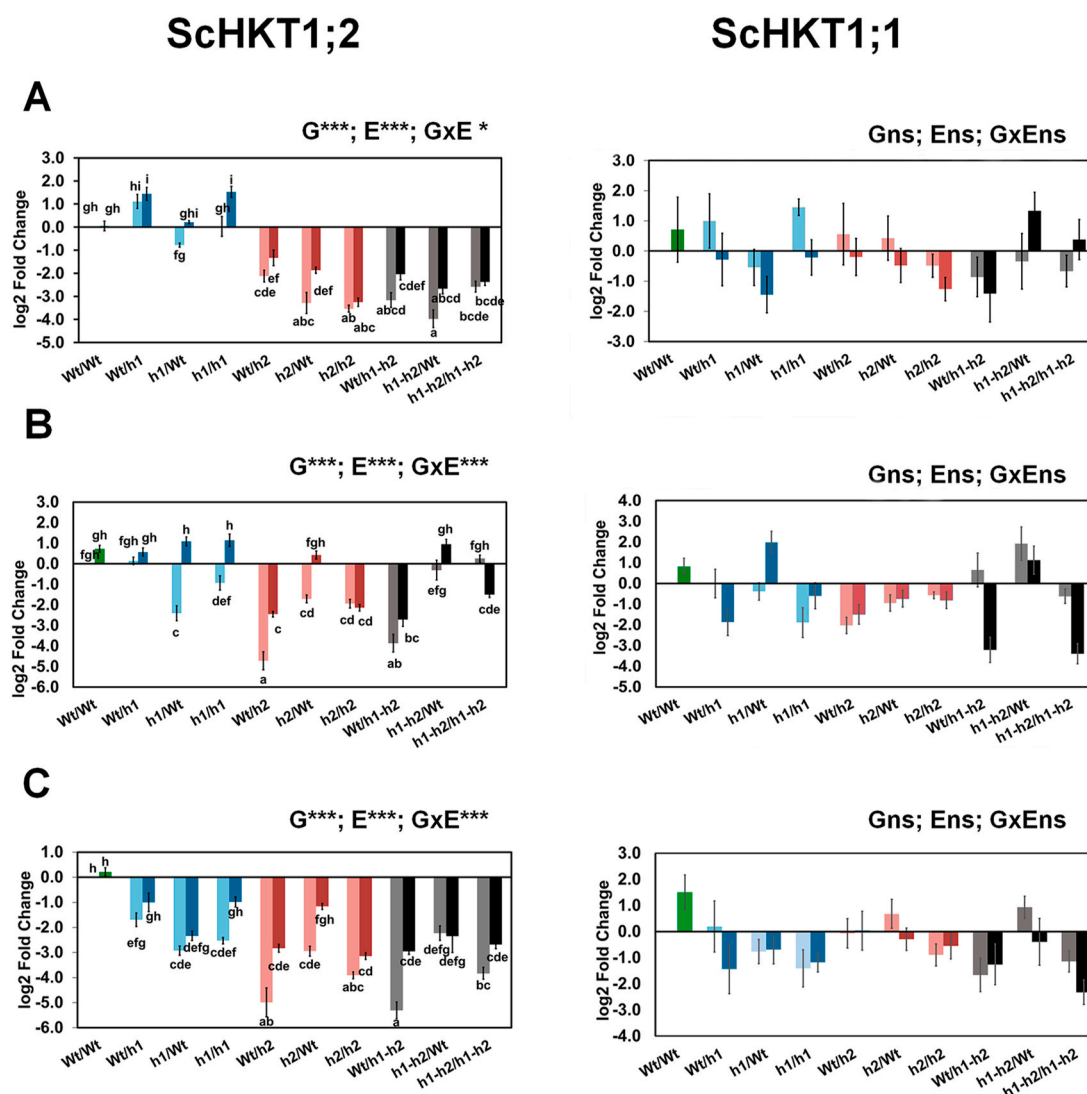
Fig. 2. Transcript levels of SchKTI;2 and SchKTI;1 in root (A), leaf (B) and flower (C) tissues in reciprocal rootstock/scion combinations with non-silenced (Wt), single RNAi-silenced lines for SchKTI;1 (h1) and SchKTI;2 (h2), as well as double silenced lines at both loci (h1-h2) grown under control and saline conditions. Total RNA was purified from roots, the 7 th leaf and 1 st floral inflorescence, including the peduncle, pedicel and floral receptacle of grafted combinations cultivated in vermiculite in 17 L pots irrigated with 1x Hoagland solution and treated for 30 d with 0 mM NaCl (clear bars) and 70 mM NaCl (dark bars) under natural greenhouse conditions during the fall-spring season (November–April). The tomato elongation factor gene, LeEF-1 \alpha , was used as the reference gene. The results show an increase or decrease in the transcript levels of each HKTI;2 gene in relation to the levels for roots, leaves and flowers of the Wt/Wt combination graft cultivated in the absence of stress, to which the value 0 was assigned. Each value is the mean \pm the standard error of nine replicates for roots and flowers (three biological and three technical replicates). Data were analyzed by two-way ANOVA using genotype (G), salt treatment (E) and their interaction (GxE) as sources of variation. Their significance was evaluated (P-value, not significant, ns, * P < 0.05 , ** P < 0.01 , *** P < 0.001 ). Significant differences are indicated by different letters according to Fisher's LSD test ( P < 0.05 ).
