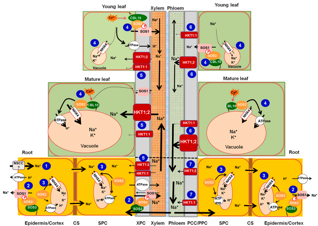
Fig. 9. A hypothetical model for the role of SchHKT1;1 and SchHKT1;2 \text{Na}^+/\text{K}^+ transporters in \text{Na}^+/\text{K}^+ homeostasis in tomato under salinity conditions. (1) \text{Na}^+ ions massively enter the cells via non selective cation channels (NSCCs) (Van Zelm et al., 2020). (2) The \text{Na}^+/\text{H}^+ antiporter SOS1, activated by the SOS2–SOS3 complex, promotes \text{Na}^+ extrusion out of the root in the epidermis and cortex cells, thus reducing the net influx of \text{Na}^+ , \text{Na}^+ loading into the xylem, and \text{Na}^+ efflux from leaves at the XPC (Oliás et al., 2009). (3) Activation of NHX4 and NHX2 by SOS2 causes \text{Na}^+ (and \text{K}^+ ) accumulation in the vacuolar and endosomal (not shown) compartments, respectively, in roots and leaves (Huertas et al., 2012, 2013). SOS2 also activates the plasma membrane and tonoplast \text{H}^+ -ATPase responsible for energizing SOS1 antiporter activity, as well as NHX2 and NHX4 (Huertas et al., 2012; 2013). (4) In aerial parts, the CBL10/SOS2 kinase complex promotes cell \text{Na}^+ extrusion by SOS1 in young leaves and intracellular \text{Na}^+ compartmentalization by NHX transporters in mature leaf tissues (Egea et al., 2018). (5) At the root XPC, HKT1-like proteins retrieve \text{Na}^+ from the xylem sap, thereby restricting the amount of \text{Na}^+ reaching the photosynthetic tissues which is probably exchanged for \text{K}^+ through other \text{K}^+ channels (Rubio et al., 2020). In the case of NIL14, the hypoactive cheesmaniae allele of HKT1;2 at the root level causes less withdrawal of \text{Na}^+ from the root xylem, again exchanged for \text{K}^+ , which remains in the root (Asins et al., 2013; Jaime-Pérez et al., 2017). Thus, more \text{Na}^+ reaches the aerial part through the transpiration current, which, together with the presence of a SchHKT1;2 hyperactive allele in XPC from the aerial part, promotes the removal of \text{Na}^+ from xylem and subsequent vacuolar accumulation in the mesophyll cells through the NHX system (4) (Jaime-Pérez et al., 2017). This would functionally explain the QTL as defined by the HKT1;2 cheesmaniae allele which determines higher \text{Na}^+ and lower \text{K}^+ accumulation in the aerial part of tomato under saline conditions, while the SchHKT1;1 \text{Na}^+ transporter in XPC appears to play a minor role in \text{Na}^+/\text{K}^+ homeostasis in the aerial part of tomato (Jaime-Pérez et al., 2017). (6) To translocate \text{Na}^+ back to the root, ions unloaded from the xylem in the symplast and apoplast from leaf mesophyll cells may be transported into the phloem via HKT1;2 and HKT1;1 transporters and \text{Na}^+ is then transferred into roots via the phloem, preventing \text{Na}^+ over-accumulation in leaves and flowers. (7) This \text{Na}^+ recirculation from aerial parts to roots is further facilitated by SchHKT1;1 silencing in root phloem cells, which promotes phloem \text{Na}^+ unloading and subsequent transport to other root compartments or extrusion back to the medium (results from this study). CS, casparian strip; SPC, stelar parenchyma cells; XPC, xylem parenchyma cells; PCC/PPC, phloem companion cells/phloem parenchyma cells. Arrow thickness indicates the hypothetical dominance of the ion flux. Gene box size indicates the gene expression levels reported in specific tissues (Asins et al., 2013; Jaime-Pérez et al., 2017).
