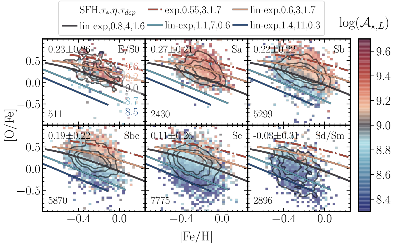
Fig. 1. Distribution of [\text{O}/\text{Fe}] as a function of [\text{Fe}/\text{H}] , for the H II regions of our sample (segregated by galaxy morphology), color coded by the average \mathcal{A}_{*,L} of the underlying stellar population. Contours represent the density of the plotted regions, encircling 95%, 80% and 40% of them, respectively, with the total number shown at the bottom-left of each panel. The average [\text{O}/\text{Fe}] value for each morphology is shown at the top-left of each panel too. The solid and dashed-dotted lines are all the same in the six panels. They correspond to the predictions by the five ChEMs described in the text, generated to cover the observed distributions. Each model is defined by the values of a set of input parameters ( \tau_* , \eta , \tau_{dep} ) and two shapes of the SFHs (exponential decay, exp , and linear rising plus exponential decay, lin-exp ), indicated in the upper legend. Lines are color coded according to the average \mathcal{A}_{*,L} too. Note that there is no exact one-to-one correspondence between a single model and the observed distribution for a single morphological bin (i.e., panel).
