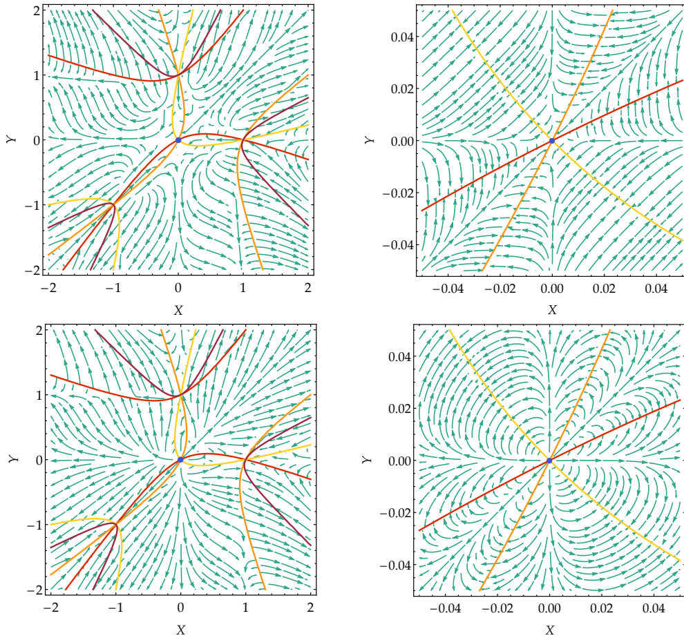
Figure 8.2.1: These plots show how the field (\xi^2, \xi^3)' = (X''', Y''') behaves with respect to X and Y under the conditions H' = X' = Y' = X'' = Y'' = 0 and H = H_{\text{ds}} . The curves in red, orange and yellow are, respectively, the three branches of singular separatrices as they appear in (8.2.23), while the dark red one is the additional separatrix that does not appear in the Hessian determinant. The isotropic solution corresponds to the blue point at the origin. We can also see other three distinctive singular points that correspond to the physical solutions where only one of the directions expands (see Table 8.2.1). The first two plots correspond to the value \beta M_{\text{Pl}}^4/H_{\text{ds}}^4 = 0.1 and the last ones to \beta M_{\text{Pl}}^4/H_{\text{ds}}^4 = 0.001 .
