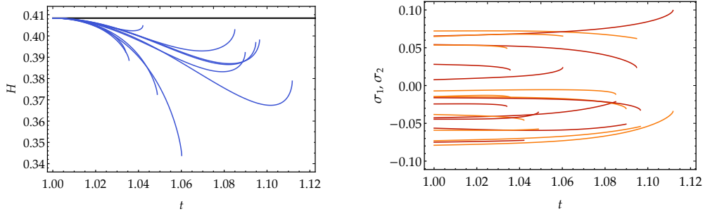
Figure 8.2.2: In the first plot we represent the isotropic solution for H(t) (black line) and the numerical ones (blue lines) starting with the same initial conditions for H , but for randomly generated initial conditions for \sigma_1(t) and \sigma_2(t) . The second plot shows the result of the integration for \sigma_1(t) and \sigma_2(t) . For this numerical result we have chosen \Lambda = 0.5 , M_{\text{Pl}} = 1 , \beta = 0.01 and the initial value H(t = 1) = 0.408362 (the only solution of (8.2.4) compatible with the stability condition that forces \Lambda > 2H^2 [381]).
