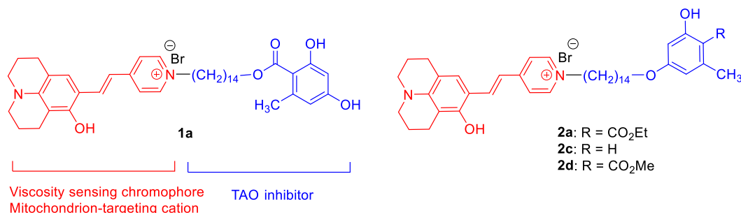
Fig. 1. Structures of fluorescent TAO inhibitor conjugates 1a , 2a , 2c , and 2d bearing a molecular rotor as viscosity sensor (in red) and a TAO inhibitor pharmacophore (in blue).
