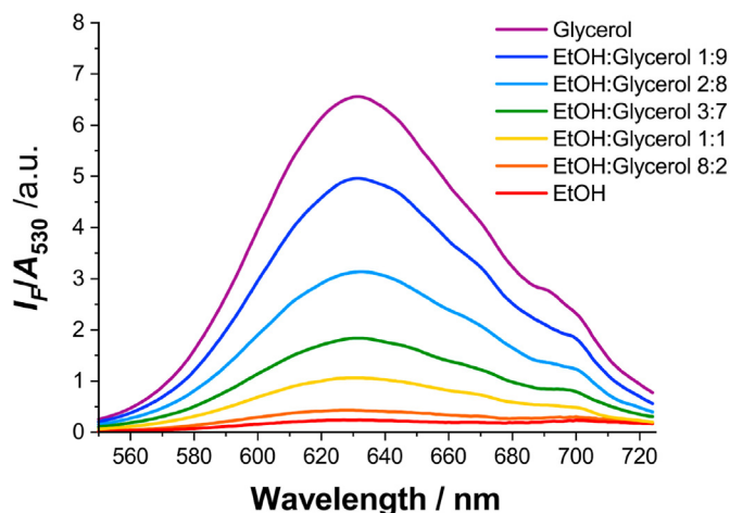
Fig. 2. Emission spectra of 1a (normalized by the absorbance at the excitation wavelength, \lambda_{\text{ex}} = 530 nm) in EtOH:glycerol mixtures.
