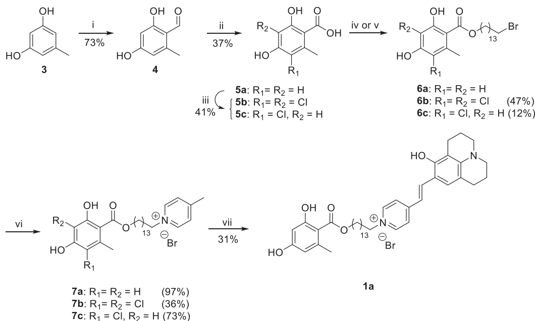
Scheme 1. Synthesis of julolidine derivative 1a and chloro intermediates 7b,c .
