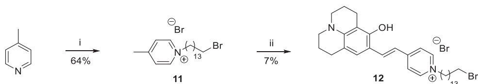
Scheme 3. Synthesis of compound 12 . Reagents and conditions: (i) Br-(CH 2 ) 14 -Br, CH 3 CN, 48 h; (ii) 9-Formyl-8-hydroxyjulolidine, piperidine, 75 °C, 24 h.
