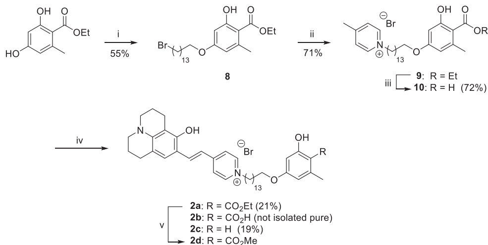
Scheme 2. Synthesis of julolidine derivatives 2a-d . Reagents and conditions: (i) DIAD, PPh 3 , HO-(CH 2 ) 14 -Br, THF, r.t., 18 h; (ii) 4-methylpyridine, CH 3 CN, 80 °C, 3 days; (iii) 1) 3.5 M KOH, H 2 O/MeOH (2/1), 50 °C, 48 h, 2) 3.5 M HCl; (iv) 9-formyl-8-hydroxyjulolidine, pyridine, 75 °C, 24 h; (v) KOH, H 2 O/MeOH, r.t., 24 h.
