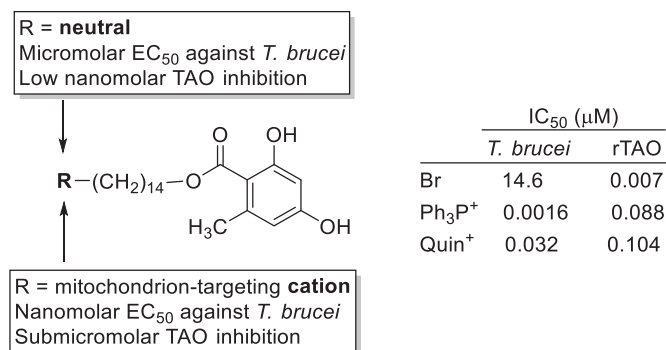
Chart 1. Example of previous 2,4-dihydroxybenzoate-based TAO inhibitors [8,10]. Ph 3 P + : triphenylphosphonium; Quin + : quinolin-1-ium; rTAO: recombinant TAO enzyme.
