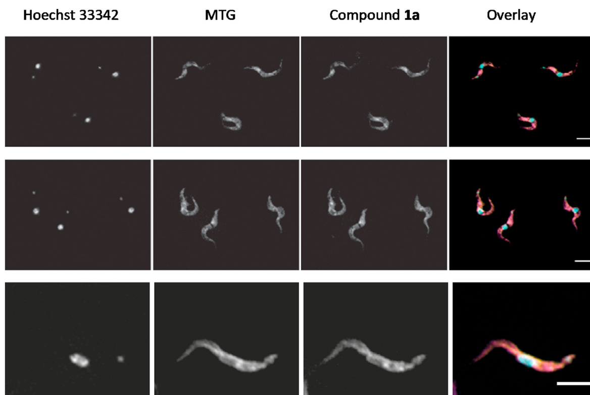
Fig. 8. Mitochondrial localization of 1a in T. brucei . The first column is Hoechst 33342 (stains DNA), the second Mitotracker Green, third compound 1a and the last one the overlay (Hoechst in cyan, Mitotracker in yellow and 1a (40 \mu M, 1 h) in magenta). All scale bars indicate 5 \mu m.
