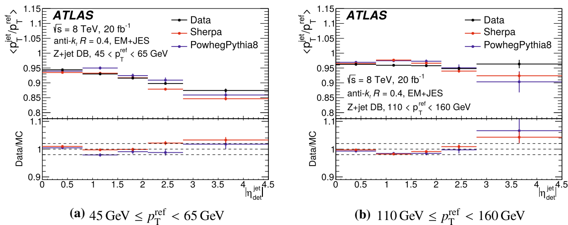
Fig. 23 R_{DB} as a function of \eta_{\text{det}} for anti- k_r jets with R = 0.4 calibrated with the EM + JES scheme in data (black), as well as in SHERPA (red) and POWHEG + PYTHIA8 (blue) simulation, for a 45 \text{ GeV} \leq p_T^{\text{ref}} < 65 \text{ GeV} and b 110 \text{ GeV} \leq p_T^{\text{ref}} < 160 \text{ GeV} . Only statistical uncertainties are shown
