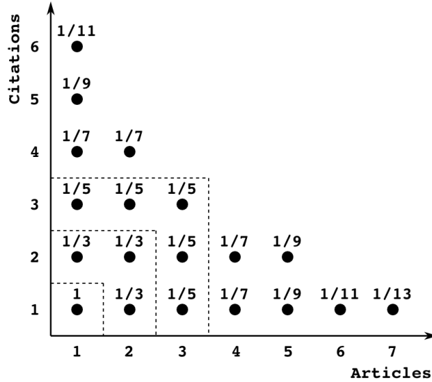
Figure 3: Example of a Ferrers diagram of an author’s citations
