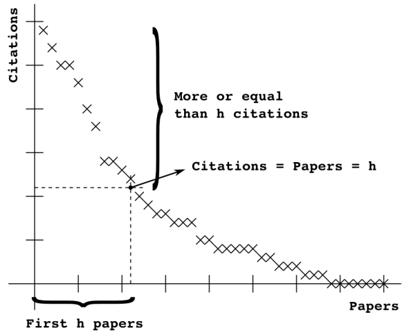
Figure 1: Graphical interpretation of the h-index
