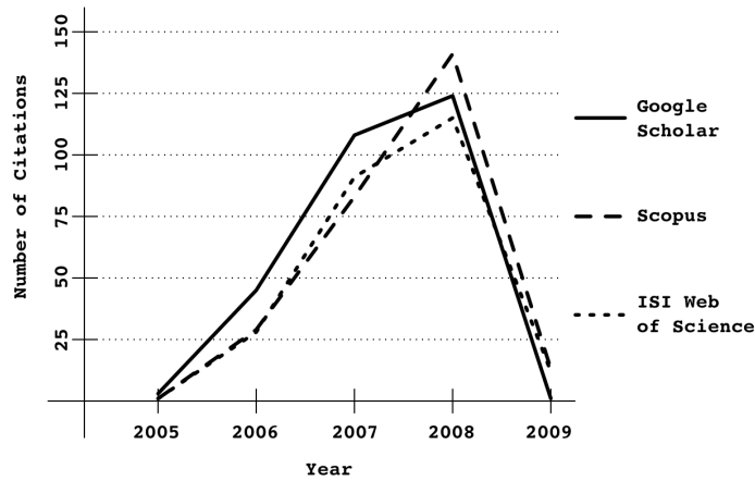
Figure 2: Number of citations received by the original h-index paper (Hirsch (2005)) according to 3 different citation databases (citations until February 16, 2009)
