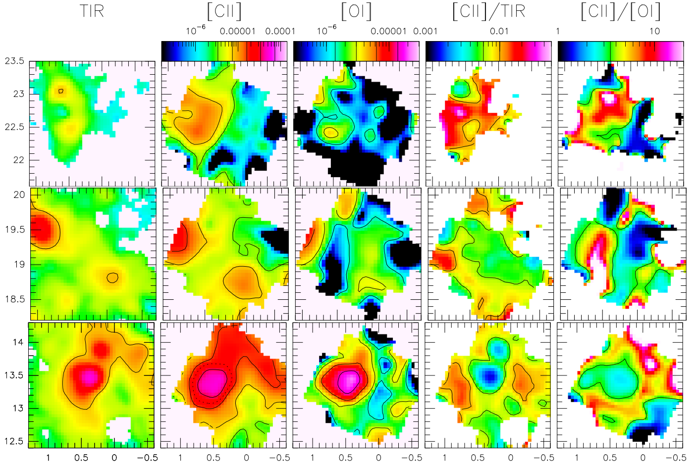
Fig. 3. Three northern most regions of M33 covered with PACS. Top row: northernmost region. Middle row: northern region. Bottom row: BCLMP 691. From left to right: intensities of total infrared continuum (TIR), [C II], [O I](63 \mu\text{m} ), [C II]/TIR, and [C II]/[O I] intensity ratios. Intensities are in units of \text{erg s}^{-1} \text{cm}^{-2} \text{sr}^{-1} . Offsets are in arcminutes relative to the nucleus, the same as in Fig. 2. The TIR color wedge is the same as in Fig. 1. Contours of TIR, [C II], [O I], [C II]/TIR, and [C II]/[O I] are the same as in Fig. 2. The dashed [C II] contour for BCLMP 691 corresponds to a constant intensity of 22.4 \times 10^{-6} \text{erg s}^{-1} \text{cm}^{-2} \text{sr}^{-1} derived from the best-fitting y -intercept in the correlation plot of \log[\text{C II}]/\text{TIR} vs. \log\text{TIR} , for a slope of -1 (Fig. 9).
