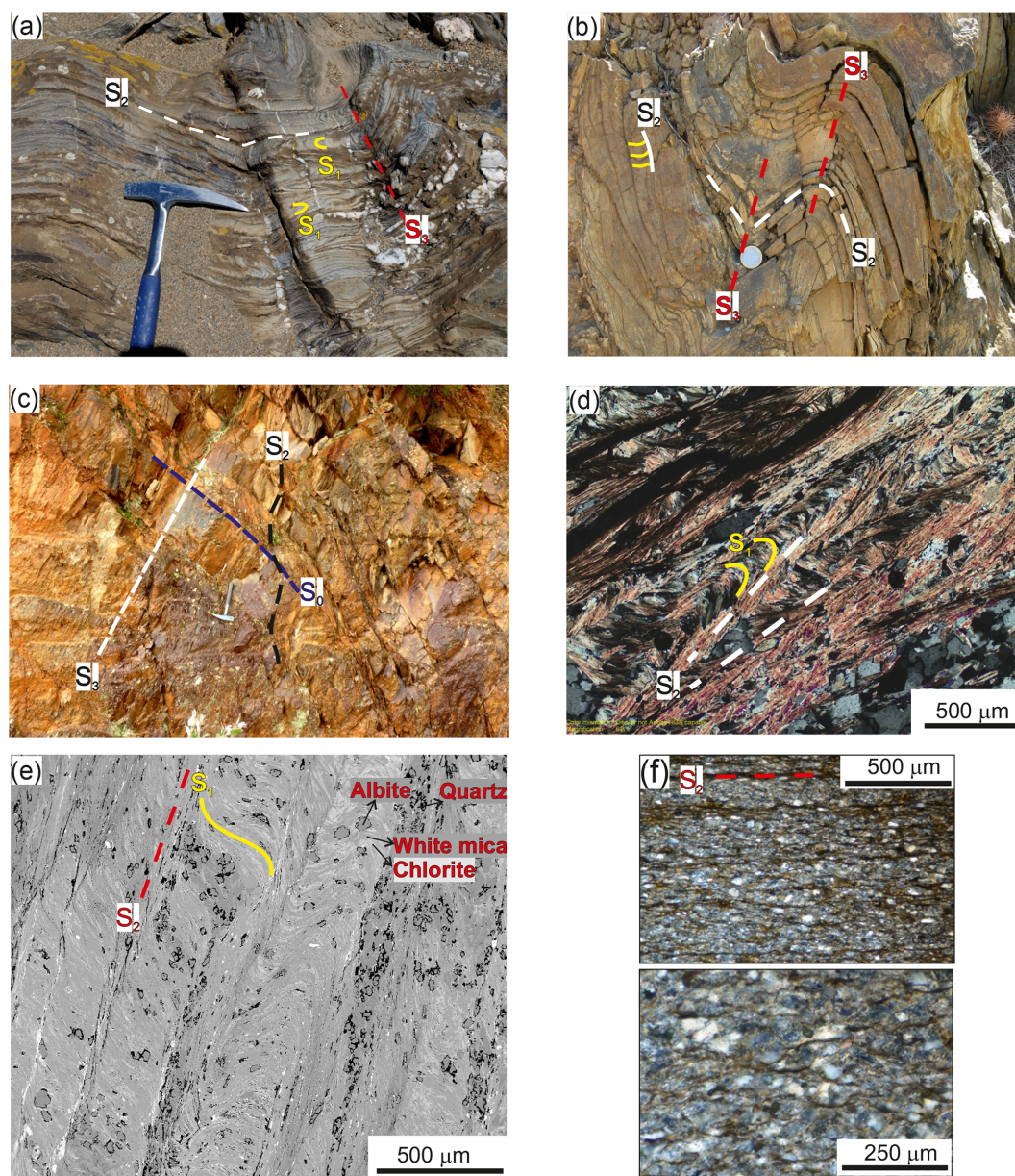
Figure 2. Pictures of the Pulo do Lobo rocks illustrating deformation at the outcrop scale: (a) Pulo do Lobo Formation, (b) Ribeira de Limas Formation, (c) Santa Iria Formation. Microphotographs from thin sections: (d) cross-polarized light image of sample PLB-84 (Pulo do Lobo Formation), (e) SEM-BSE (backscattered electron) image of sample PLB-88 (Ribeira de Limas Formation), (f) cross-polarized light images of sample PLB-71 (Santa Iria Formation).
