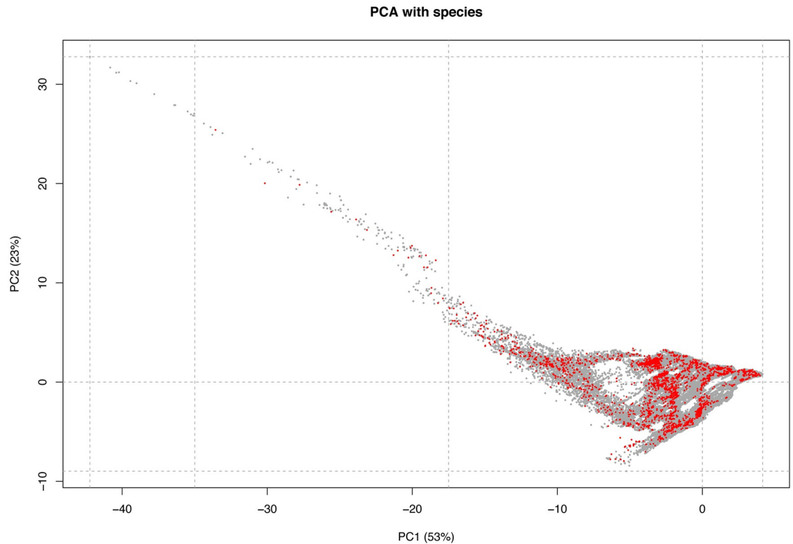
Fig 4. Principal component analysis (PCA) of the climatic space of the UAE (grey dots) using 19 bioclimatic variables from WORLDCLIM. Red dots represent the distribution of the 5,535 occurrence records of all 60 species of terrestrial reptiles of the UAE in this climatic space. Dashed lines delimit climatic clusters that group 20% of the explained variance of PC1 and PC2.
