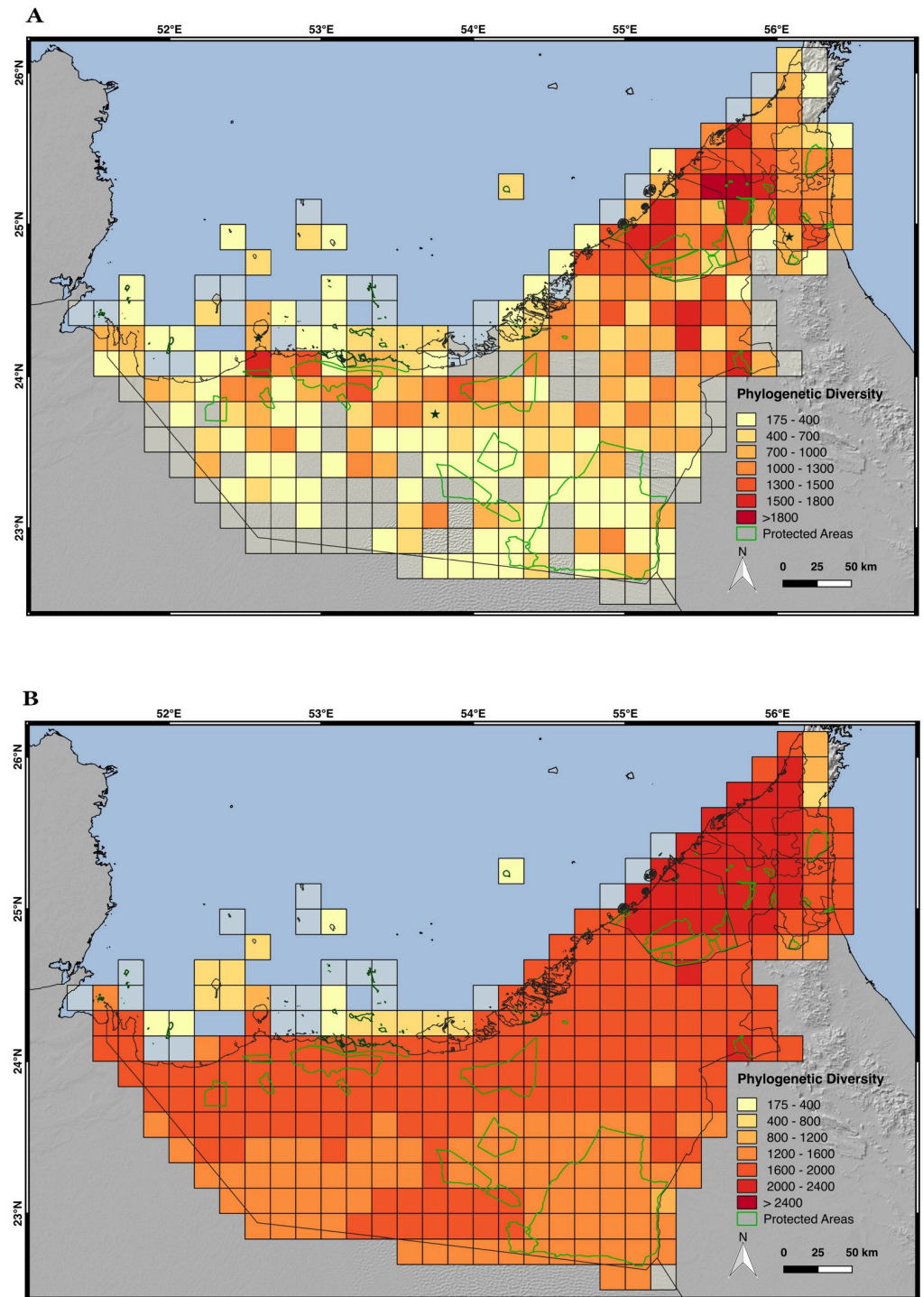
Fig 10. Maps of phylogenetic diversity (PD). A) PD by grid cells of 10 arc-minutes of longitude and latitude, using the area of occupancy of each species calculated with the occurrence point data; B) PD by grid cells of 10 arc-minutes of latitude and longitude inferred with the species distribution models; the terrestrial protected areas of the UAE are shown in light green; black stars represent the cells with values of PD significantly different than the expected by random. Only the 57 native species have been included in the analyses. Credits: OpenStreetMap contributors, SRTM.
