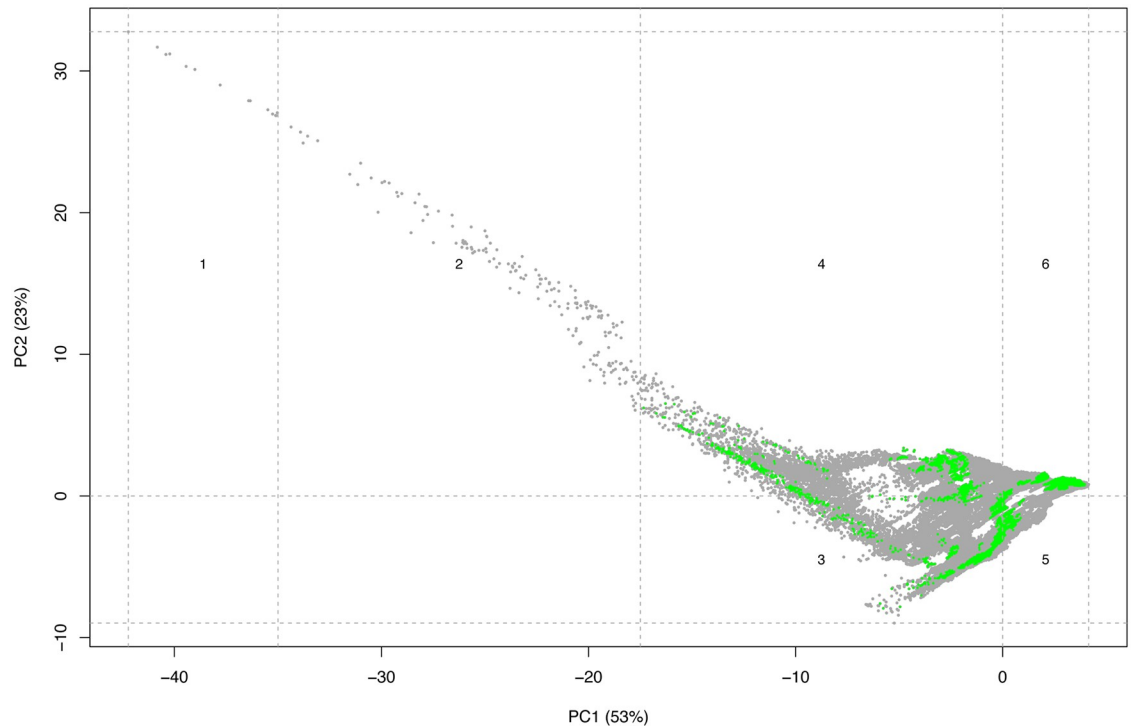
Fig 8. Principal component analysis (PCA) of the climatic space of the UAE (grey dots) using 19 bioclimatic variables from BIOCLIM. Dashed lines delimit climatic clusters that group 20% of the explained variance of PC1 and PC2. Green dots represent the climatic space occupied by the protected areas.
