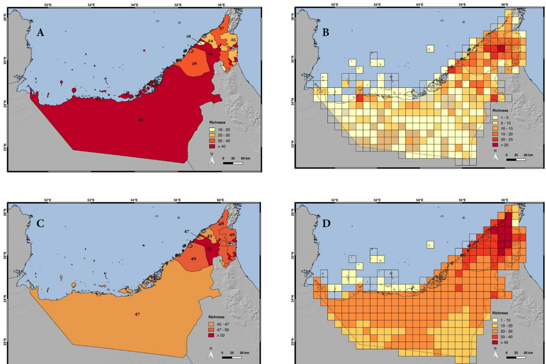
Fig 6. Species richness map of the UAE terrestrial reptiles. A) Species richness by emirate inferred with the occurrence point data; B) Species richness by 10 arc-minutes grid cells inferred with the occurrence point data; C) Species richness by emirate inferred with the species distribution models; D) Species richness by 10 arc-minutes grid cells inferred with the species distribution models. Only the 57 native species have been included in the analyses. Credits: OpenStreetMap contributors, SRTM.
