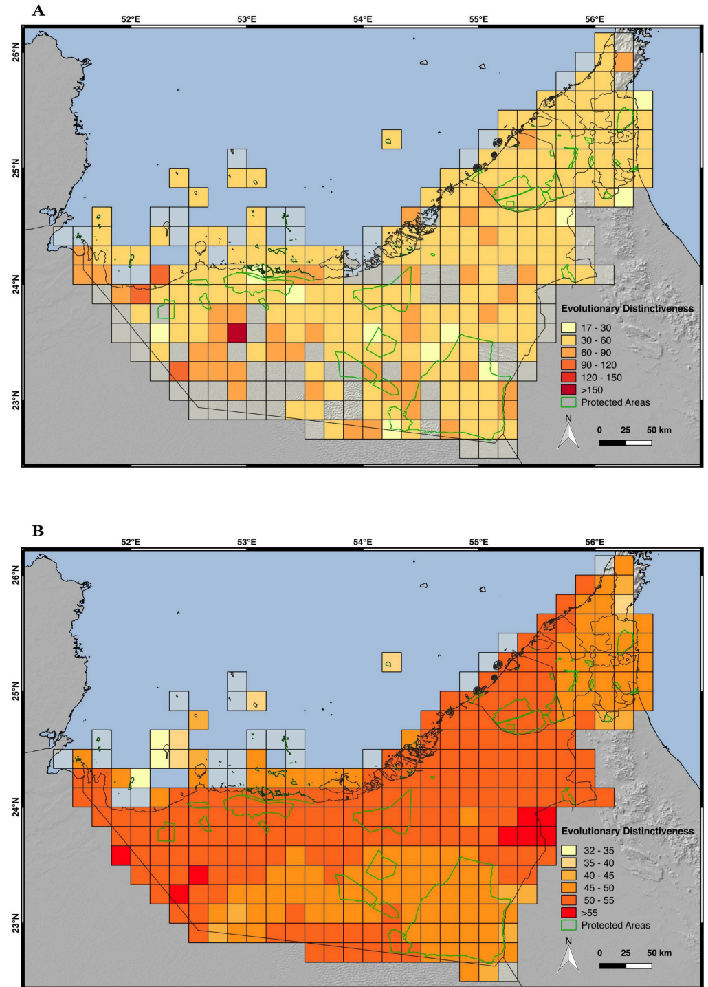
Fig 11. Maps of evolutionary distinctiveness (ED). A) ED by grid cells of 10 arc-minutes of longitude and latitude, using the area of occupancy of each species calculated with the occurrence point data; B) ED by grid cells of 10 arc-minutes of latitude and longitude inferred with the species distribution models; the terrestrial protected areas of the UAE are shown in light green. Only the 57 native species have been included in the analyses. Credits: OpenStreetMap contributors, SRTM.
