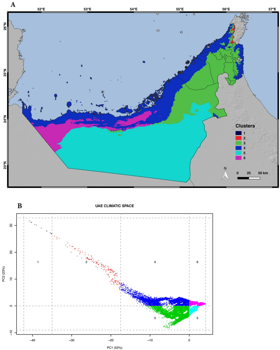
Fig 5. Climatic variability of the UAE. A) Map showing the distribution and extension of the six UAE climatic clusters; B) Principal component analysis (PCA) of the climatic space of the UAE (grey dots) using 19 bioclimatic variables from BIOCLIM with the climatic clusters numbered from one to six and colored with the same colors as in the map. Credits: OpenStreetMap contributors, SRTM.
