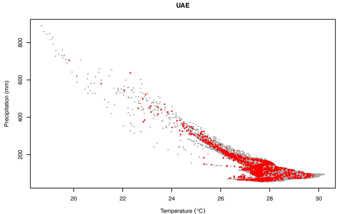
Fig 3. Two-dimensional climatic space of the UAE (grey dots) defined by the annual mean temperature (BIO1) and annual mean precipitation (BIO12). Red dots represent the distribution of the 5,535 occurrence records of all 60 species of terrestrial reptiles of the UAE.
