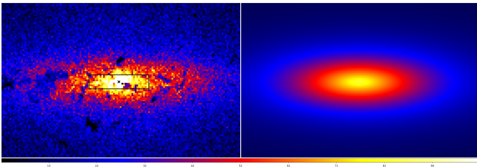
Figure 3.7: Map of the stellar density in the central 341 pc x 219 pc of our Galaxy. Both panels use the same color linear scales. Left: stellar number density map from Nishiyama et al. (2013). The black rectangle indicates the FOV of our data ( \sim 86 pc \times 20.2 pc). Sgr A* is located in the position of the black cross. Right: Sérsic plus triaxial ellipsoidal fit to the data after masking the central 10 pc occupied by the NSC and regions with low density.
