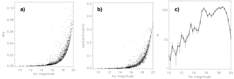
Figure E.3: Results obtained applying method 1 to AO data. a) Photometric uncertainties versus K_s magnitude from Starfinder program. b) Astrometric uncertainties versus K_s magnitude from Starfinder program. We represent \sqrt{dx^2 + dy^2} versus K_s , where dx and dy are the errors in the x-position and y-position, respectively, of each star. c) KLF for the deep image.
