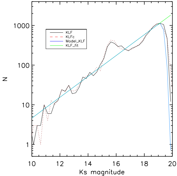
Figure 4.3: The Ks LF in pointing 1 for min\_correlation=0.8 and deblend=0 if shown as a black line. The dotted red line is the K_s LF after correcting the magnitude of each star for differential extinction. The green lines shows a power law fit to the bright stars 11 < K_s < 14.5 with power law index of 0.26 \pm 0.02 . The blue line shows the effect of the completeness function according to equation (2) in Chatzopoulos et al. (2015b) .
