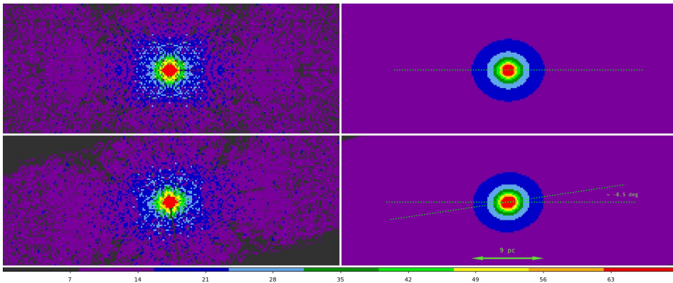
Figure 3.13: Zoom-in to compare the symmetrized images of the inner \sim 42 pc x 16 pc of the Galaxy for stars with 12.5 \leq K_{s,extc} \leq 14.0 obtained by keeping the angle between the NSC and GP equal to 0 (upper panels, ID 3 in Table A.1) and leaving the tilt angle free in the fits (lower panels, ID 3 in Table A.2). Right panels show the Sérsic model that we obtain from the fits for each case. The color scale is linear and all the images have been scaled in an identical way. Galactic north is up and Galactic east is to the left.
