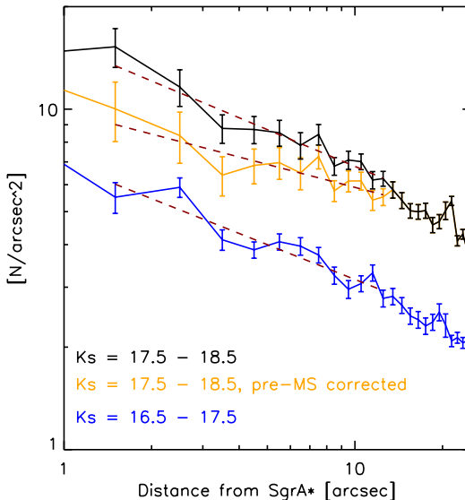
Figure 4.18: Extinction and crowding-corrected surface number density profiles for 16.5 \leq K_s \leq 17.5 (blue line), 17.5 \leq K_s \leq 18.5 (black line), and for 17.5 \leq K_s \leq 18.5 after correction for potentially present pre-MS stars from the most recent star formation event (using parameters from ID 1 in Tab. 4.3). The dashed red lines are simple power-law fits in the range 0.04 (pc) \leq R \leq 0.5 pc .
