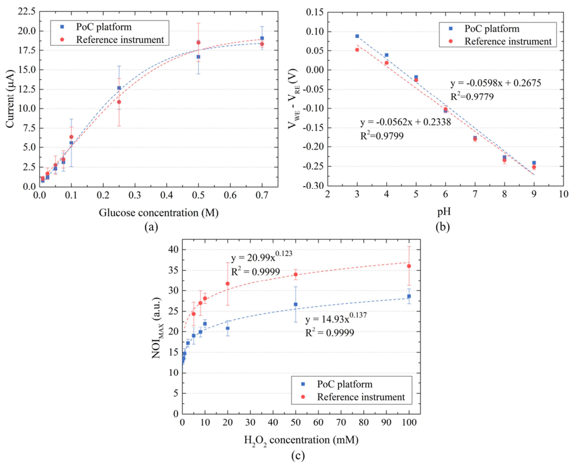
Figure 4. PoC platform applications. Comparison between signals acquired by the described platform and the reference electrochemical instrument for: (a) Determination of glucose by chronoamperometry; (b) pH measurement by potentiometry; and (c) Determination of \text{H}_2\text{O}_2 by ECL.
