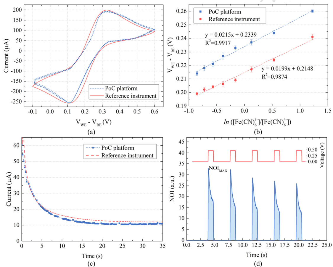
Figure 3. PoC platform validation. Comparison between signals acquired by the described platform and a commercial electrochemical instrument using ferricyanide/ferrocyanide couple for (a) cyclic voltammetry, (b) potentiometry and (c) chronoamperometry. In case of ECL (d), the well-known system luminol – \text{H}_2\text{O}_2 has been used as a model. Graph (d) represents the normalized optical intensity, NOI, obtained from the filtered frames as the sum of the value of all the pixels when 0.5 V pulse voltages are applied. \text{NOI}_{\text{MAX}} is also shown as the maximum at the first voltage pulse.
