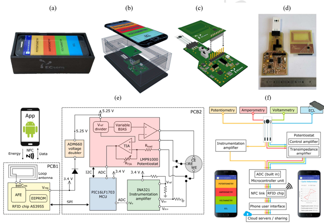
Figure 1. Images and schematic illustrations of the smartphone-based analytical PoC platform. (a) Picture of the complete PoC platform in operative mode showing the black methacrylate holder accessory as the ambient light shielding enclosure to accommodate the PCBs and the NFC-enabled mobile phone running the custom-developed application. (b) Rendered exploded view of the complete PoC platform with a see-through view of the holder accessory to show the positioning and alignment of the PCBs inside it. (c) Rendered 3D detailed view of the designed PCBs for signal processing/transmission and power management. (d) Photograph of the fabricated PCBs with the SPE attached. (e) Schematic, power and data flow of the PCBs for power management (PCB1) and signals processing/transmission (PCB2) showing all the components involved in the operation. (f) System-level block diagram of the PoC platform showing the signal transduction, conditioning, processing and wireless transmission paths from the electrode to the custom-developed mobile application for amperometry, potentiometry, cyclic voltammetry and electrochemiluminescence techniques. The inset images show the home page (left) and the real-time data display page for cyclic voltammetry (right) of the mobile application.
