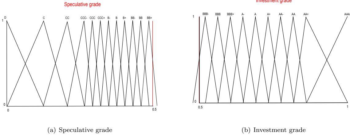
Figure 4: Linguistic term sets grouped by main categories
