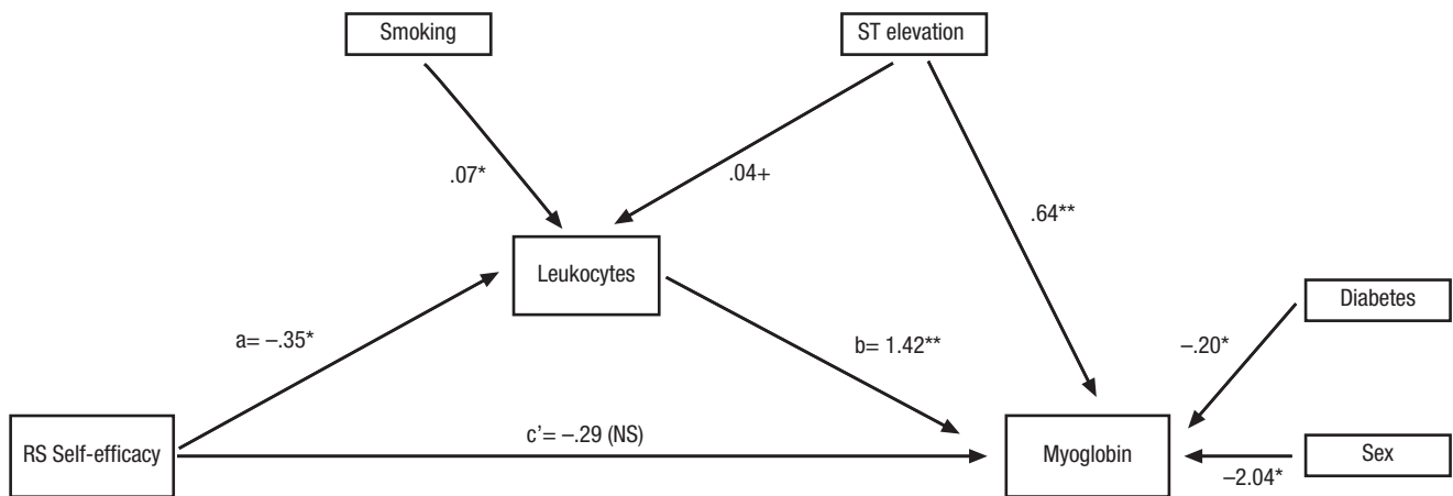
Figure 2 Path scheme of the effect of RS self-efficacy on myoglobin and the mediator effect of leukocytes. In the analyses, we controlled for the effect of ST elevation and classical risk factors. Only significant and almost significant factors were displayed. Note: Estimated coefficients are shown.
