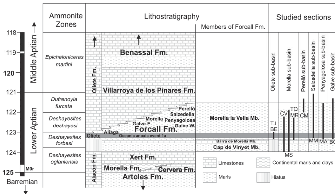
FIGURE 2 | Stratigraphic framework and age relationships of the Aptian deposits in the Maestrat Basin. Position of OAE 1a is indicated by shaded level (after Moreno-Bedmar et al., 2008, 2009). Oi: Oliete sub-basin; Al: Aliaga sub-basin; Ga: Galve sub-basin; E: East; W: West; Mo: Morella sub-basin; Pe: Perelló sub-basin; Sa: Salzedella sub-basin, and Pg: Penyalgosa sub-basin. Stratigraphic positions of the ten sections studied of the Forcall Formation relative to ammonoid biozones. MA: Mas Agustina section; MM: Mola Murada section; BC: Barranco de las Calzadas section; CV: Cap de Vinyet section; TO: Todolella section; MR: Mas del Roc section; MS: Mas Segura section; CM: Cala dels Moros section; TJ: Tejería de Josa section and BE: Barranco Emilia section. Absolute ages after Gradstein et al. (2004).
