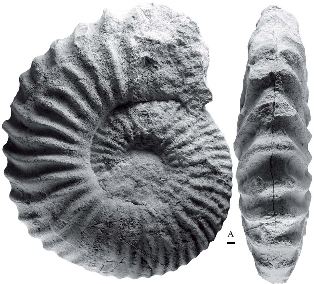
FIGURE IX | A) Dufrenoyia furcata specimen DT-1, Noguerauelas. Scale bar, 1cm.
