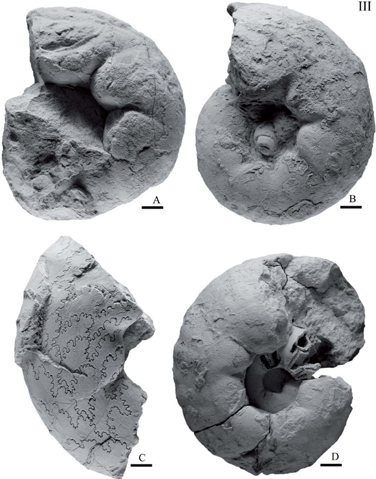
FIGURE III | A) Roloboceras hispanicum , specimen CPT-3234, Barranco de las Calzadas section, sample BCGa-3. B) Roloboceras hispanicum , specimen RA-1 (Ramiro Álvarez, Barcelona, Particular collection), Tejería de Josa section, equivalent to sample TJOI-1. C) Roloboceras hispanicum , specimen CPT-3788, Tejería de Josa section, sample TJOI-1. D) Roloboceras hispanicum , specimen RM-2 (Ramon Margalef, Barcelona particular collection), Tejería de Josa section, equivalent to sample TJOI-1. Scale bar, 1 cm.
