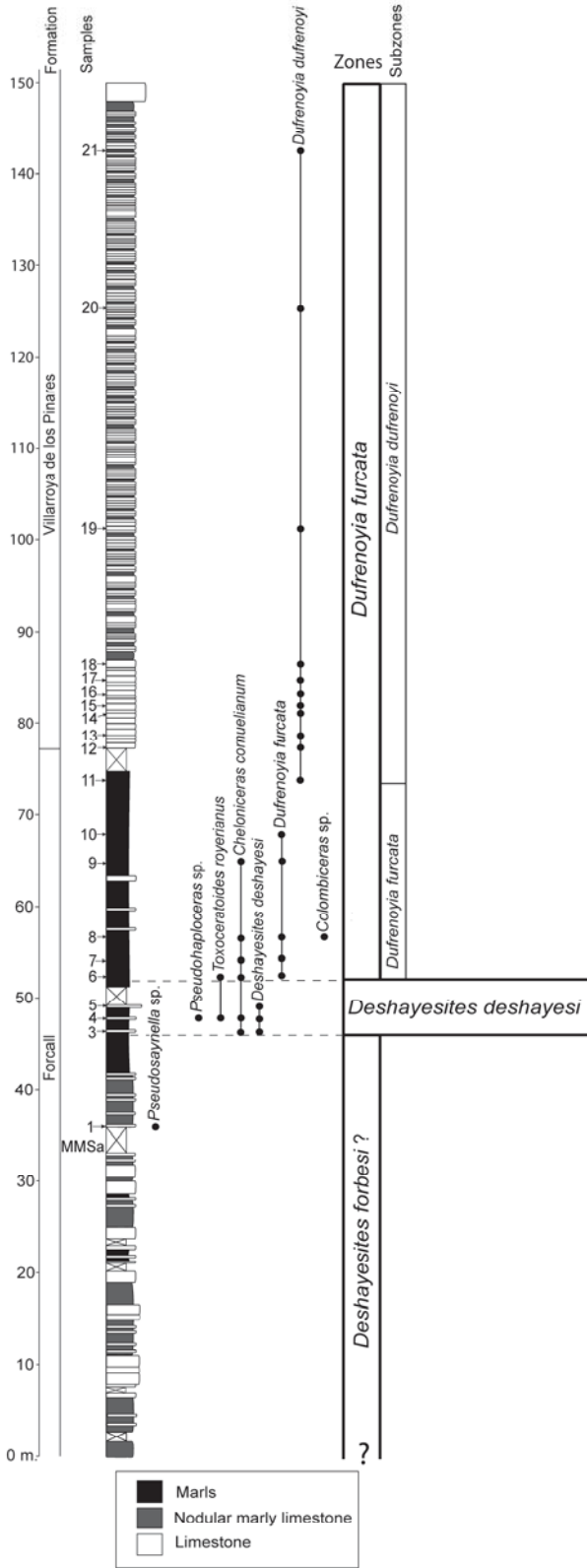
FIGURE 7 | Saizadella sub-basin, Mola Murada section.
