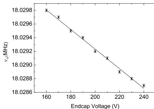
Figure 5: Modified cyclotron frequency ( \nu_+ ) for \text{He}^+ ions as a function of the voltage applied to the endcap electrodes. A relative uncertainty of 10^{-6} due to magnetic field inhomogeneities was added to the modified cyclotron frequencies.
