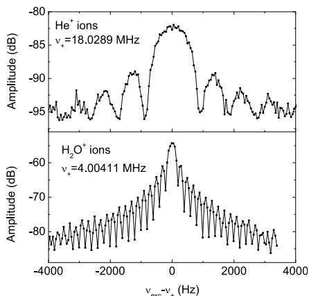
Figure 4: Top: amplitude of the FT-ICR signal versus excitation frequency ( \nu_{\text{exc}} ) for \text{He}^+ ions ( \Delta\nu_{\text{FWHM}} = 1095 Hz). Bottom: amplitude of the FT-ICR signal versus excitation frequency for \text{H}_2\text{O}^+ ions ( \Delta\nu_{\text{FWHM}} = 276 Hz). \nu_+ is the modified cyclotron frequency. For details see text.
