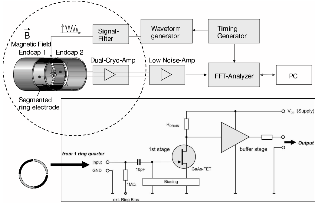
Figure 2: Schematic view of the three-electrode cylindrical Penning trap system to be placed in the transport section of the KATRIN beam line. The dashed circle houses all the components: Penning trap, cryogenic preamplifier and signal filter, located in vacuum in the high-magnetic field region of a superconducting magnet. The waveform generator used for excitation provides also the trigger for data acquisition with the FFT analyzer. The square box shows a simplified version of the electronic circuit for one channel of the Dual-Cryo-Amplifier.
