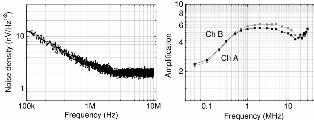
Figure 3: Noise level and amplification factor versus frequency of the amplifier designed to be operated at cryogenic temperatures in the KATRIN beamline. The noise level was measured at T = 300 K and is expected to be reduced by a factor of \approx 1.5 at T = 50 K. For the determination of the amplification factor, the signals from the two quarters of the ring were fed into the measuring device through different channels (ChA and ChB).
