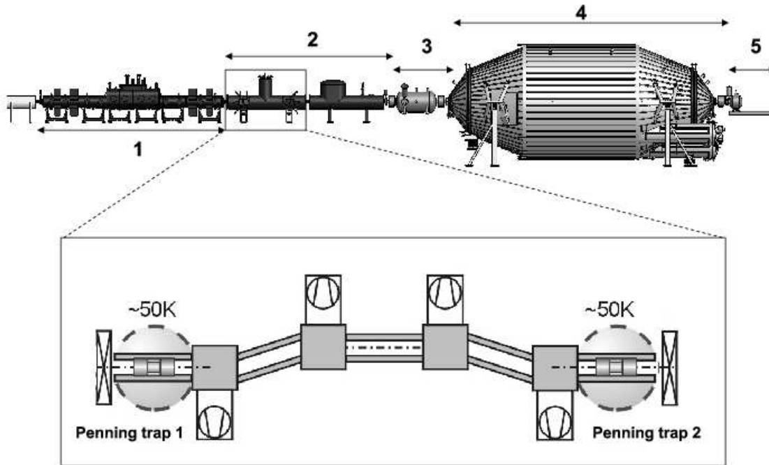
Figure 1: Sketch of the KATRIN beam line indicating the main components: 1) windowless gaseous tritium source, 2) transport section, 3) pre-spectrometer, 4) main spectrometer, and 5) detector. The total length of the KATRIN beam line is 70 m. In the first part of the transport section (enlarged at the bottom) the concentration of unwanted ions due to the formation of clusters will be monitored employing Penning traps using the Fourier-Transform Ion-Cyclotron-Resonance (FT-ICR) detection technique. The traps will be operated at cryogenic temperatures in a magnetic field of 5.6 T.
