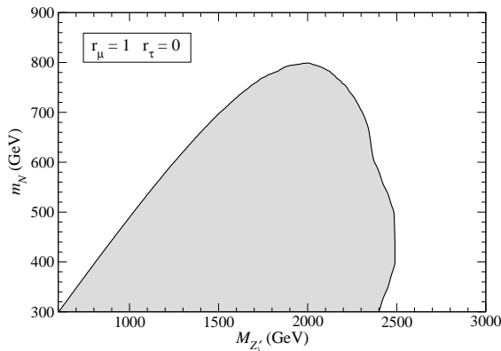
Figure 8: 5\sigma discovery limit for pp \rightarrow Z'_\lambda \rightarrow NN giving \mu^\pm \mu^\pm X final states at LHC, for a luminosity of 30 \text{ fb}^{-1} . Heavy neutrinos are assumed to couple only to the muon.
