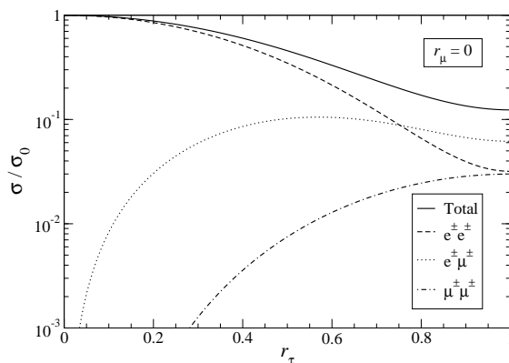
Figure 3: Ratio \sigma/\sigma_0 between the dilepton cross section to electron and muon final states and the total one in Fig. 2. The parameters r_\mu , r_\tau are defined in Eq. (5).
