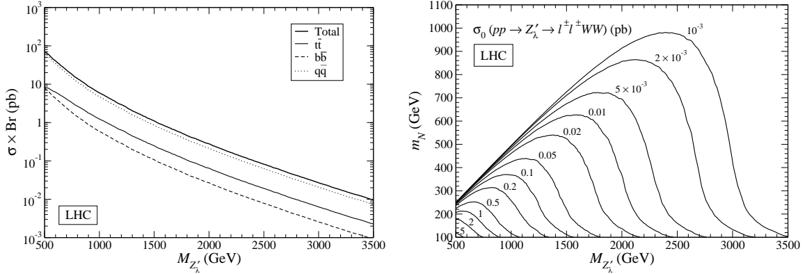
Figure 7: Left: Total cross section for Z'_\lambda production at LHC, and cross sections for several SM final states. Right: Total cross section for \ell^\pm \ell^\pm W^\mp W^\mp production at LHC, summing final states with any combination of \ell = e, \mu, \tau .
