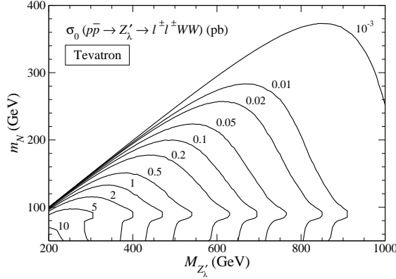
Figure 2: Total cross section for \ell^\pm \ell^\pm W^\mp W^\mp production at Tevatron, summing final states with any combination of \ell = e, \mu, \tau .
