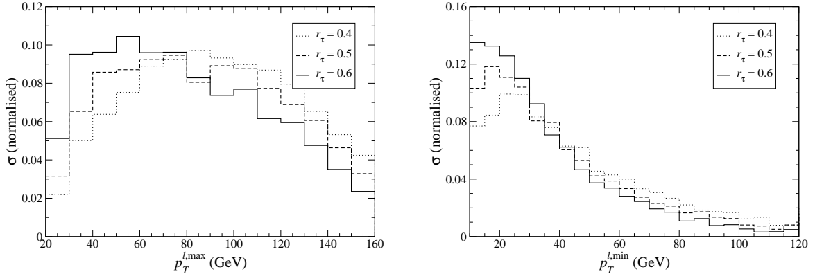
Figure 4: Transverse momenta of the leading ( p_T^{\ell,\max} ) and sub-leading ( p_T^{\ell,\min} ) charged leptons.
