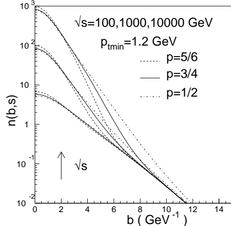
Figure 7: The average number of collisions for the singular \alpha_s case for different values of the singularity parameter p .
