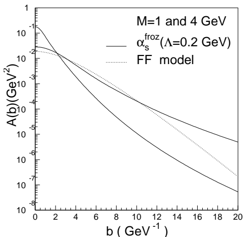
Figure 4: The overlap function A_{BN}(b) for frozen \alpha_s and comparison with the Form Factor model
