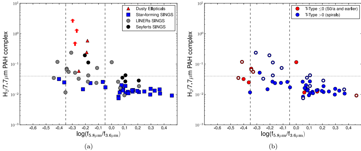
FIG. 16.— a) The Kaneda et al. (2008) dusty ellipticals (red) and SINGS H_2 -detected galaxies are plotted as a function of \log[f_{5.8\mu\text{m}}/f_{3.6\mu\text{m}}] color, where the vertical dashed lines indicate the mid-infrared green valley (from Equation 1). SINGS star-forming systems are shown in blue (squares), LINER systems are grey (circles) and Seyferts are in black (circles). b) The SINGS sample is plotted in terms of T-type (late-type in blue, early type in red), with open circles indicating galaxies in dense/interacting environments.
