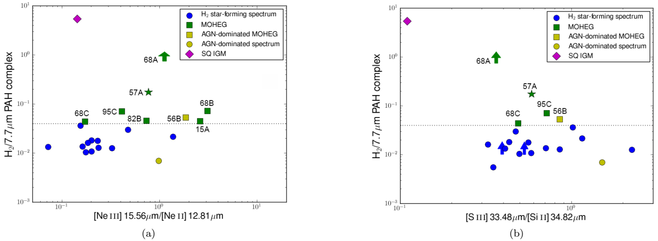
FIG. 13.— a) \text{H}_2/7.7\mu\text{m} PAH plotted as a function of [\text{Ne III}] 15.56\mu\text{m}/[\text{Ne II}] 12.81\mu\text{m} with the same color-coding as Figures 10 and 11a. The off-nuclear extraction of HCG 57A is shown as a star. b) \text{H}_2/7.7\mu\text{m} PAH plotted as a function of [\text{S III}] 33.48\mu\text{m}/[\text{Si II}] 34.82\mu\text{m} with the same color designation as on the left.
