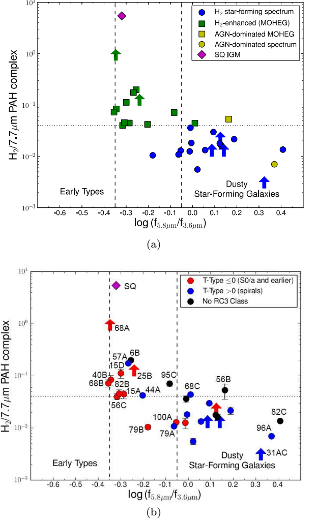
FIG. 11.— a) H 2 /7.7 \mu m PAH ratio as a function of IRAC color ( f_{5.8\mu m}/f_{3.6\mu m} ) with the same symbols as in Figure 10. Lower limits are shown as arrows and the location of the IGM shock in SQ is plotted as a magenta diamond. The dashed lines indicate intermediate mid-infrared colours (determined in Section 2) and the dotted horizontal line indicates MOHEG H 2 -enhancement (Ogle et al. 2010). b) H 2 /7.7 \mu m PAH ratio as a function of [f_{5.8\mu m}/f_{3.6\mu m}] color color-coded according to T-Type. Error bars from the combined line measurements are indicated, although for several systems they are comparable to the size of the marker.
