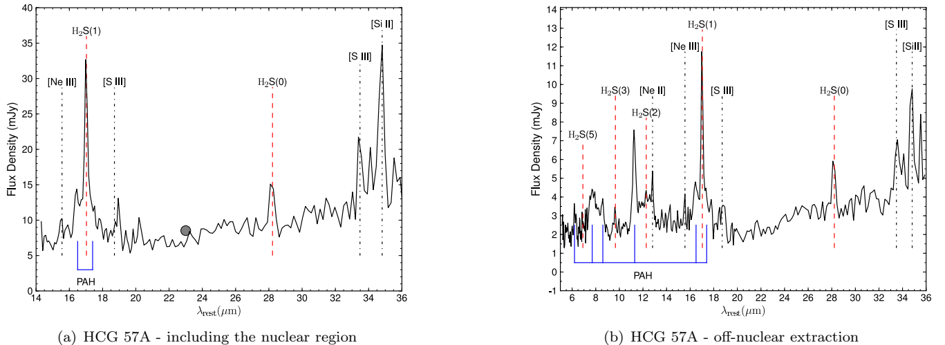
FIG. 5.— Spectra of HCG 57A. The matched MIPS 24 \mu m photometry is shown as a filled grey circle.
