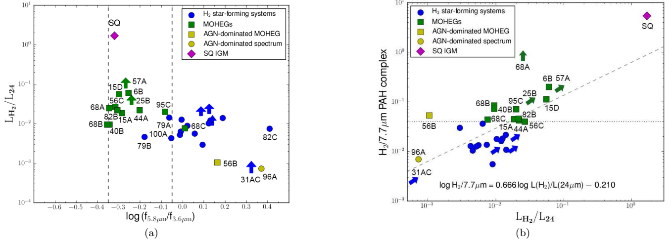
FIG. 12.— a) L_{\text{H}_2} S(0)-S(3)/L_{24} luminosity ratio for \text{H}_2 -detected systems as a function of \log[f_{5.8}/f_{3.6}] color with the same symbols as in Figures 10 and 11a. Arrows represent systems where the \text{H}_2 luminosity is a lower limit and the vertical dashed lines are from Equation 1. The diamond shows the location of the shocked IGM of SQ (from Cluver et al. 2010). b) \text{H}_2/7.7\mu\text{m} PAH ratio as a function of L_{\text{H}_2} S(0)-S(3)/L_{24} with the same color-coding as on the left. The dotted line indicates MOHEG \text{H}_2 -enhancement (Ogle et al. 2010). Arrows indicate systems with lower limits for their \text{H}_2 fluxes (due to not having the full SL+LL coverage) and are not included in the least-squares fit (grey dashed line); the best-fit relation is given at the bottom of the figure.
