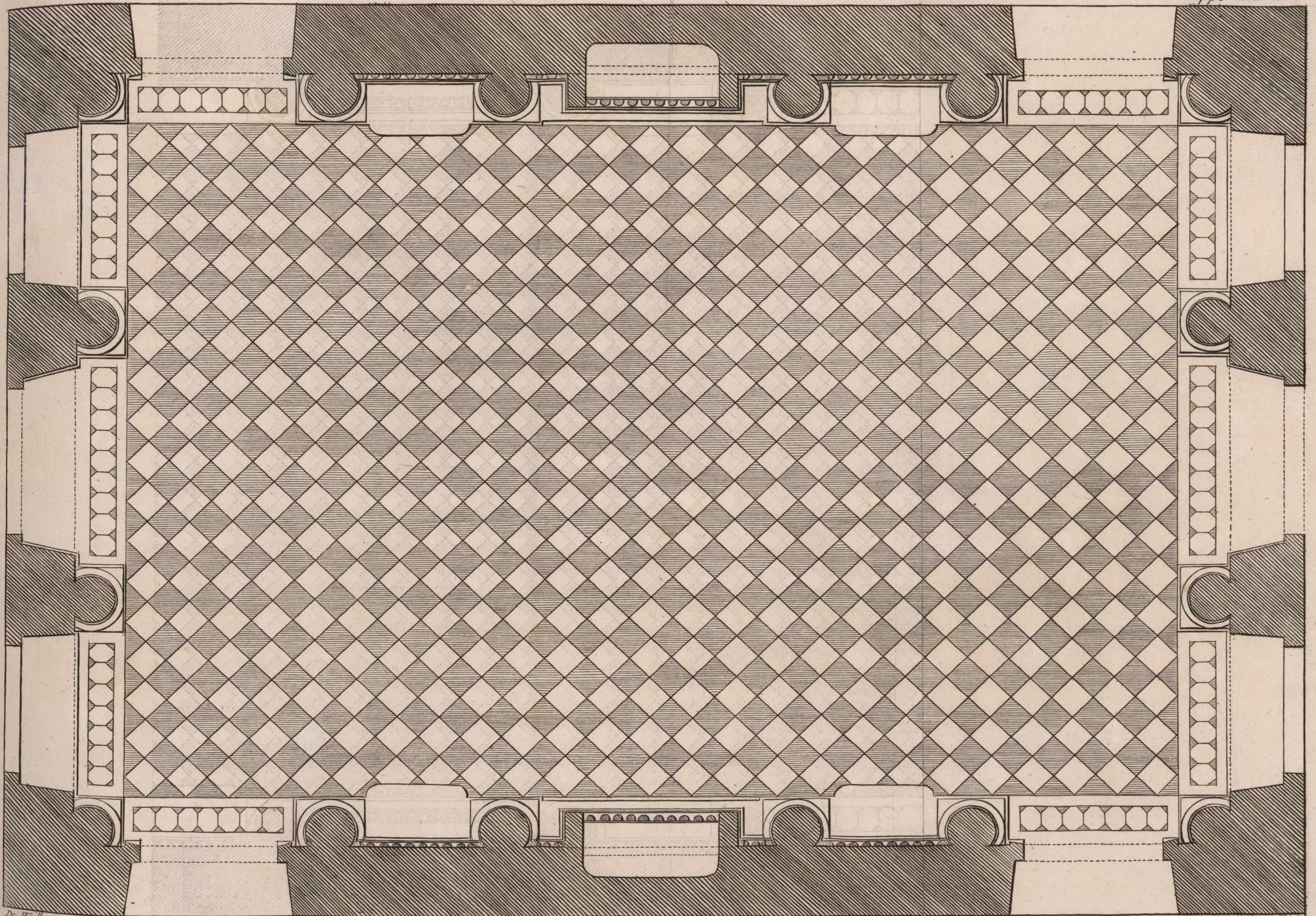
Architecture. Sallon. Plan.
