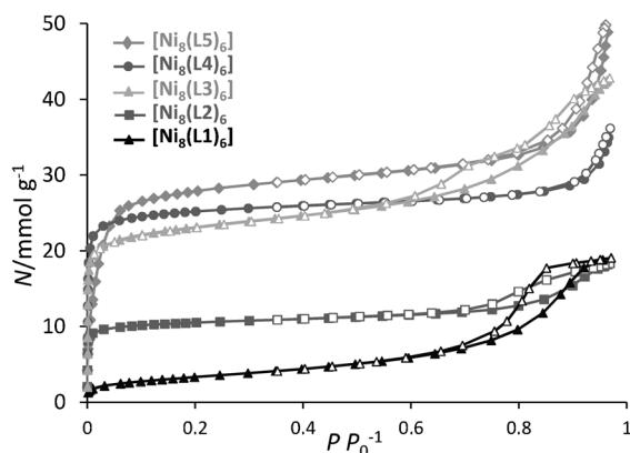
Figure 2. \text{N}_2 physisorption isotherms (77 K) for the isoreticular [\text{Ni}_8(\text{L})_6] series. Solid symbols denote adsorption, open symbols desorption ( P/P_0 = partial pressure).
