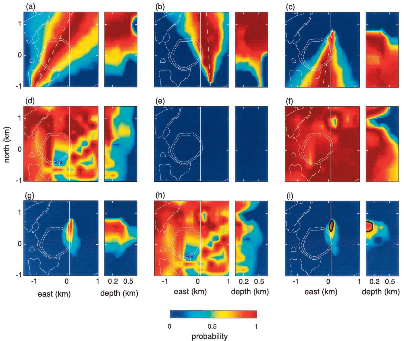
Plate 3. Spatial probability distributions used in the source location procedure for one LP event (same event as in Plate 1) using the synthetic slowness vector model. Each panel pair shows (left) a horizontal slice through a probability distribution at 40 m depth in the slowness model and (right) a north-south vertical cross section, whose position is marked by the white line in the map view. (a,b,c) Probability distributions for azimuths obtained at arrays D, E, and F, respectively. The white dashed lines show the average geometric back azimuths of the waves detected by each antenna. (d,e,f) Probability distributions for slownesses obtained at arrays D, E, and F, respectively. The probability distribution for slowness obtained at the E antenna (Plate 3e) is not used (see text for explanations). (g) Combined probability for azimuth, the product of Plates 3a, 3b, and 3c. (h) Combined probability for slowness, the product of Plates 3d and 3f. (i) Spatial source probability, including both azimuth and slowness information. The bold black lines are contours of the surface at 80% of the maximum probability. We take these contours as a measure of the error of the solution.
