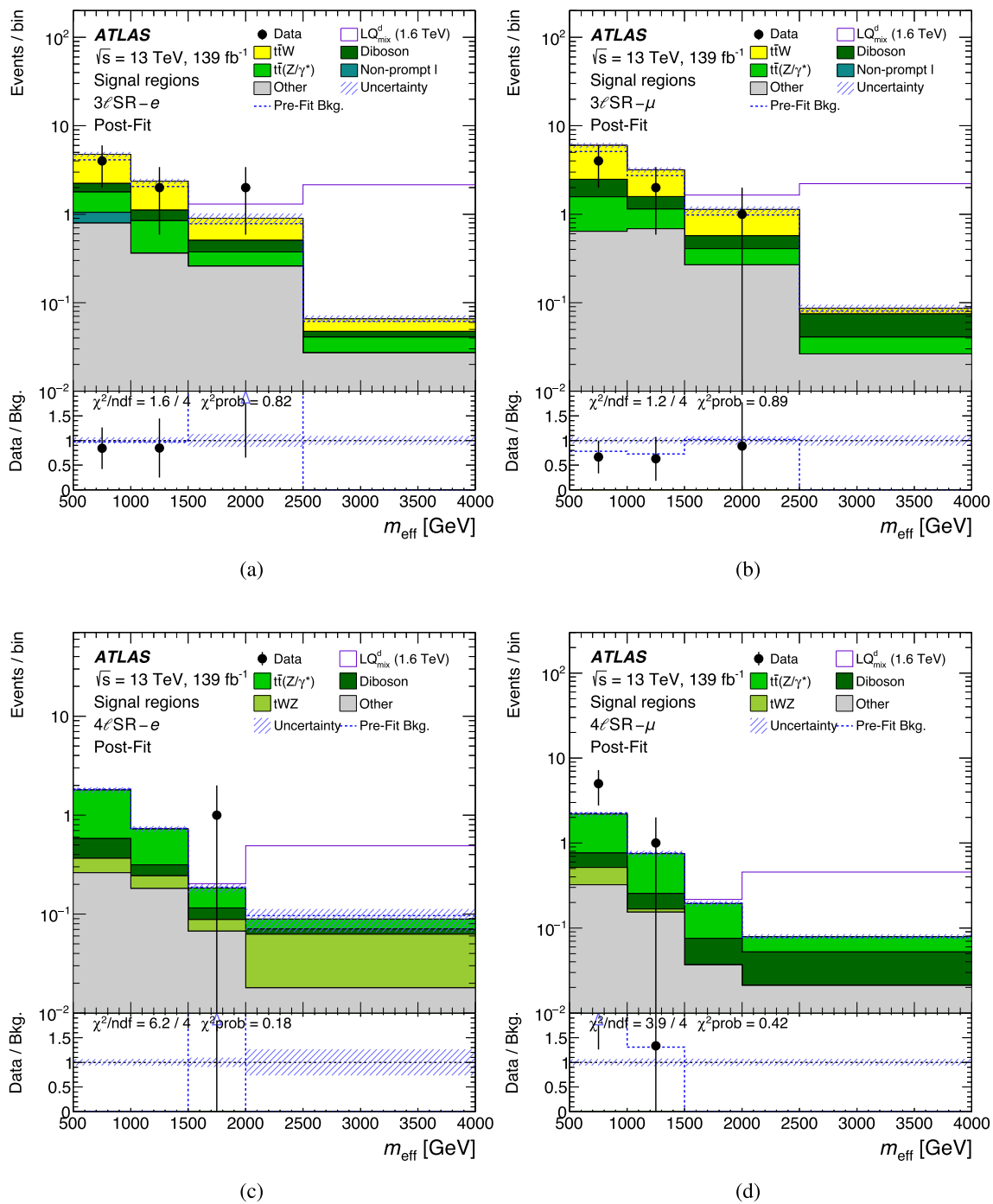
Fig. 7 Comparison between data and prediction for the m_{\text{eff}} distribution used in different signal region categories: a 3ℓSR – e, b 3ℓSR – μ, c 4ℓSR – e, and d 4ℓSR – μ. The background contributions after the likelihood fit to data (“Post-Fit”) under the background-only hypothesis are shown as filled histograms. The total background prediction before the likelihood fit to data (“Pre-Fit Bkg.”) is shown as a dashed blue histogram in the upper panel. The ratio of the data to the background (“Bkg.”) prediction is shown in the lower panel, separately for post-fit
