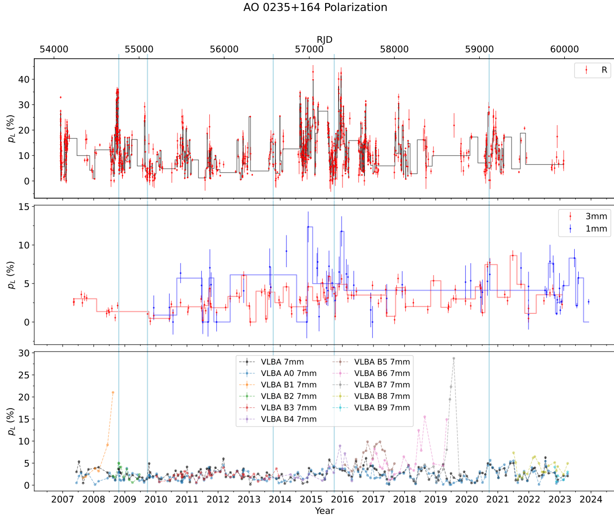
Fig. 3. Historical evolution of the polarization degree of AO 0235+164. A Bayesian block representation is shown superimposed for R at 99.9% confidence and for 1mm and 3mm at 90% confidence. Vertical lines corresponds to the dates marked in Fig. 1.
