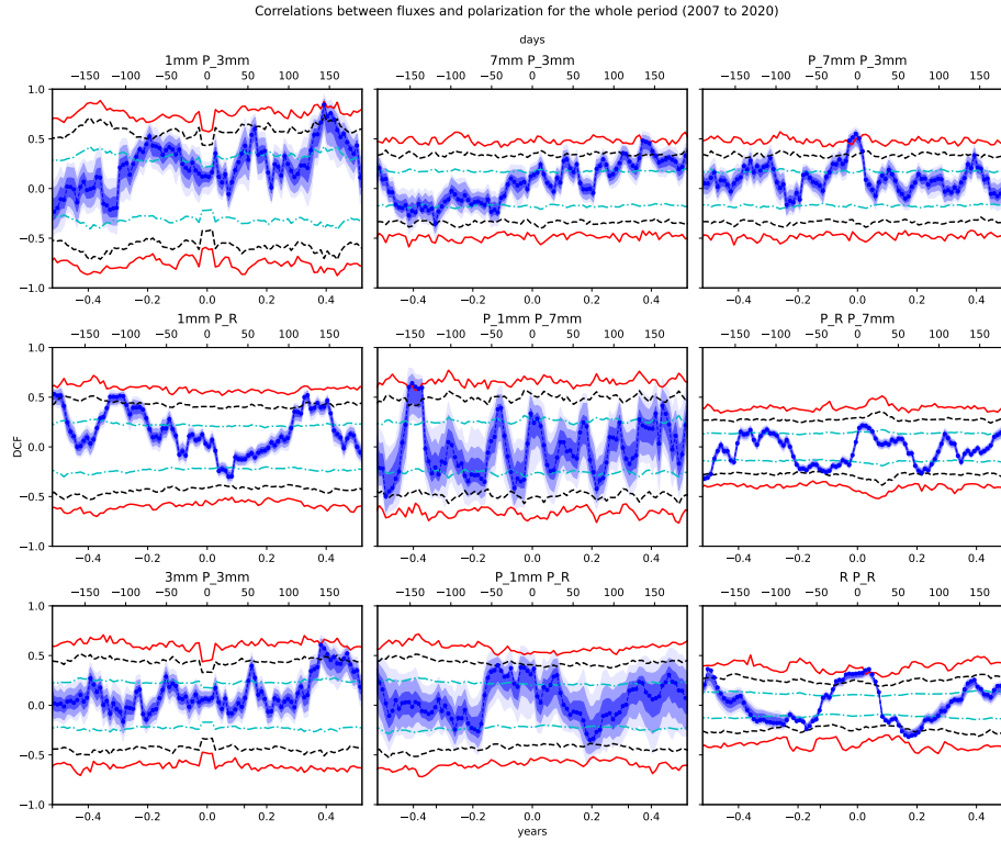
Fig. 10. Correlations between fluxes and polarization degree across all wavelengths. Horizontal lines show significance levels for 1\sigma , 2\sigma , and 3\sigma , computed using N = 2000 synthetic light curves, as described in Sect. 4.2. The DCFs here are computed using the whole period of available data, from 2007 to 2020.
