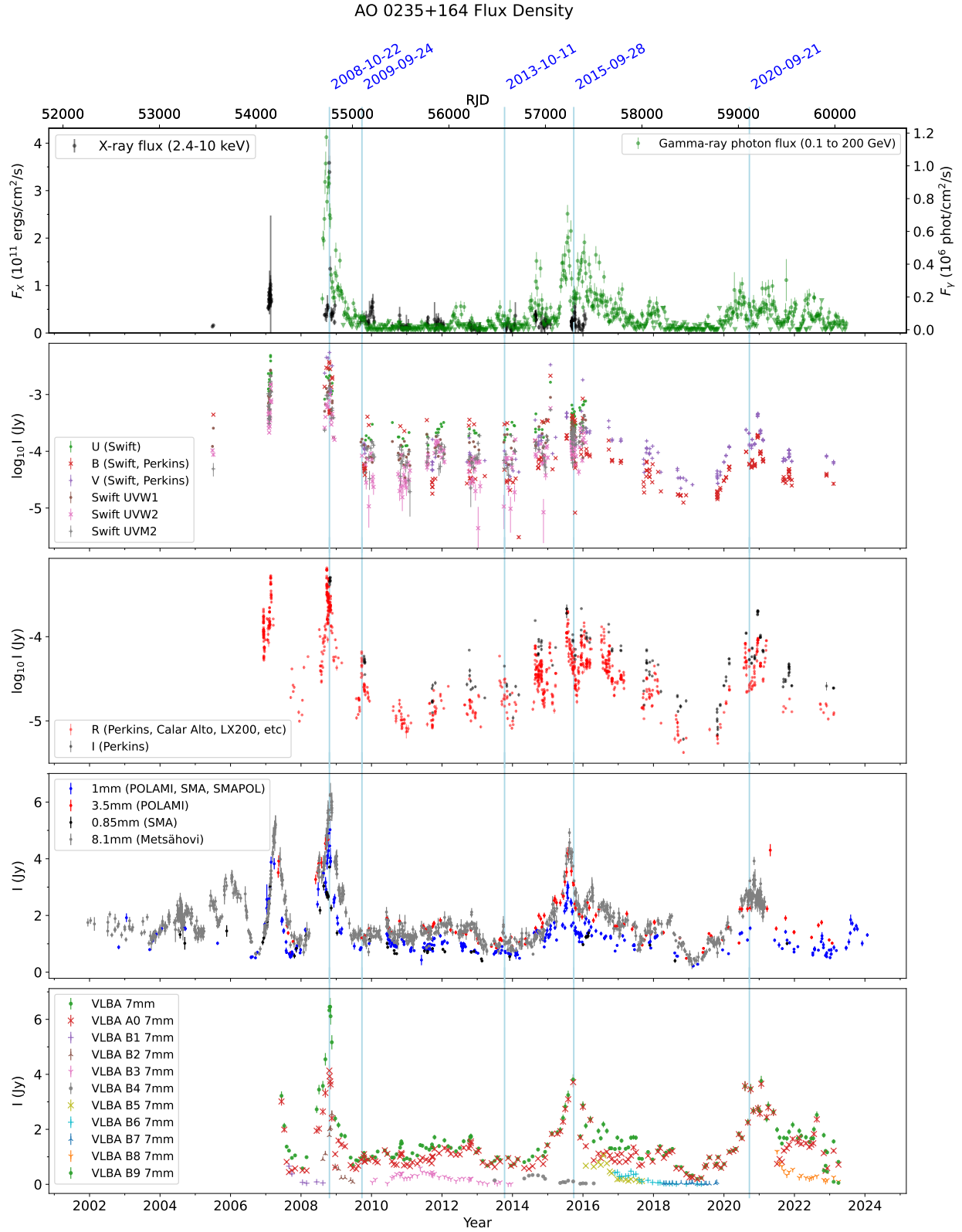
Fig. 1. Historical light curves of AO 0235+164 at different wavelengths. The first four vertical lines mark the epochs analyzed in Escudero et al. (2024) ; the last one corresponds to the epoch analyzed in Sect. 3.6.
