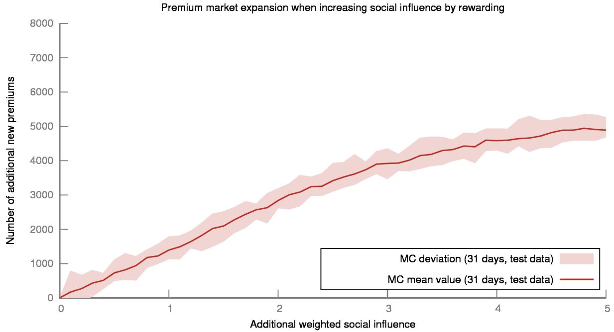
Figure 3: AN AGENT-BASED DSS SIMULATION OUTPUT OF ADDITIONAL PREMIUM ADOPTIONS WHEN REWARDING ADOPTERS VERSUS THE SOCIAL INFLUENCE PER DOLLAR.
