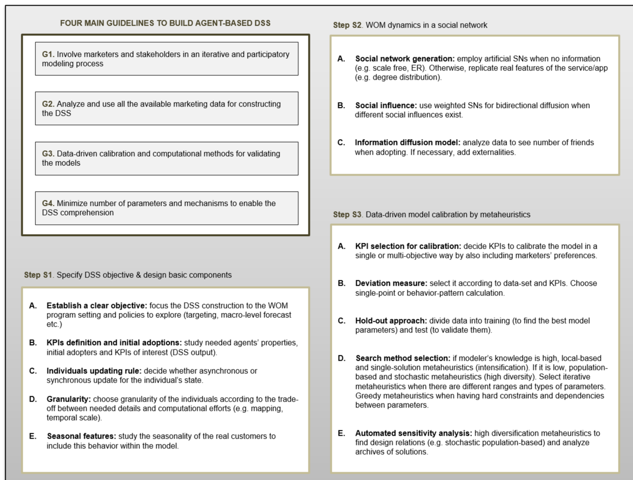
Figure 1: FOUR GUIDELINES AND THREE STEPS TO BUILD AN AGENT-BASED DSS FOR WOM PROGRAMS.
