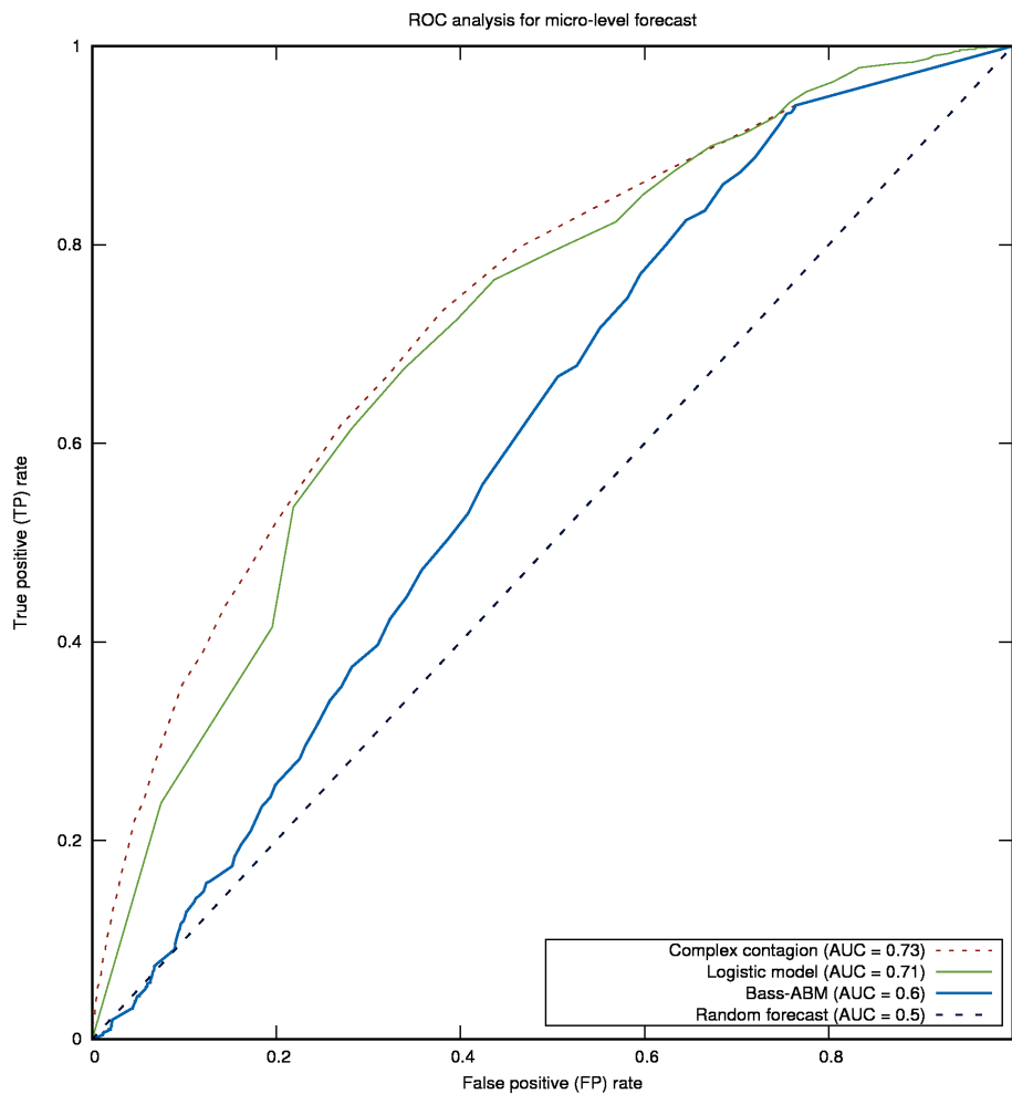
Figure 2: ROC ANALYSIS OF THE MODELS FOR THE MICRO-LEVEL FORECAST. AUC VALUES SHOWN IN THE LEGEND.
