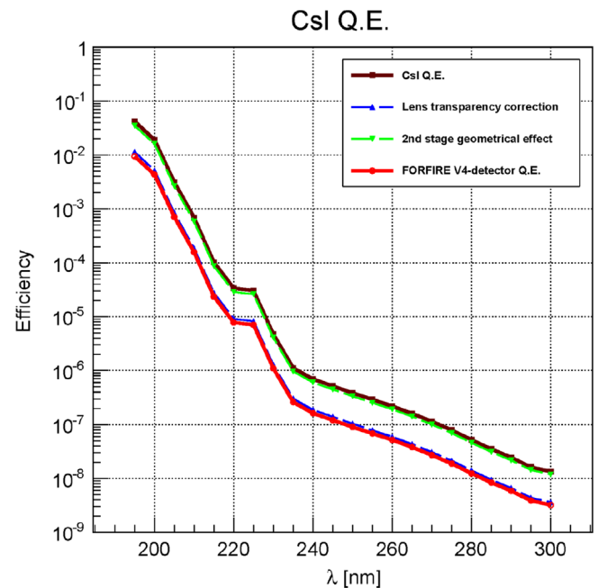
Fig. 3. Efficiency of the CsI photocathode.
