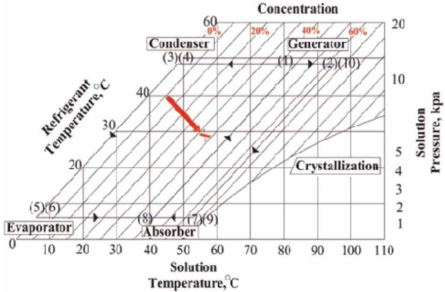
Figure 3. Single-stage absorption cycle on PTX diagram.
