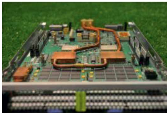
Figure 2. Water flows along copper pipes in a blade server used in the Aquasar supercomputer as in [17].
