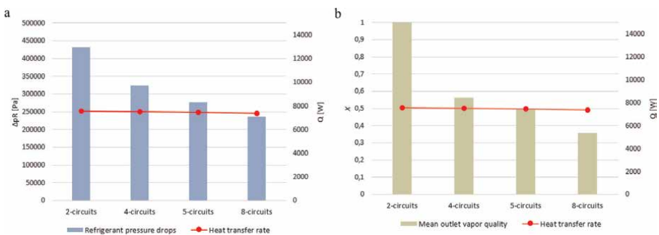
Figure 8. Test b: Refrigerant pressure drops (a) and mean outlet vapor quality (b) for each of the four circuit layouts of Set 1 [16].
