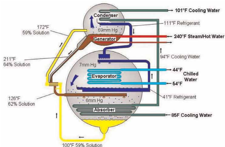
Figure 2. Simplified diagram of a single effect absorption cycle. Source: https://gasairconditioning.com/technologies/absorption/how-it-works/
