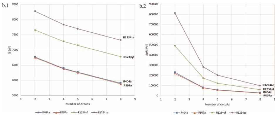
Figure 7. Test a, case b): Heat transfer rate (b.1) and refrigerant pressure drops (b.2) for each of the four circuit layouts of Set 1. Tested refrigerant: R404a, R507a, R1234yf, and R1234ze [16].
