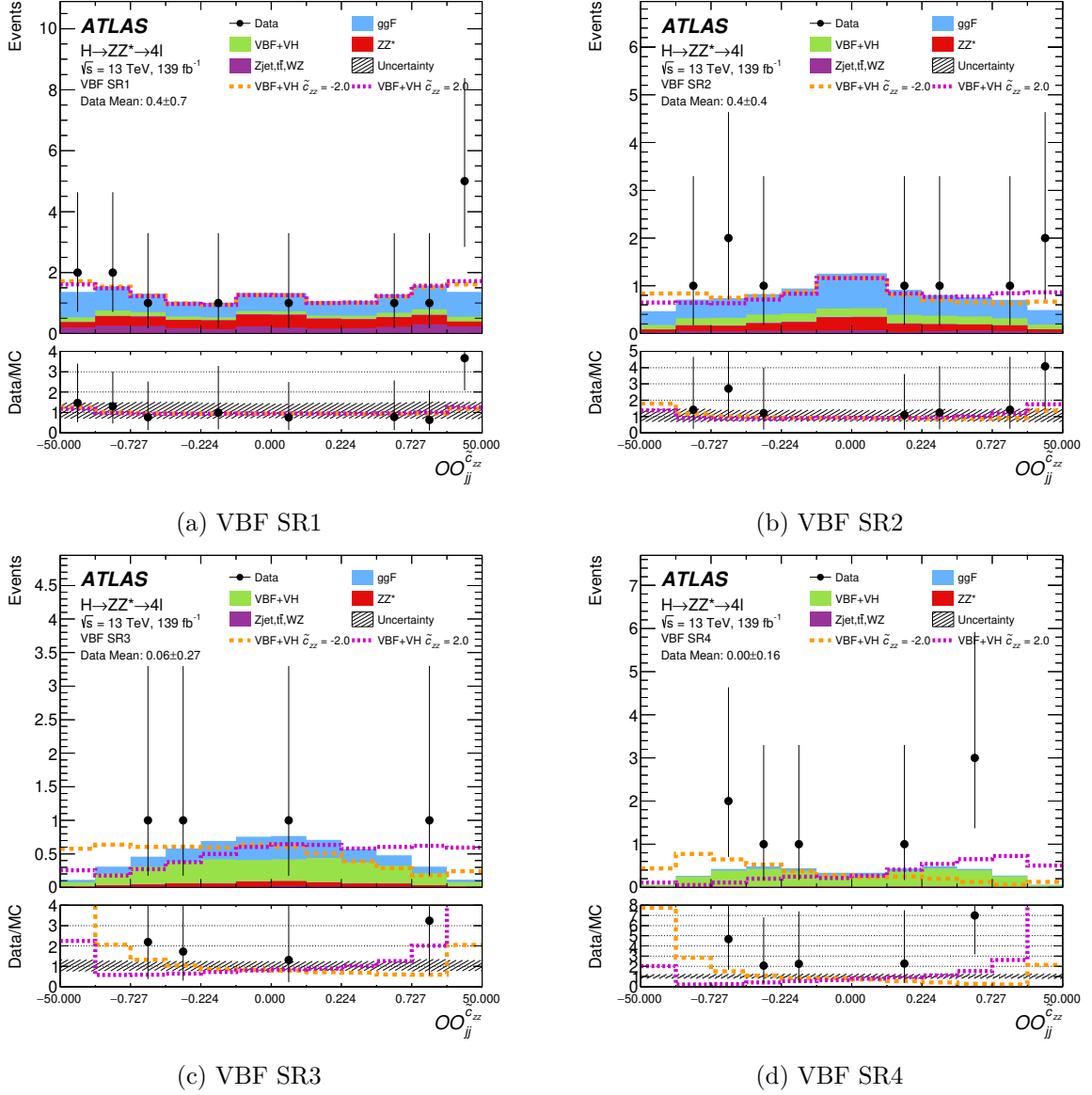
Figure 5. The observed and expected distributions for the production-level observable OO_{jj}^{\tilde{c}_{zz}} in each of the four VBF signal regions: (a) SR1, (b) SR2, (c) SR3, and (d) SR4. The expected distribution for the VBF signal and the backgrounds from ggF, ZZ^* , and reducible backgrounds are shown as a stacked histogram. Also shown are the expected distributions in presence of CP-odd contributions for \tilde{c}_{zz} = \pm 2.0 , assuming the VBF/ VH event rate remains that of the SM. The bin size is variable, optimized for an approximately flat distribution for the SM combined with a positive and negative BSM scenario. All events have optimal observable values within the limits of the plots. The mean value of the optimal observable across the data events is given with its standard deviation. The lower panels show the ratio of data to expectation and the shaded band corresponds to the combined statistical and systematic uncertainties in the predictions.
