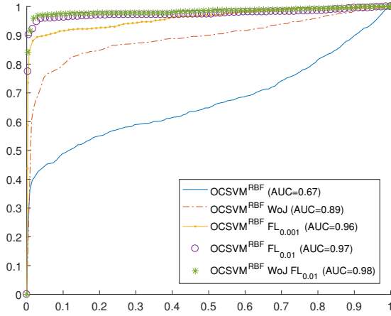
Fig. 8: ROC curves for OCSVM variants.
