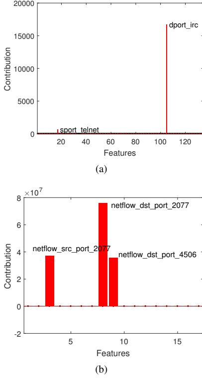
Fig. 4: Profile of detection of NERISBOTNET attacks with MBDA Opt (a) and MBDA FL 0.01 (b) using oMEDA.
