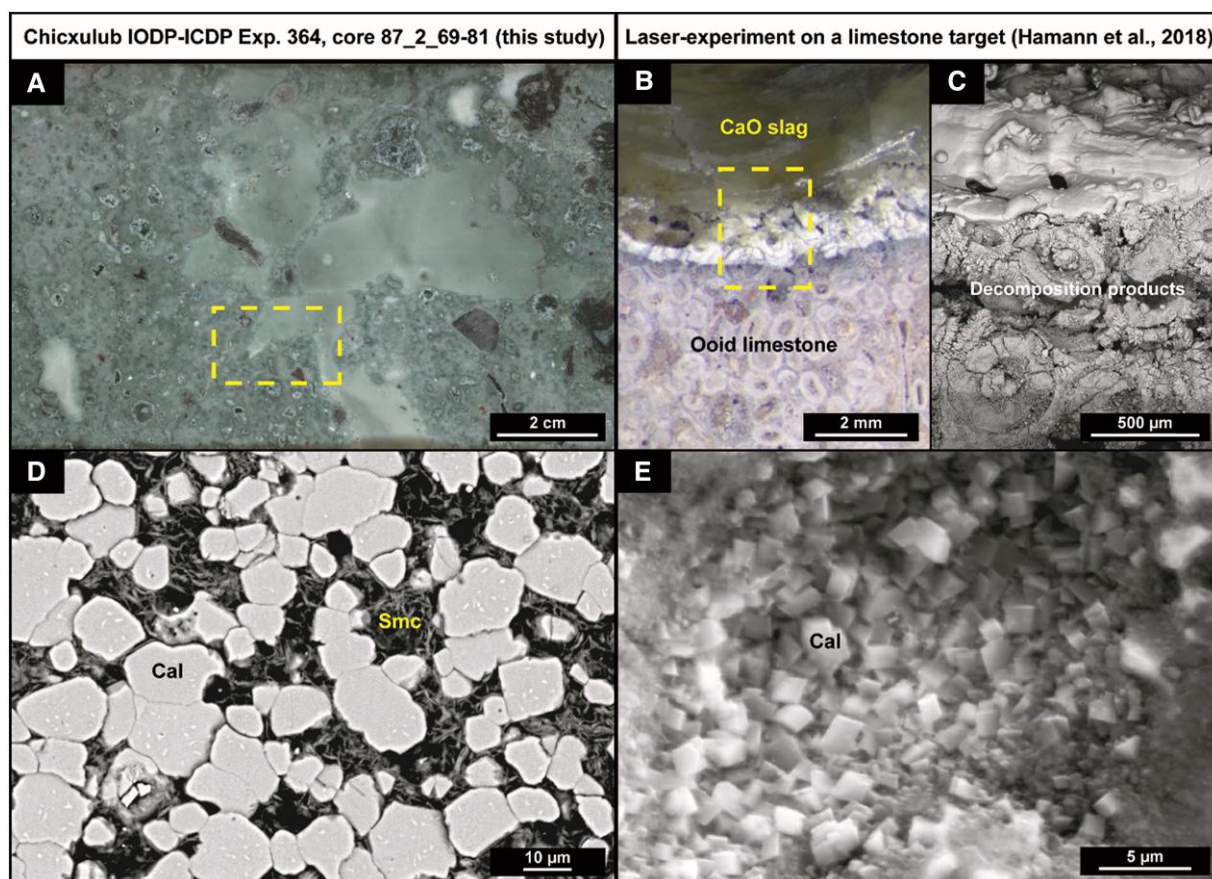
Fig. 4. Petrographic similarities between Chicxulub samples and experimental analogs. The IODP-ICDP Exp. 364 impact melt rock interval, yielding high T(\Delta_{47}) ( 327 \pm 33^\circ\text{C} [1 SE]), shows similar macro- and micro-textures compared to results from laser-irradiation experiments on a limestone target (8). A) Halfcore photograph of IODP-ICDP Exp. 364 core section 87_2 (69–81 cm; 721.35–721.47 mbsf) displaying smooth green textures, which were analyzed in this isotopic study (see yellow area and Fig. S1B sample #6). B) Reflected-light photomicrograph and C) zoomed-in scanning electron microscopy-backscatter electron (SEM-BSE) image of an ooid-limestone plate after laser irradiation, showing successive thermal decomposition of \text{CaCO}_3 resulting in white decomposition products and eventually in lustrous green CaO slag (modified from Hamann et al. [8]). D) Equigranular-like calcite matrix of the smooth textures in sample 721.45 mbsf, displaying subhedral calcite (Cal) grains of \sim 5\text{--}15\ \mu\text{m} in size, interspersed with minor smectite (Smc). E) Equigranular matrix of the zone with the decomposition products from the laser experiment showing euhedral calcite crystallites of \sim 1\text{--}2\ \mu\text{m} in size (modified from Hamann et al. [8]).
