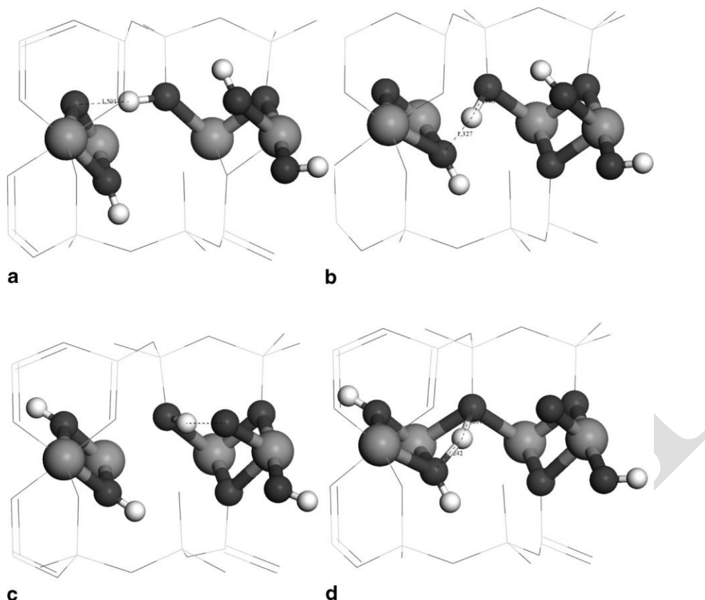
Figure 6. Transition states for the dehydroxylation reaction with apical oxygen assistance: (a,b) on-site mechanism [(a) apical oxygen protonation, (b) water molecule formation], (c,d) cross mechanism [(c) apical oxygen protonation, (d) water molecule formation]. The Si, Al, O, and H atoms are represented in dark gray, gray, black, and white, respectively.
