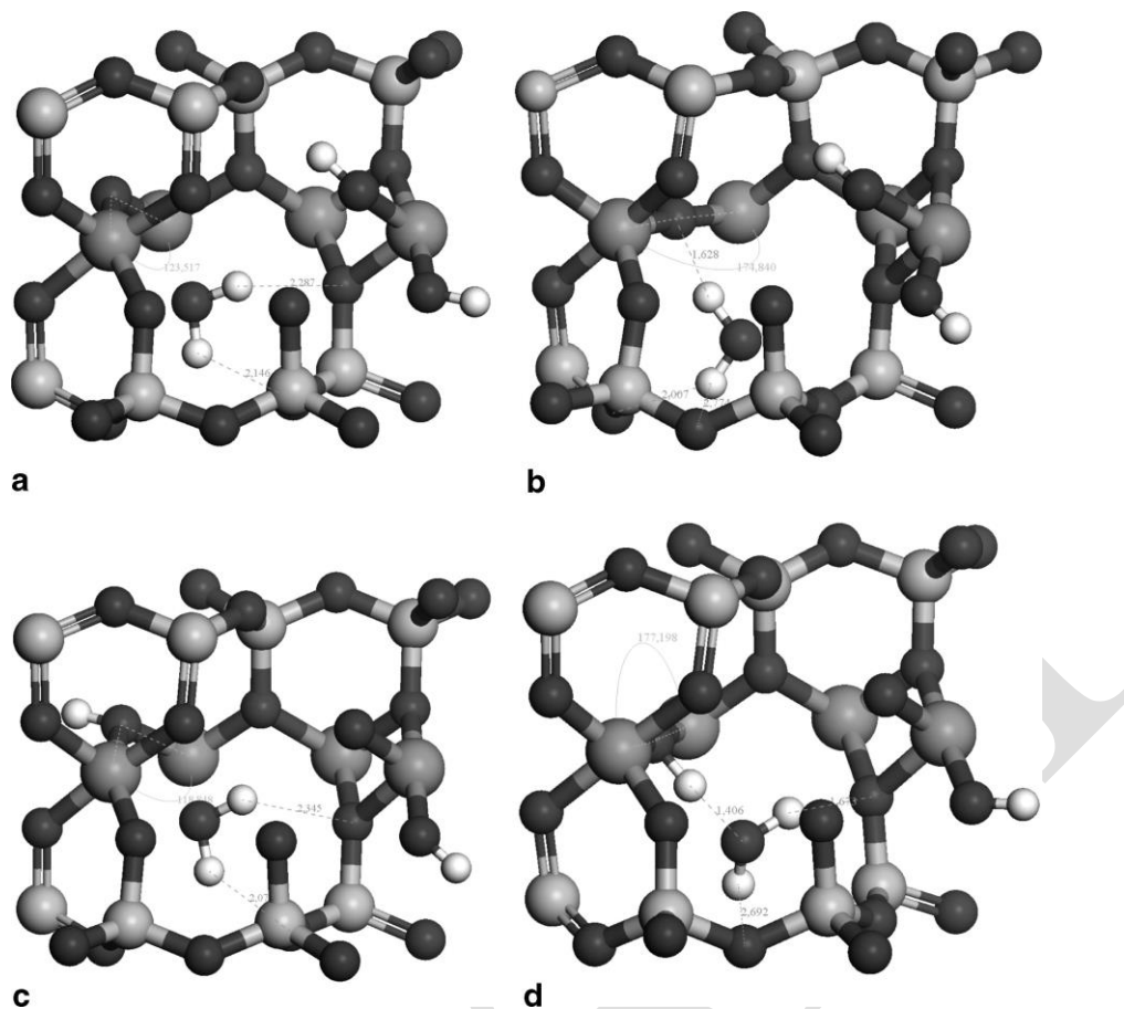
Figure 2. Interactions of the water molecule in the ditrigonal cavity in the optimized structures of the intermediates for the (a,b) on-site and (c,d) cross mechanisms. The Si, Al, O, and H atoms are represented in dark gray, gray, black, and white, respectively.
