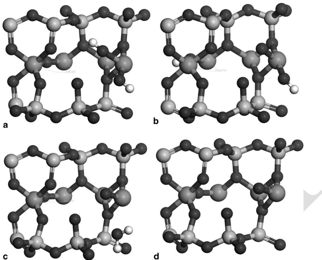
Figure 3. Semidehydroxylate derivatives without water for the (a) on-site and (b) cross intermediates. Dehydroxylate derivative (c) with water and (d) without water. The Si, Al, O, and H atoms are represented in dark gray, gray, black, and white, respectively.
