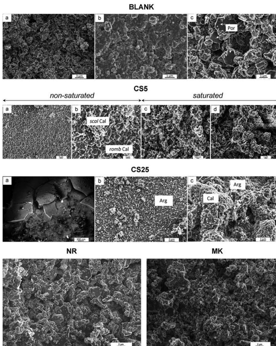
Fig. 6. FESEM images of cylindrical mortar samples: untreated (BLANK); treated with CaLoSil 5 g/L (CS5, saturated and non-saturated), CaLoSil 25 g/L (CS25), Nanorestore 5g/L (NR) and Merck 5 g/L (MK) dispersions after 8 weeks exposure at 90 % RH. Por: portlandite; Arg, aragonite; Cal: calcite; scal Cal , scalenohedral calcite; romb Cal : rhombohedral calcite.
