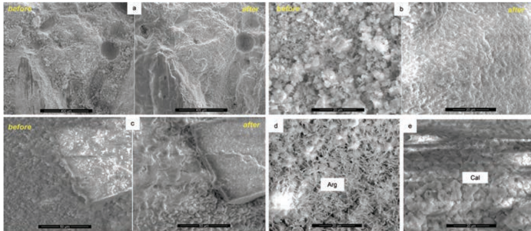
Fig. 7. ESEM images of areas of the same cubic sample before and after treatment with CaLoSil dispersion at 5 g/L. Arg, aragonite; Cal, calcite. Scales bars are 400 \mu\text{m} (a), 20 \mu\text{m} (b, d, e) and 50 \mu\text{m} (c).
