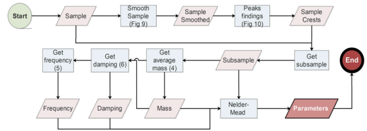
Fig. 11. First-phase algorithm implemented in FLEXOR
