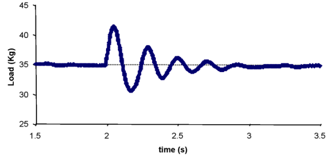
Fig. 4. Force-vs-time experimental record
