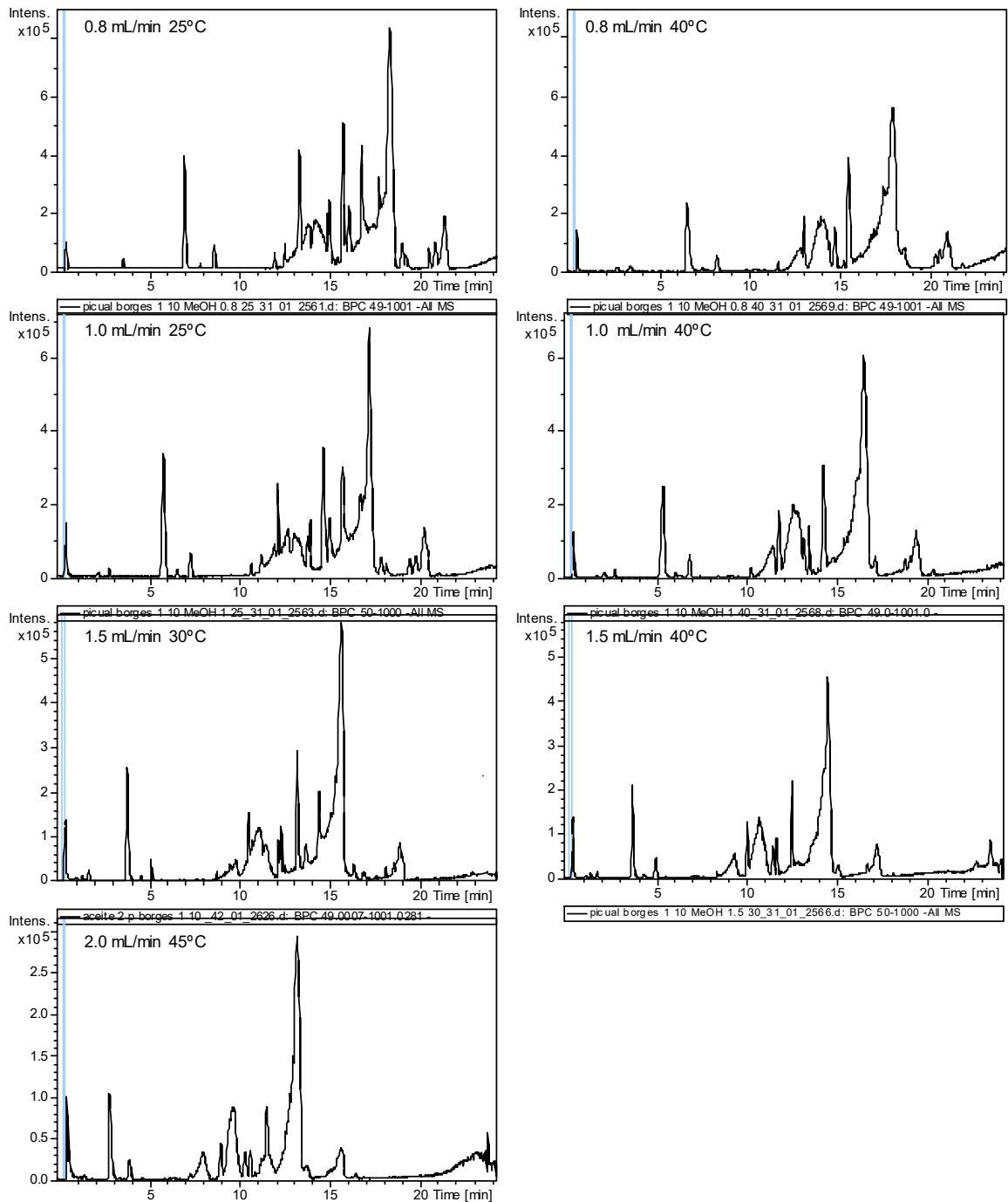
Fig. 1. RRLC-ESI-TOF Base peak chromatograms (BPC) of an olive oil extract (Picual Borges) using different mobile phase flow rates and temperatures. The rest of chromatographic conditions were those described in Section 2, the analytical column was a C18 Zorbax column, 1.8 \mu m, 4.6mm \times 150mm and the mobile phase: water + 0.5% acetic acid (A) and ACN (B).
