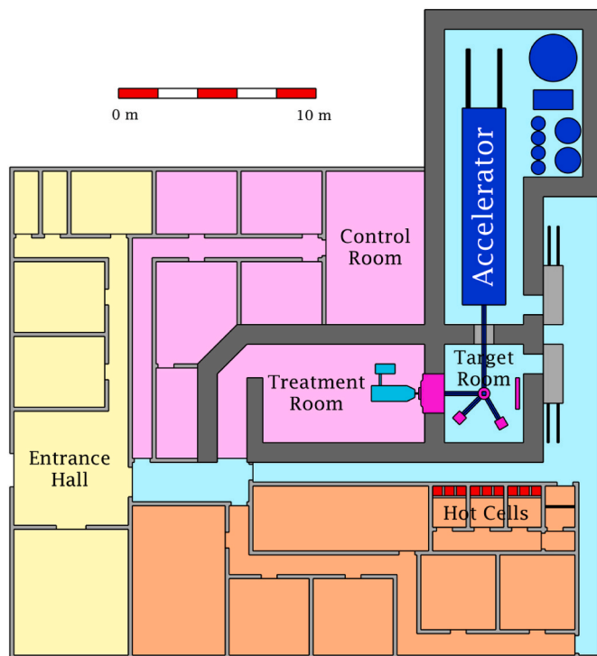
Fig. 6. Scheme of the facility: from the accelerator hall up to three beams will be extracted in the target area: (i) the one transporting protons to the beam shape assembly inserted in the shielding next to the treatment room, (ii) a second beam of protons will impinge another lithium target inside a moderator containing the target for radioisotope production by neutron capture, and (iii) a deuteron beam will hit the targets for PET radioisotope production. Also shown are the hot cells for radiopharmaceutical production.
