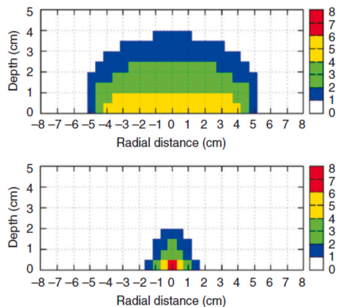
Fig. 5. Ratio of dose at tumor with respect to the maximum dose at normal tissue produced by an original cold beam of 10 × 10 cm (above) and the result of focalizing the beam at 5 × 5 cm (below).
