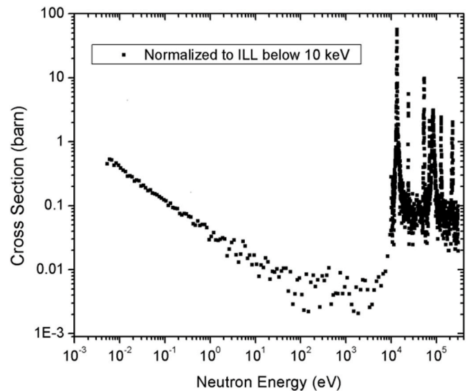
Fig. 4. Cross section values for the 33 S (n,α) reaction measured at nTOF and normalized to the thermal value from the ILL measurement. High resonances in the epithermal region have been confirmed.
