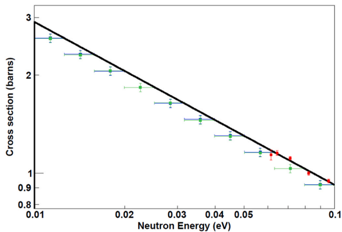
Fig. 2. Preliminary estimations of the cross section of the ^{14}\text{N} (n,p)^{14}\text{C} reaction (green dots) in the thermal region, compared to the ENDF-8 evaluation in black and previous measurements data (Koehler et al., 1989) in red. (For interpretation of the references to colour in this figure legend, the reader is referred to the Web version of this article.)
