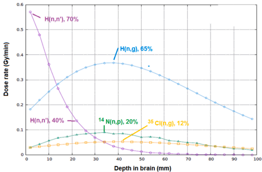
Fig. 3. Dose components due to the most relevant individual reactions, in brain tissue, as a function of depth, estimated with Monte Carlo simulations.
