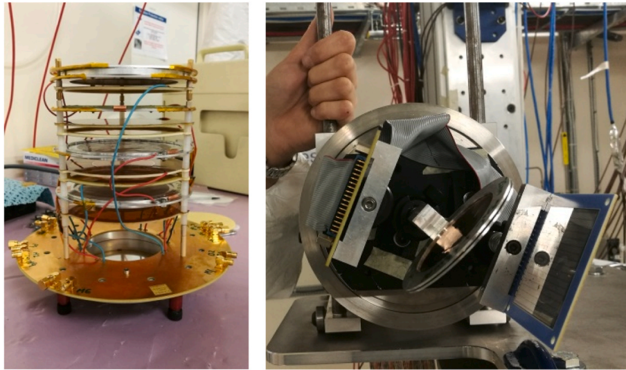
Fig. 1. The two detection systems used for the measurement of the ^{14}\text{N} (n,p)^{14}\text{C} reaction at n_TOF. The picture on the left shows the MicroMegs setup and the picture on the right shows the DSSSD setup.
