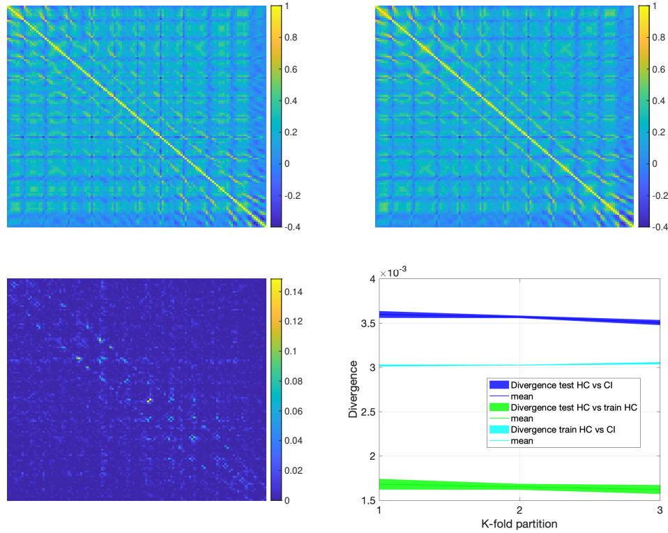
Figure 6. Correlation matrix of the HC (top left) and CI (top right) sample set using images scaled down to 12x12. Case-Control divergence matrix (bottom left). Divergence between the estimated correlation matrices of subsets of samples of healthy subjects and the set related to subjects with cognitive impairment (bottom right). The test HC set contains the same number of samples as the CI set, while the training HC contains the remaining samples. A 3-fold was performed to divide the set of healthy subjects and the results were randomised by 100 iterations. The thickness of the lines represents the standard deviation obtained by averaging the 100 values.
