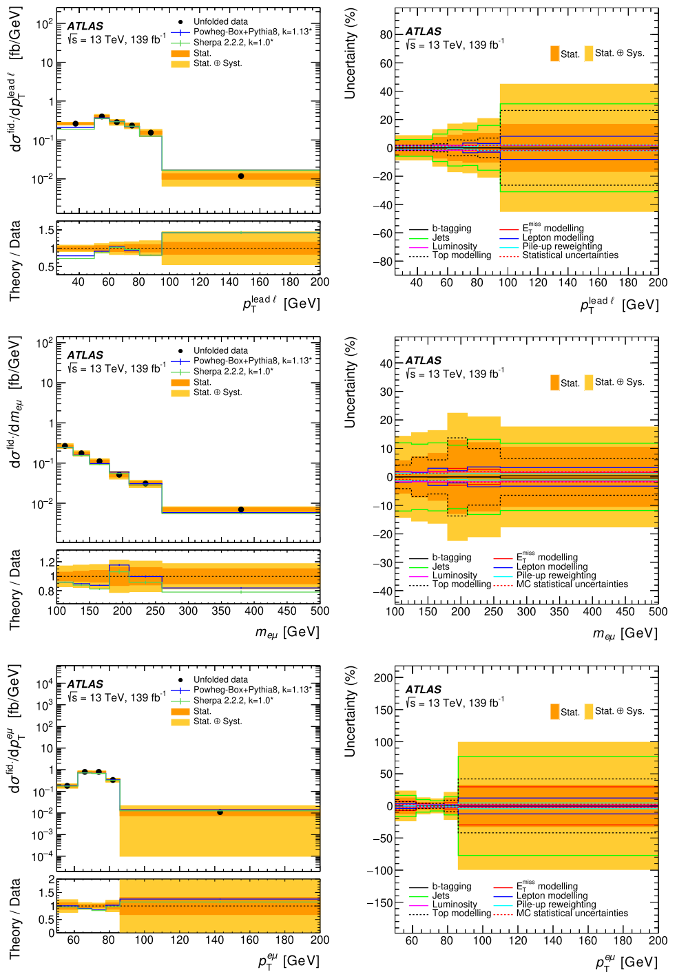
Fig. 4 Measured fiducial differential cross-sections of WW production for (top to bottom) p_T^{\text{lead } \ell} , m_{e\mu} and p_T^{e\mu} . The last bin is inclusive in the measured observable and for p_T^{e\mu} the first bin contains the underflow bin. The measured cross-section values are shown as points with dark bands giving the statistical uncertainty and light bands indicating the size of the total uncertainty. The results are compared with the q\bar{q} -initiated predictions from POWHEG BOX V2+PYTHIA 8.186 and SHERPA 2.2.2, each combined with SHERPA 2.2.2+OPEN LOOPS (LO+PS) for the gg -initiated states. The k -factors refer to the corrections applied to scale the predictions of qq -initiated and gg -initiated processes to NNLO and NLO accuracy in QCD respectively. The right column shows a breakdown of contributions to the uncertainties in the unfolded measurement
