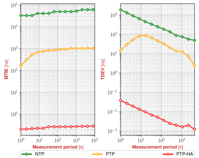
Fig. 9. MTIE and TDEV curves for the evaluation of the synchronization accuracy of the three protocols for a symmetrical bidirectional bandwidth utilization of 18% (maximum bandwidth tolerated by PTP fulfilling 1 \mu\text{s} of accuracy). 3 hours and a half of measurements (about 12600 samples) have been obtained for each curve.
