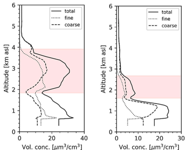
Fig. 14. Particle volume concentration for the different modes from the multi-wavelength Raman lidar plus sun-photometer configuration in GRASP algorithm: (a) 12 October 2021 at 13:29 UTC and (b) 20 October at 12:49 UTC. The volcanic aerosol layers are highlighted by the shadowed areas.
