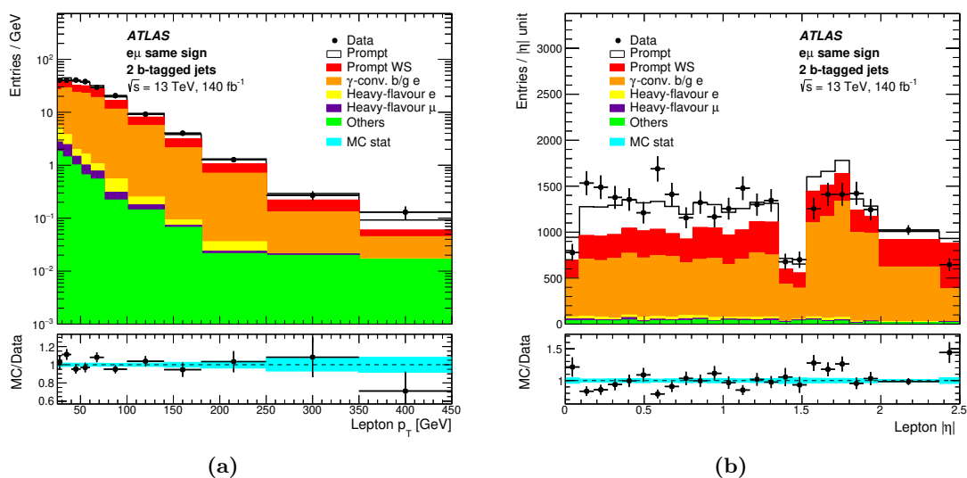
Figure 5. Distribution of lepton p_T (left) and |\eta| (right) in same-sign e\mu events with two b -tagged jets. The data (dots) are compared with the combined prediction from signal and background processes (line). The coloured distributions show the breakdown of the predicted contributions: wrong-sign (WS) prompt leptons, where the lepton charge is mismeasured; background electrons from photon conversions; electrons or muons from heavy-flavour decays; and other sources of fake leptons. The bottom panel shows the ratio of the predictions to the data with an uncertainty band covering the MC statistical uncertainty. The last bin of the p_T distribution includes overflow events.
