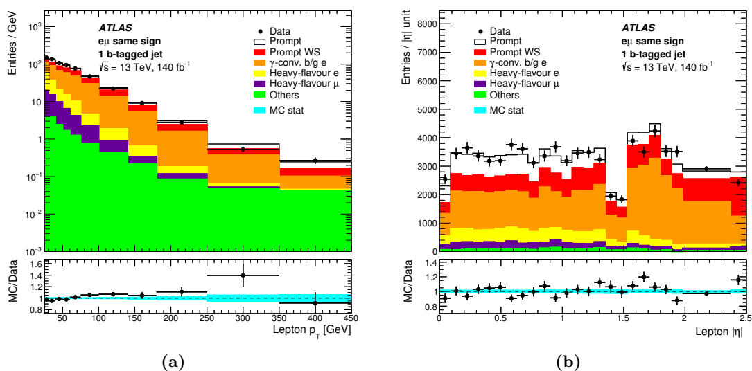
Figure 4. Distribution of lepton p_T (left) and |\eta| (right) in same-sign e\mu events with one b -tagged jet. The data (dots) are compared with the combined prediction from signal and background processes (line). The coloured distributions show the breakdown of the predicted contributions: wrong-sign (WS) prompt leptons, where the lepton charge is mismeasured; background electrons from photon conversions; electrons or muons from heavy-flavour decays; and other sources of fake leptons. The bottom panel shows the ratio of the predictions to the data with an uncertainty band covering the MC statistical uncertainty. The last bin of the p_T distribution includes overflow events.
