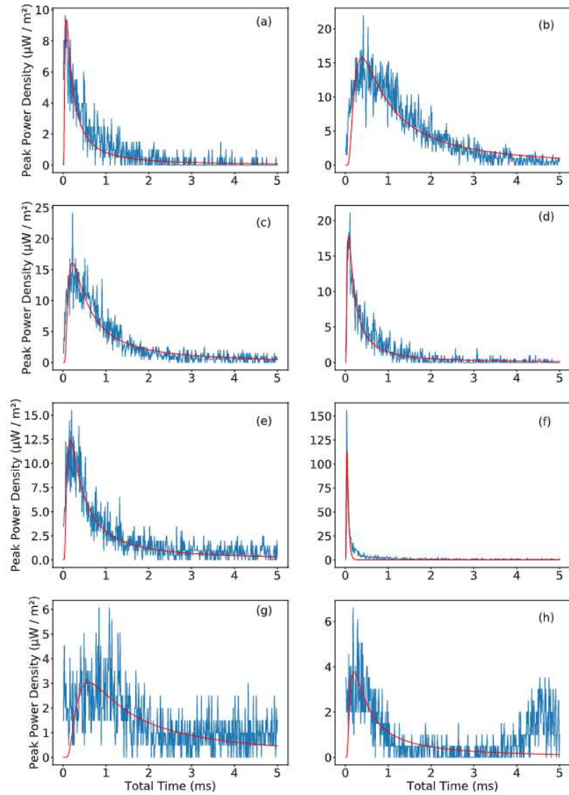
Figure 39. Examples of eight impulsive single pulse BLUEs fitted (red line) with the first hitting time (FHT) model resulting in a R^2 of (a) 0.75, (b) 0.80, (c) 0.85, (d) 0.90, (e) 0.79, (f) 0.86, (g) 0.24, and (h) 0.21.
