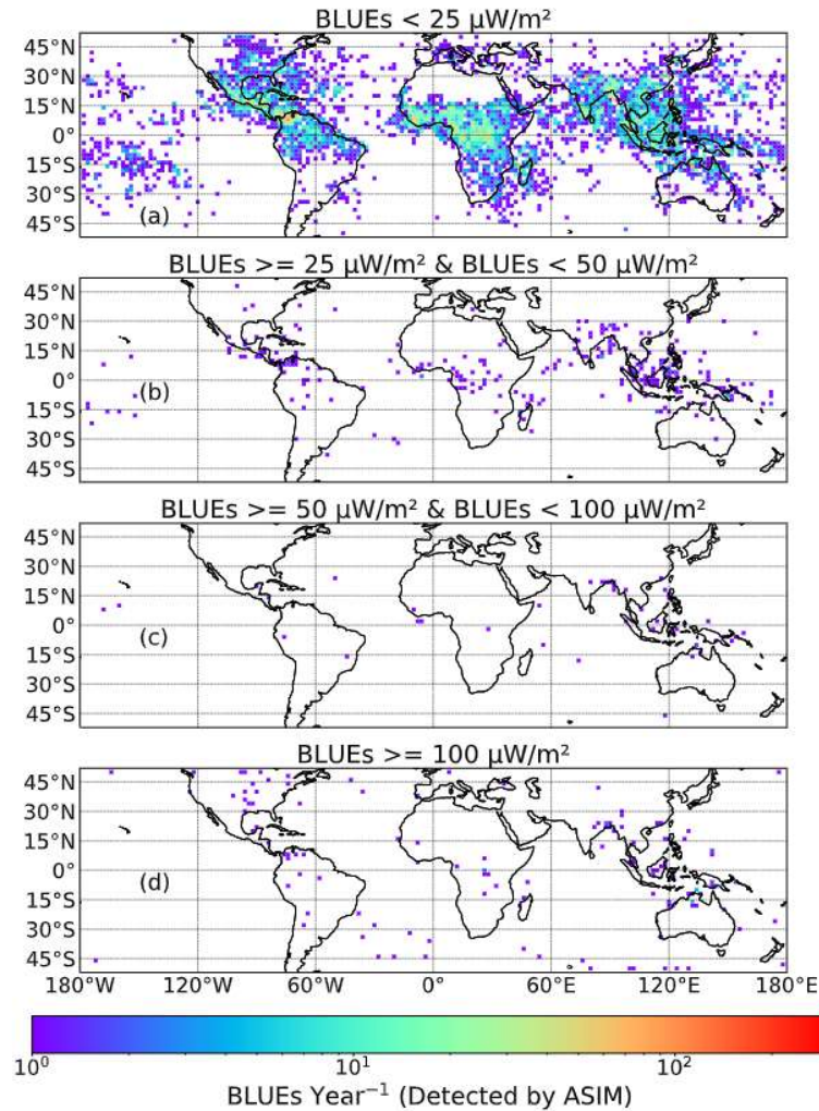
Figure 32. Geographical distribution (in 2^\circ \times 2^\circ grid cells) of the \sim 26,500 nighttime GD-2 BLUEs detected by ASIM-MMIA in the two-year period from 1 April 2019 to 31 March 2021 removing events in all the planet (including the SAA) with rise time ( \tau_{rise} ) \leq 40 \mu\text{s} and total duration ( \tau_{total} ) \leq 150 \mu\text{s} . Panels (a), (b), (c) and (d) show BLUEs of any shape with peak power density (PPD) between \geq 3 \mu\text{W m}^{-2} and < 25 \mu\text{W m}^{-2} , between \geq 25 \mu\text{W m}^{-2} and < 50 \mu\text{W m}^{-2} , between \geq 50 \mu\text{W m}^{-2} and < 100 \mu\text{W m}^{-2} , and \geq 100 \mu\text{W m}^{-2} , respectively. There are 25720 BLUEs in panel (a) (12860/year), 380 in panel (b) (190/year), 52 in panel (c) (26/year), and 204 in panel (d) (102/year). The BLUEs shown in these maps can have any temporal shape, that is, no distinction has been made here among BLUEs with a single (impulsive or not) pulse, multiple pulses or any other irregular pulse shape.
