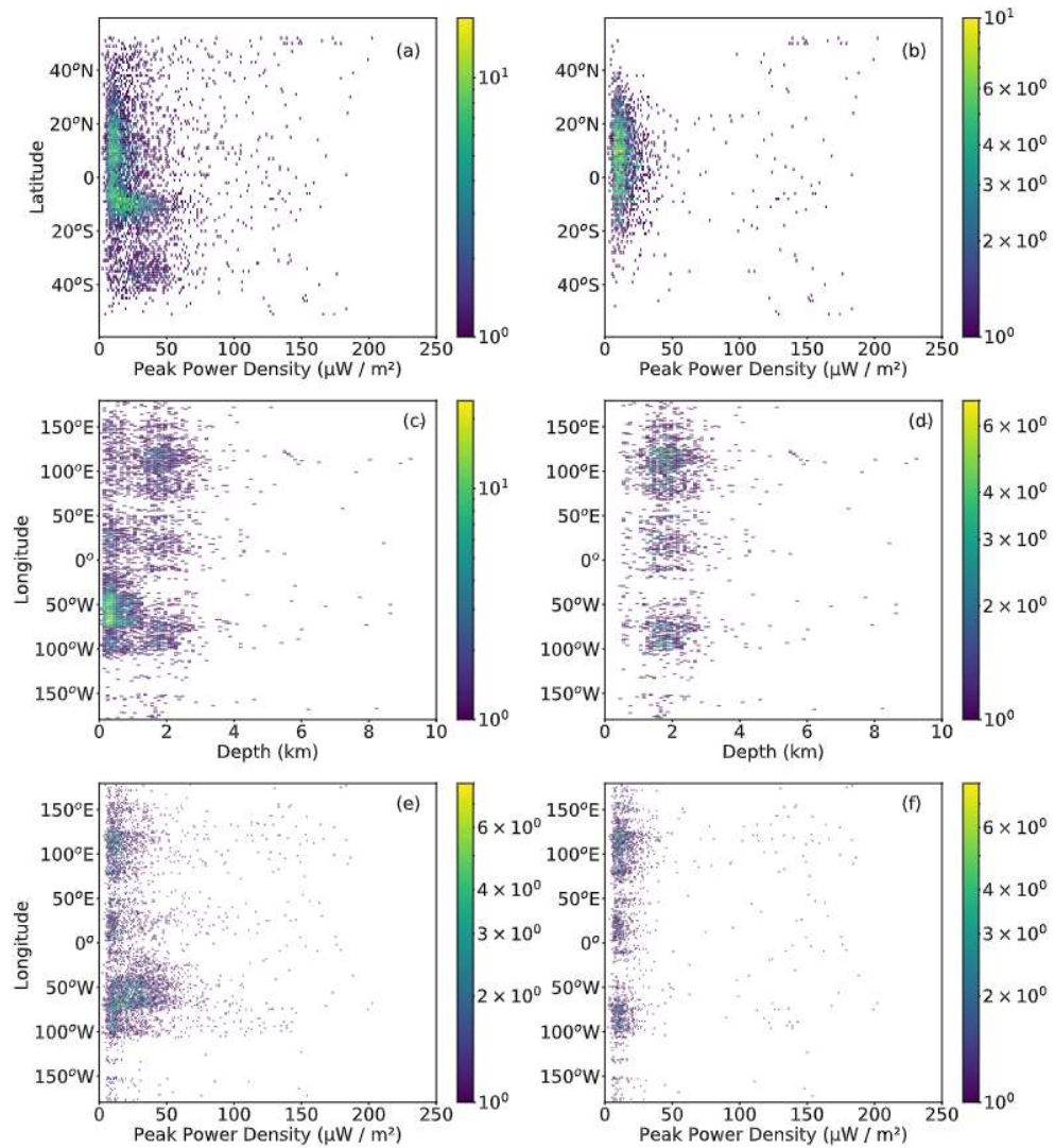
Figure 34. Zonal distributions of GD-1 and GD-2 impulsive single pulse BLUE peak power density (a, b). Meridional distributions of impulsive single pulse BLUE depths (c, d) and peak power density (e, f). Note that, always, GD-1 is in the left column and GD-2 is in the right column. The colorbar indicates number of events.
