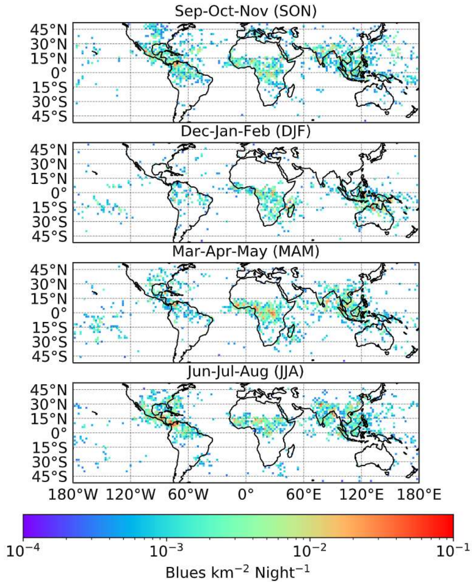
Figure 30. Nighttime seasonal distribution of BLUE electrical activity in thunderclouds associated to GD-2 in Figure 28. The global nighttime seasonal BLUE rates are: 3.7 (SON), 2.6 (DJF), 3.7 (MAM) and 4.0 (JJA) BLUEs \text{s}^{-1} . These maps are generated using 2^\circ \times 2^\circ grid cells. The BLUEs shown can have any temporal shape, that is, no distinction has been made here among BLUEs with a single (impulsive or not) pulse, multiple pulses or any other irregular pulse shape.
