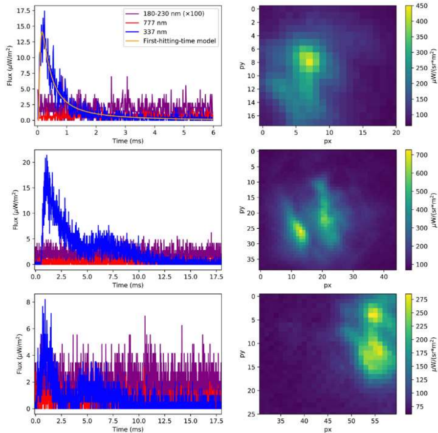
Figure 8. (Top panel) Photometer signal (left) and 337.0 nm image (right) recorded by MMIA at 13:09:45.0861 UTC (source) corresponding to a narrow single pulse blue event illuminating a cloud top area of 31.4 km 2 . The photometric signal (blue line) is well fitted by a distribution accounting for the scattering and absorption of photons in the thundercloud (orange line). Note that the 777.4 nm signal (red line) typical of lightning is in the noise level. The 180 - 230 nm photometric signal is also represented (purple line) with a \times 100 factor. (Middle and bottom panels) Photometer signals (left) and images (right) recorded by MMIA corresponding to double pulse (middle panel) and multiple pulse (bottom panel) blue flashes lasting above 14 and 8 milliseconds, respectively. Signals in the noise level are simultaneously detected in the MMIA 777.4 nm photometer and camera.
