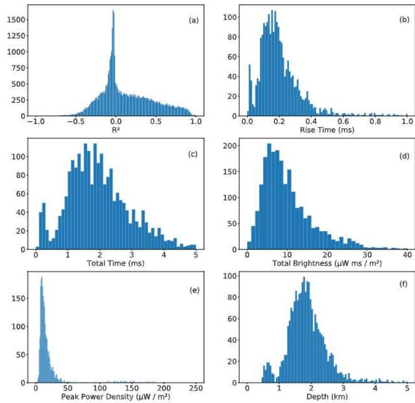
Figure 46. Histograms for BLUEs in GD-2 (see Figure 28 of main paper) recorded by ASIM-MMIA within 1 April 2019 to 31 March 2021. Events in panels (b) through (f) are fitted with the first hitting time (FHM) model (Soler et al., 2020; Luque et al., 2020) assuming point-like light sources. The different histograms show the number of BLUEs for different (a) R^2 (bin = 0.01), (b) Rise Time (ms) (bin = 0.01), (c) Total Times (ms) (bin = 0.1), (d) Total Brightness ( \mu\text{W ms m}^{-2} ) (bin = 1), (e) Peak Power Density ( \mu\text{W m}^{-2} ) (bin = 1), and (f) Depth (km) (bin = 0.05) below cloud tops. Note that impulsive single pulse BLUEs are only those for which R^2 > 0.75 (panels (b) through (f)). Please note that the word bin is used with the meaning of step.
