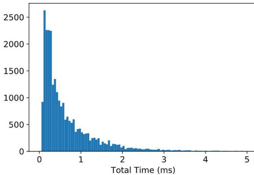
Figure 52. Histogram showing the number of BLUEs with all sort of temporal shapes (not only impulsive single pulse ones) geographically distributed according to GD-2 (see Figure 28 of main paper) with different total times (ms) (bin = 0.05 ms). Please note that the word bin is used with the meaning of step.
