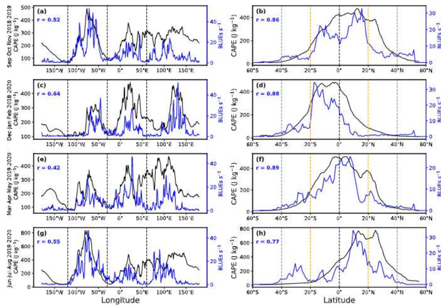
Figure 26. Seasonal meridional (left) and zonal (right) nighttime distributions of 2-year (1 September 2018 to 31 August 2020) BLUE climatology (blue line) and monthly average values of CAPE (black line) in the same period. Vertical lines as in Figure 11 of the main paper. The Pearson linear correlation coefficient ( R ) is shown in the inset of each panel.
