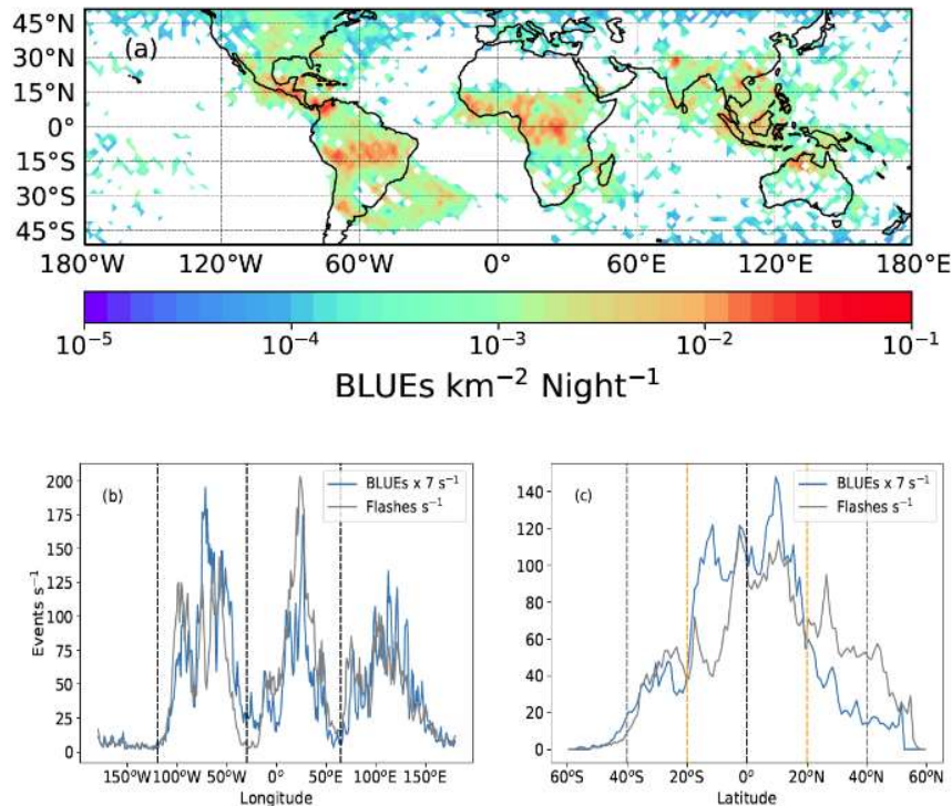
Figure 11. Panel (a): Two-year average (September 2018 through August 2020) nighttime climatology of global BLUE electrical activity in thunderclouds. The map is generated using 2^\circ \times 2^\circ grid cells where the sharp pixels of the image are smoothed by drawing level lines using the python function called contourf . Decimal logarithm is used in the colorbar scale so that 0.08 (roughly the maximum in the map) corresponds to \sim 30 BLUES \text{km}^{-2} \text{year}^{-1} provided night and day have the same global flash rate. Panels (b, c): Annual cycle (for the period investigated) of ASIM-MMIA nighttime global BLUE flash rate (blue line) and ISS-LIS global nighttime flash rate (gray line) represented in meridional (b) and zonal (c) distributions. Three BLUE and nighttime lightning chimneys are clearly distinguishable in the Americas ( 120^\circ\text{W} - 25^\circ\text{W} ), Africa/Europe ( 25^\circ\text{W} - 60^\circ\text{E} ) and Asia/Australia ( 60^\circ\text{E} - 180^\circ\text{E} ) in the meridional distributions. There is a fourth chimney slightly visible around 150^\circ\text{W} - 15^\circ\text{S} near Tahiti. Tropical ( 20^\circ\text{S} - 20^\circ\text{N} ), subtropical ( 40^\circ\text{S} - 20^\circ\text{S} , 20^\circ\text{N} - 40^\circ\text{N} ) and midlatitude ( 60^\circ\text{S} - 40^\circ\text{S} , 40^\circ\text{N} - 60^\circ\text{N} ) regions are indicated in the zonal distributions with dashed orange and gray vertical lines, respectively. The (b) and (c) panels were generated using 1^\circ \times 1^\circ grid cells. A non smooth two-year average nighttime climatology map of BLUES is shown in Figure 24 of the SM. Note that the global BLUE rates are scaled up 7 times for best comparison with global nighttime lightning flash rates.
