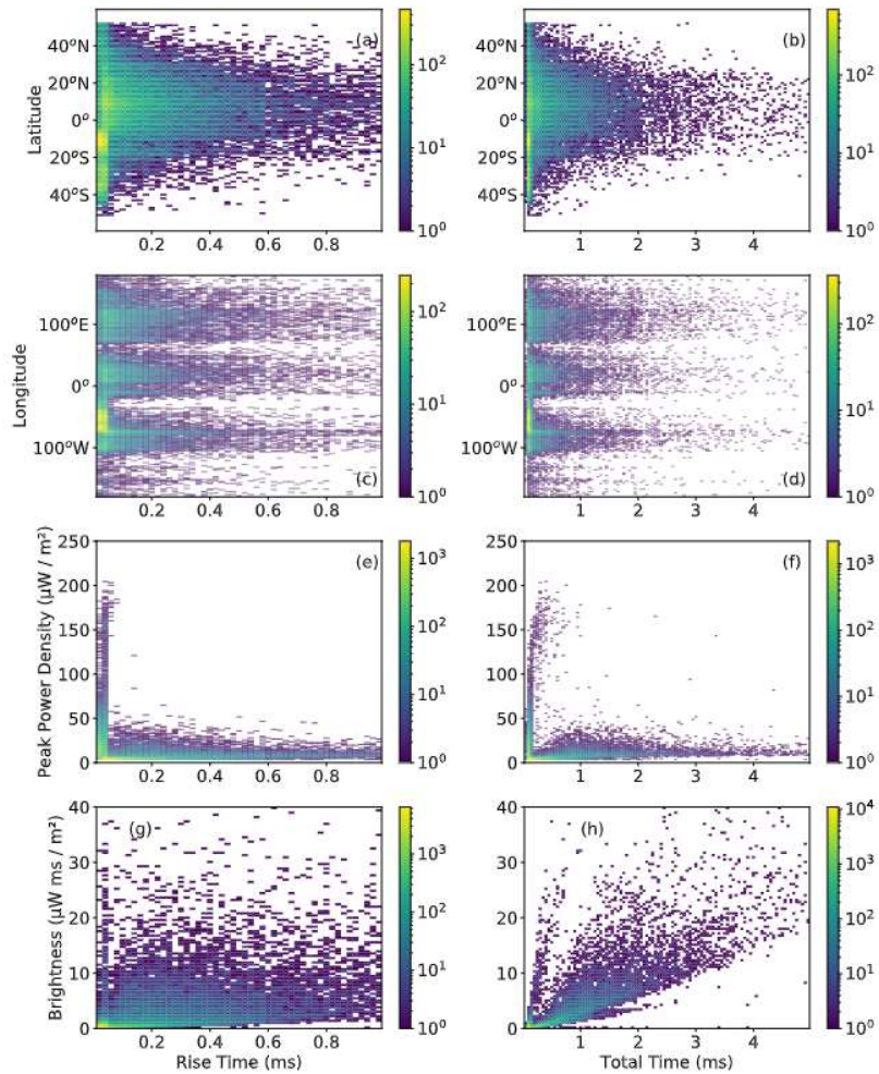
Figure 57. Zonal (a, b) and meridional (c, d) distributions of rise times and total times (duration) of BLUE with all sort of shapes (single pulse (impulsive or not), multiple pulse, irregular pulse) distributed according to GD-1. Variation of the peak power density and total brightness as a function of the BLUE rise times (e, g) and total time (duration) (f, h). The colorbar indicates number of events.
