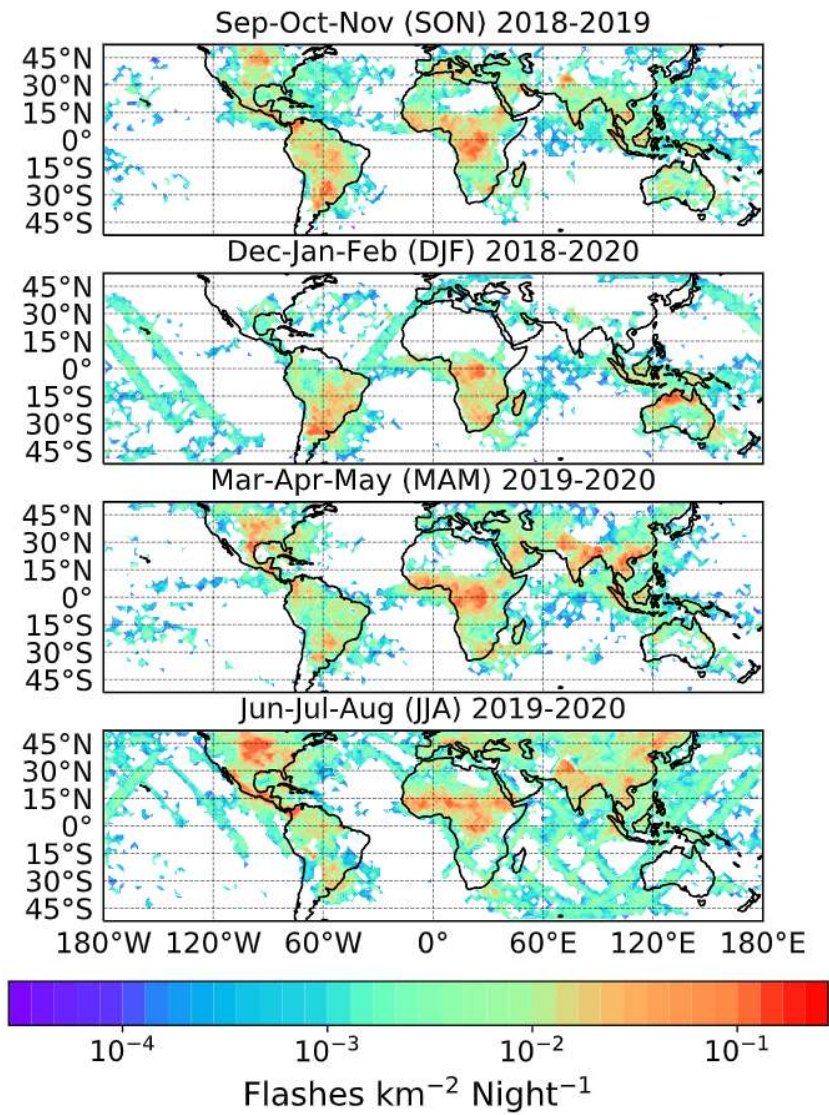
Figure 18. Seasonal nighttime lightning flash distributions from the ISS-Lightning Imager Sensor (LIS) climatology for the 2-year period from 1 September 2018 to 31 August 2020 with an average spatial resolution of 5 km/pixel and an assumed average detection efficiency (DE) of 100 %. The obtained ISS-LIS seasonal nighttime only lightning global flash rates are: 45.9 (SON), 33.7 (DJF), 50.4 (MAM) and 61.9 (JJA) flashes s -1 , respectively. Grid cells as in Figure 17.
