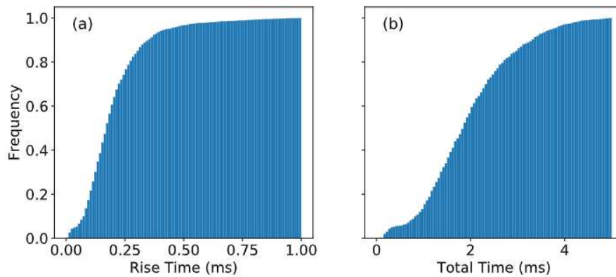
Figure 50. Frequency histograms showing the cumulative frequency of impulsive single pulse BLUEs (with R^2 > 0.75 ) in GD-2 (see Figure 28 of main paper) with different (a) Rise Times (ms) (bin = 0.01 ms) and (b) Total times (ms) (bin = 0.05 ms). These histograms indicate that, for instance, 10 % of impulsive single pulse BLUEs among all BLUEs in GD-2 have rise times and durations \leq 80 \mu\text{s} and \leq 900 \mu\text{s} , respectively. Note that GD-2 (in Figure 28 of main paper) represents the geographical distribution of BLUEs with all sort of temporal shapes, not only impulsive single pulse ones. Please note that the word bin is used with the meaning of step.
