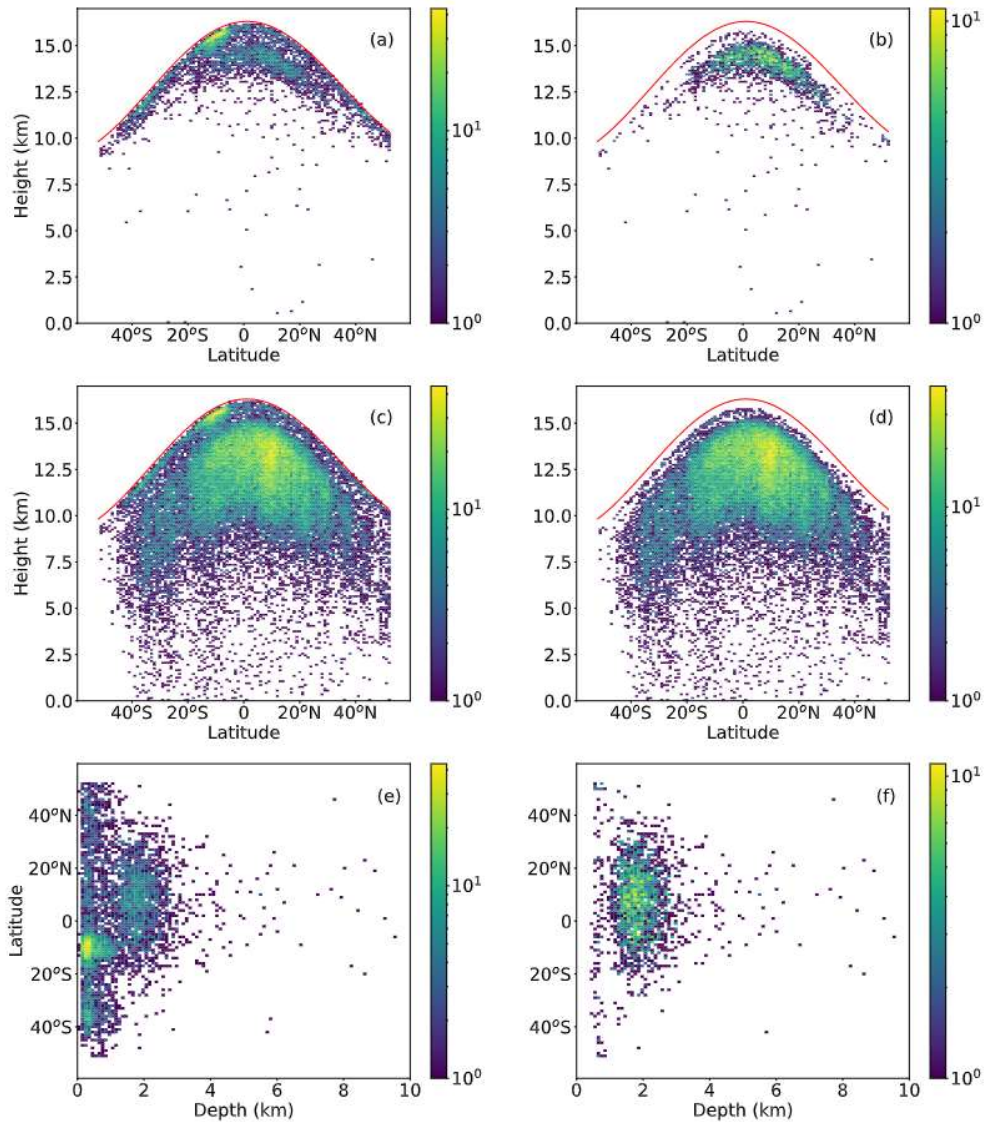
Figure 33. Approximate altitude distributions of GD-1 (left column) and GD-2 (right column) impulsive single pulse BLUEs (with R^2 > 0.75 ) (a, b), all sort of first hitting time (FHT) fittable BLUEs in GD-1 and GD-2 with any value of R^2 (c, d). Zonal distributions of GD-1 and GD-2 impulsive single pulse BLUE depths (e, f). Note that, always, GD-1 is in the left column and GD-2 is in the right column. The colorbar indicates number of events.
