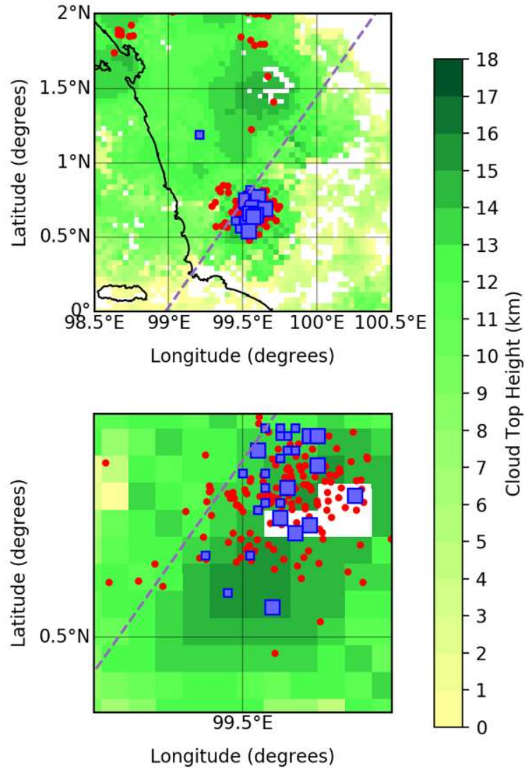
Figure 6. (Upper panel) Single (big blue squares), double and multiple pulse blue events (small blue squares) and cloud to ground (CG) lightning (small red dots) detected between 13:09 and 13:12 UTC by GLD360 represented over a cloud top height (CTH) map derived from ( 4 \text{ km} \times 4 \text{ km} spatial resolution) measurements by the Chinese Fengyun-4A (FY-4A) geostationary meteorological satellite. (Bottom panel) zoom-in of the top panel where more details can be observed. Thundercloud CTHs between 14 km and 15 km close to the tropopause are visible. The white spots are missing values. The dashed line represents the ISS orbit.
