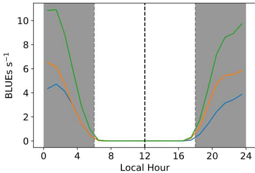
Figure 14. Diurnal (24 h) variability of global total (green line), land (orange line) and ocean (blue line) BLUE flash rate as a function of the local solar hour. The net zero rate during local daytime is caused by the fact that ASIM-MMIA can only observe during local nighttime. Local nighttime periods appear shadowed in the figure. Note that, for comparison, Figure 23 in the SM shows the diurnal (day and night) cycle of ISS-LIS total, land and ocean lightning flash rates for the two-year period investigated.
