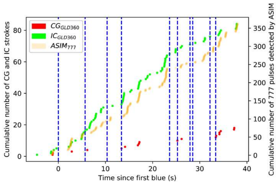
Figure 7. The vertical dashed lines indicate the temporal sequence of single pulse blue flashes detected by ASIM. The right axis marks the cumulative number of ASIM 777.4 nm flashes (orange dots) detected in its field of view between 5 seconds before the first single pulse blue flash and 5 seconds after the last single pulse blue event. The left axis indicates the cumulative number of cloud discharges classified by GLD360 as CG lightning strokes (red dots) and IC lightning strokes (green dots) occurring within a square of 1^\circ side centered in the centroid of the blue events and counting between 5 seconds before the first single pulse blue flash and 5 seconds after the last single pulse blue event.
