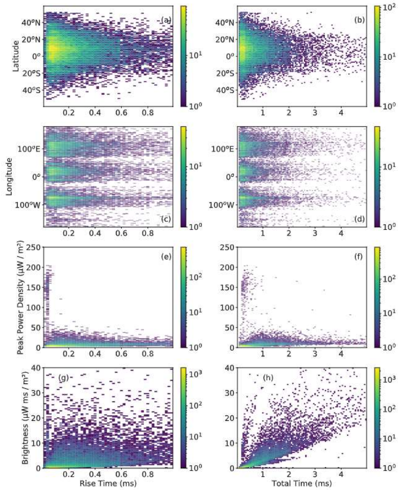
Figure 58. Zonal (a, b) and meridional (c, d) distributions of rise times and total times (duration) of BLUE with all sort of shapes (single pulse (impulsive or not), multiple pulse, irregular pulse) distributed according to GD-2. Variation of the peak power density and total brightness as a function of the BLUE rise times (e, g) and total time (duration) (f, h). The colorbar indicates number of events.
