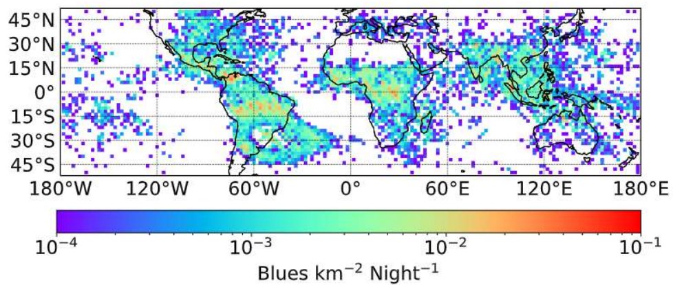
Figure 27. Two-year average (1 April 2019 through 31 March 2021) nighttime climatology of global BLUE electrical activity in thunderclouds (GD-1) showing \sim 46,000 BLUEs. The map is generated using 2^\circ \times 2^\circ grid cells. The BLUEs shown can have any temporal shape, that is, no distinction has been made here among BLUEs with a single (impulsive or not) pulse, multiple pulses or any other irregular pulse shape. The annual global rate of GD-1 BLUEs peak at 9.5 \text{ events s}^{-1} in the local midnight (00.00 local solar time), and show a decreasing global rate as local daytime approaches (and there is less MMIA observation time). On average, the global annual average rate of BLUEs in GD-1 is 6.0 \text{ events s}^{-1} . Note that ASIM can only observe during the night.
