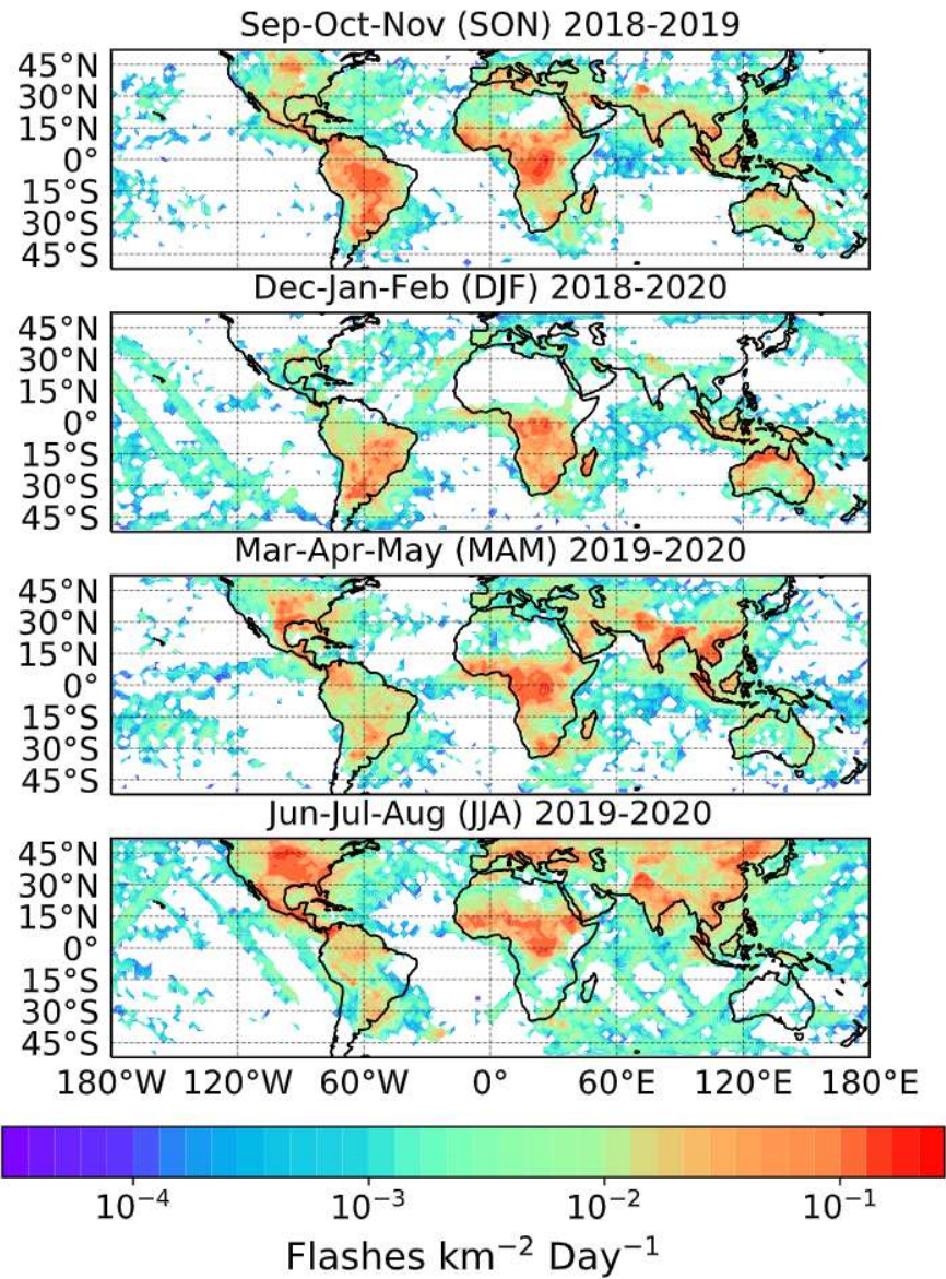
Figure 21. Full day (night and day) ISS-LIS seasonal lightning climatology for the 2-year period 1 September 2018 to 31 August 2020 investigated here. The obtained ISS-LIS seasonal 24 h lightning global flash rates are: 47.5 (SON), 32.0 (DJF), 47.0 (MAM) and 60.8 (JJA) flashes s -1 , respectively. Grid cells as in Figure 17.
