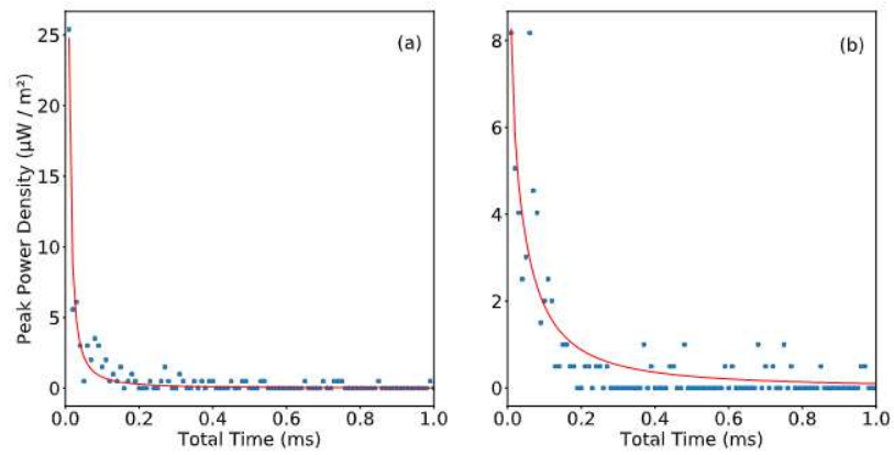
Figure 40. Examples of two BLUE events fitted (red line) assuming that they are extended sources reaching the cloud top. The fit results in a R^2 of (a) 0.94, and (b) 0.75.
