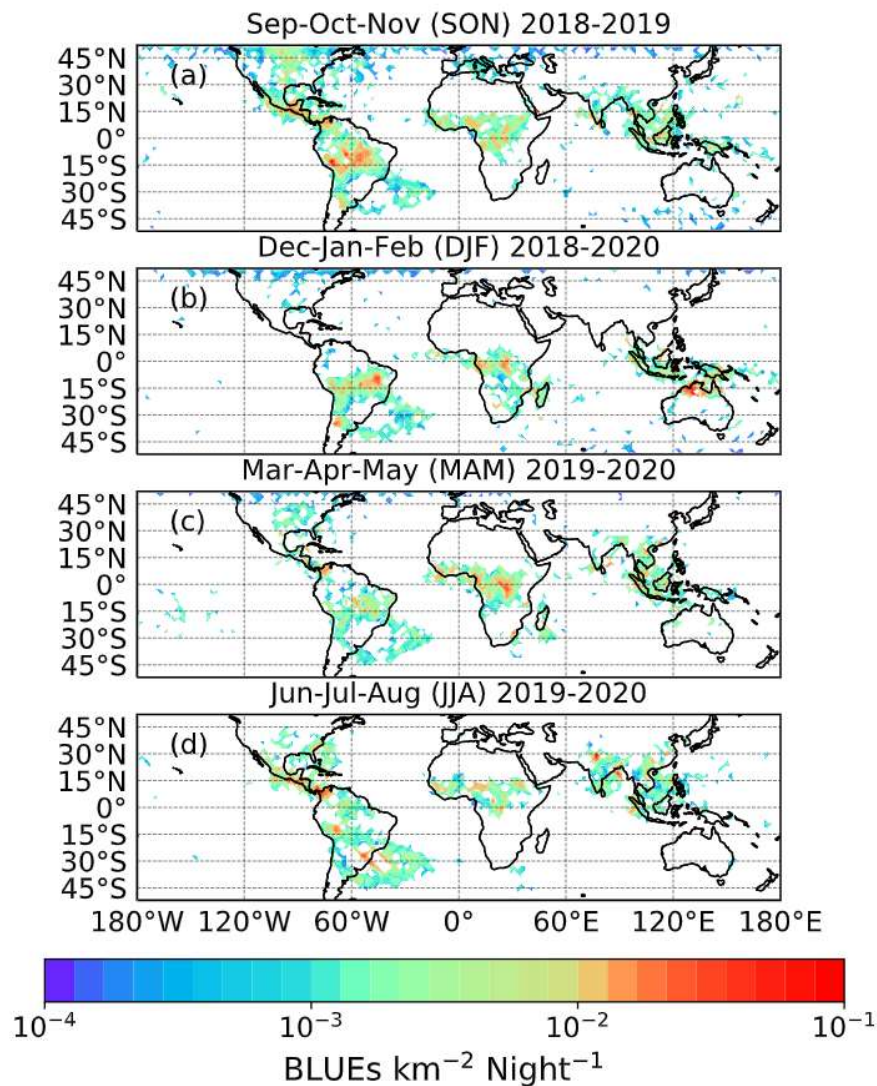
Figure 12. Nighttime seasonal distribution of BLUE electrical activity in thunderclouds. The global nighttime seasonal BLUE rates are: 8.2 (SON), 5.9 (DJF), 6.2 (MAM) and 6.7 (JJA) BLUES s -1 . Note that these global nighttime seasonal BLUE rates are biased (underestimated) due to the nighttime only ASIM-MMIA observation time mode (see Figure 14) that shortens as ISS moves since it is not a geostationary platform. Thus, the most representative nighttime BLUE rate would be that at 0 h local time (see Figure 14). These maps are generated using 2° × 2° grid cells where the sharp pixels of the image are smoothed by drawing level lines using the python function called contourf . Note that decimal logarithm is used in the colorbar. Non smooth seasonal maps are shown in Figure 25 of the SM.
