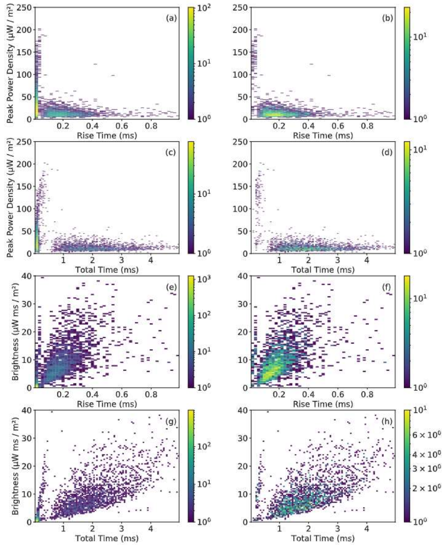
Figure 36. Variation of the peak power density (a)-(d) and total brightness (e)-(h) as a function of the GD-1 (left column) and GD-2 (right column) impulsive single pulse BLUE rise times (a, b, e, f) and total time (duration) (c, d, g, h). Note that the rise and total times are calculated as the elapsed times since the raw signal is above 10 % of the maximum until it reaches the maximum (rise time), and until it passes the maximum and decreases again to 10 % of the maximum (total time). Note that, always, GD-1 is in the left column and GD-2 is in the right column. The colorbar indicates number of events.
