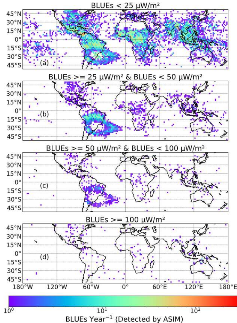
Figure 31. Geographical distribution (in 2^\circ \times 2^\circ grid cells) of the \sim 46,000 nighttime GD-1 BLUEs detected by ASIM-MMIA in the two-year period from 1 April 2019 to 31 March 2021. Panels (a), (b), (c) and (d) show BLUEs of any shape with peak power density (PPD) between \geq 3 \mu\text{W m}^{-2} and < 25 \mu\text{W m}^{-2} , between \geq 25 \mu\text{W m}^{-2} and < 50 \mu\text{W m}^{-2} , between \geq 50 \mu\text{W m}^{-2} and < 100 \mu\text{W m}^{-2} , and \geq 100 \mu\text{W m}^{-2} , respectively. There are 39980 BLUEs in panel (a) (19990/year), 4367 in panel (b) (2183.5/year), 833 in panel (c) (416.5/year), and 282 in panel (d) (141/year). The BLUEs shown in these maps can have any temporal shape, that is, no distinction has been made here among BLUEs with a single (impulsive or not) pulse, multiple pulses or any other irregular pulse shape.
