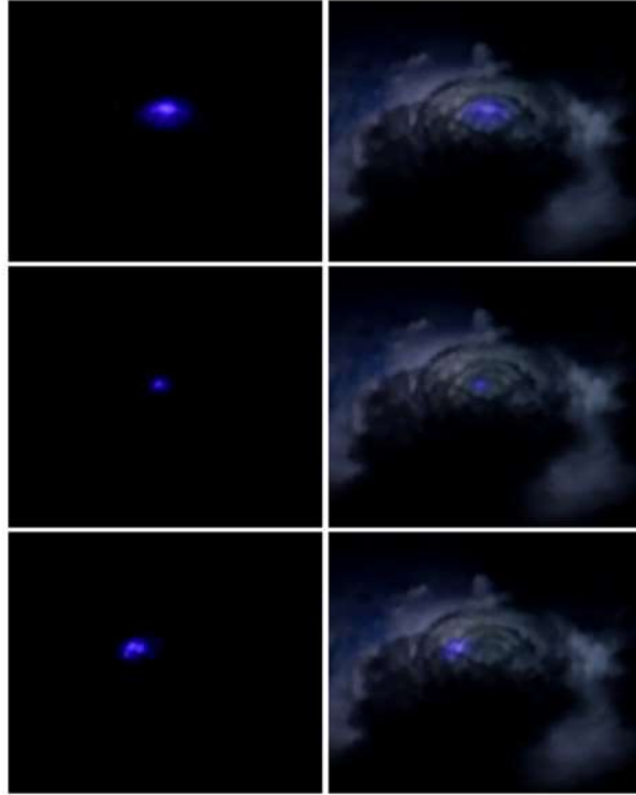
Figure 3. BLUE (corona) electrical discharges on the top of storm clouds (left column). Observed corona discharges from the ISS over-imposed on an image of the storm cloud (right column).
