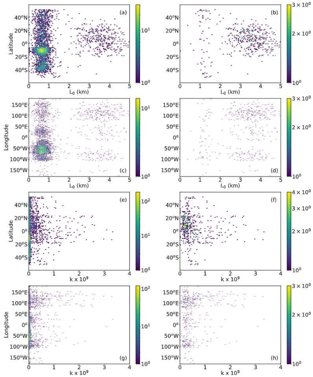
Figure 38. Zonal and meridional distributions of the lengths ( L_0 ) (a)-(d) and number of streamers ( k \times 10^9 ) (e)-(h) of impulsive single pulse BLUEs in GD-1 (left column) and GD-2 (right column). Note that, always, GD-1 is in the left column and GD-2 is in the right column. The colorbar indicates number of events.
