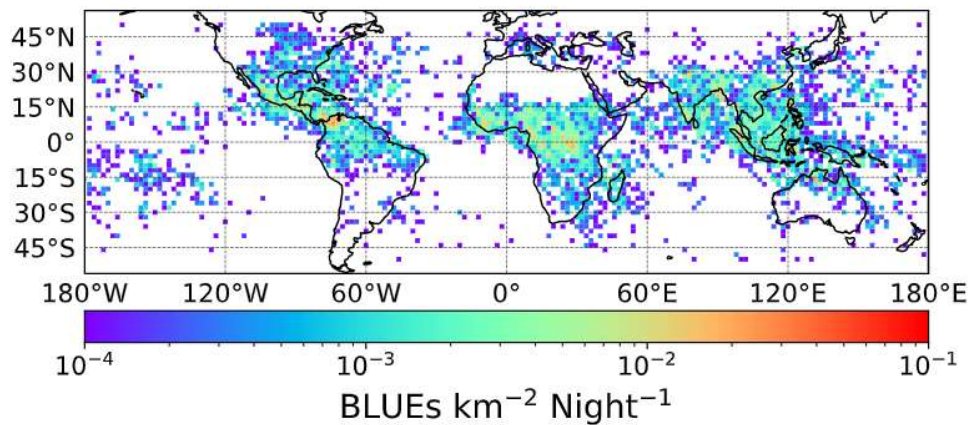
Figure 28. Two-year average (1 April 2019 through 31 March 2021) nighttime climatology of global BLUE electrical activity in thunderclouds (GD-2) removing events in all planet (including the SAA) with rise time ( \tau_{rise} \leq 40 \mu s ) and total duration ( \tau_{total} \leq 150 \mu s ). The map is generated using 2^\circ \times 2^\circ grid cells. Note that it is quite possible that not all the removed \sim 20000 events with respect to GD-1 are radiation belt particles and cosmic rays. Consequently, the number of BLUEs ( \sim 26,500 ) shown in this GD-2 distribution is most probably underestimated. The BLUEs shown can have any temporal shape, that is, no distinction has been made here among BLUEs with a single (impulsive or not) pulse, multiple pulses or any other irregular pulse shape. The annual global rate of GD-2 BLUEs peak at 5.5 \text{ events s}^{-1} in the local midnight (00.00 local solar time), and show a decreasing global rate as local daytime approaches (and there is less MMIA observation time). On average, the global annual average rate of BLUEs in GD-2 is 3.5 \text{ events s}^{-1} . Note that ASIM can only observe during the night.
