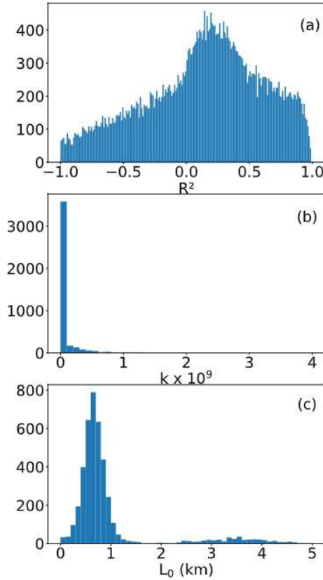
Figure 47. Histograms for BLUEs in GD-1 (see Figure 27 of main paper) recorded by ASIM-MMIA within 1 April 2019 to 31 March 2021. Events in panels (b) and (c) are fitted according to Li et al. (2021) assuming they are extended light sources that span altitudes from the cloud top to a maximum distance L_0 inside the cloud. The fit is over the time after the peak to obtain the best-fit cutoff (characteristic photon diffusion) time \tau_D = L_0^2/4D , and the total number of source photons ( N ) (Li et al., 2021). The different histograms show the number of BLUEs for different (a) R^2 (bin = 0.01), (b) Number of streamers ( k \times 10^9 ) (bin = 0.03) for events with R^2 > 0.75 , and (c) Vertical length ( L_0 ) (bin = 0.1) for events with R^2 > 0.75 . Please note that the word bin is used with the meaning of step.
