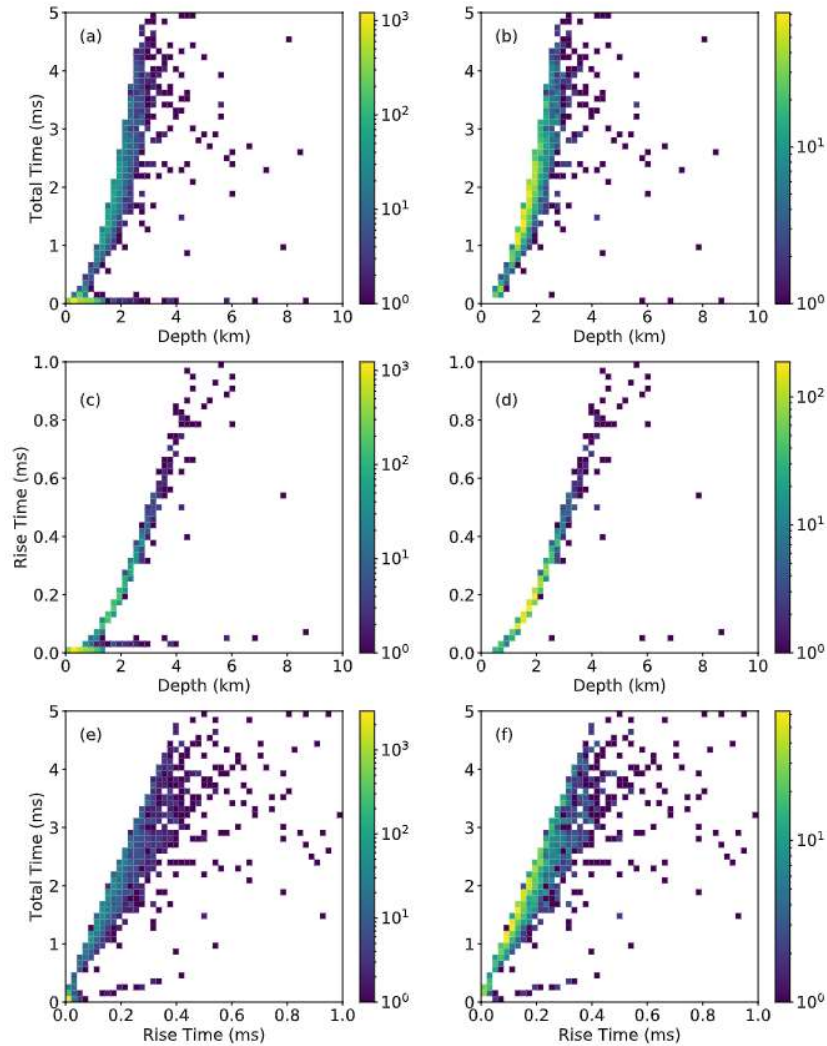
Figure 37. Total times (duration) and rise times of impulsive single pulse BLUEs in GD-1 (left column) and GD-2 (right column) as a function of depth (a)-(d). Panels (e) and (f) show the relationship between total times (duration) and rise times for GD-1 (left column) and GD-2 (right column). Note that panels (a, c) of GD-1 show the presence of some few unphysical events located deep (1-8 km below cloud tops) in thunderclouds characterized by simultaneously exhibiting very short total times ( \leq 200 \mu\text{s} ) and rise times ( \leq 60 \mu\text{s} ). This is mostly solved in panels (b, d) of GD-2. Note that, always, GD-1 is in the left column and GD-2 is in the right column. The colorbar indicates number of events.
