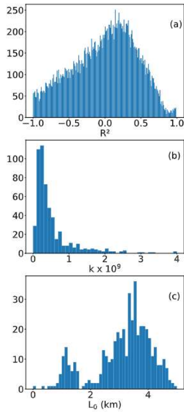
Figure 48. Histograms for BLUEs in GD-2 (see Figure 28 of main paper) recorded by ASIM-MMIA within 1 April 2019 to 31 March 2021. Events in panels (b) and (c) are fitted according to Li et al. (2021) assuming they are extended light sources that span altitudes from the cloud top to a maximum distance L_0 inside the cloud. The fit is over the time after the peak to obtain the best-fit cutoff (characteristic photon diffusion) time \tau_D = L_0^2/4D , and the total number of source photons ( N ) (Li et al., 2021). The different histograms show the number of BLUEs for different (a) R^2 (bin = 0.01), (b) Number of streamers ( k \times 10^9 ) (bin = 0.03) for events with R^2 > 0.75 , and (c) Vertical length ( L_0 ) (bin = 0.1) for events with R^2 > 0.75 . Please note that the word bin is used with the meaning of step.
