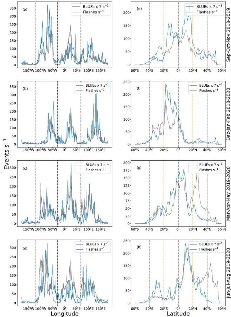
Figure 13. Seasonal meridional (left) and zonal (right) nighttime distributions of 2-year (1 September 2018 to 31 August 2020) BLUE climatology and ISS-LIS nighttime lightning in the same period. Grid cells and vertical lines as in Figure 11. Note that, for comparison, seasonal meridional/zonal 24 h (day and night) distribution of the two-year ISS-LIS lightning climatology is shown in Figure 22 of the SM. Note that the global seasonal BLUE rates are scaled up 7 times for best comparison with global nighttime lightning flash rates.
