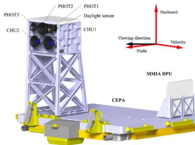
Figure 5. MMIA on the Columbus External Payloads Adaptor (CEPA). The Camera Head Units (CHUs) and the photometers (PHOTs) are mounted on an optical bench that sits on top of a support structure to avoid having the payload on the nadir-directed platform in the field of view. The instrument computer, the Data Processing Unit (DPU), is placed directly on the CEPA and is clad with a radiating shield for thermal control. The viewing direction is indicated by a black arrow in the ISS frame given by the velocity vector, the nadir and starboard direction (Chanrion et al., 2019).
