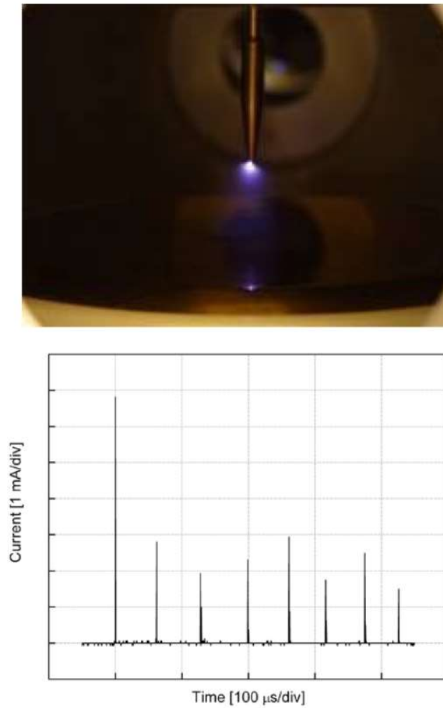
Figure 1. Negative corona in a short point-to-plane inter-electrode gap (top panel), and train of Trichel pulses (bottom panel) measured in ambient air (Halanda et al., 2012).
