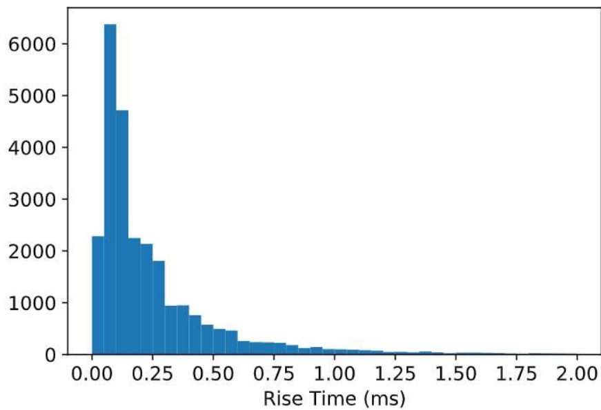
Figure 51. Histogram showing the number of BLUEs with all sort of temporal shapes (not only impulsive single pulse ones) geographically distributed according to GD-2 (see Figure 28 of main paper) with different rise times (ms) (bin = 0.05 ms). Please note that the word bin is used with the meaning of step.
