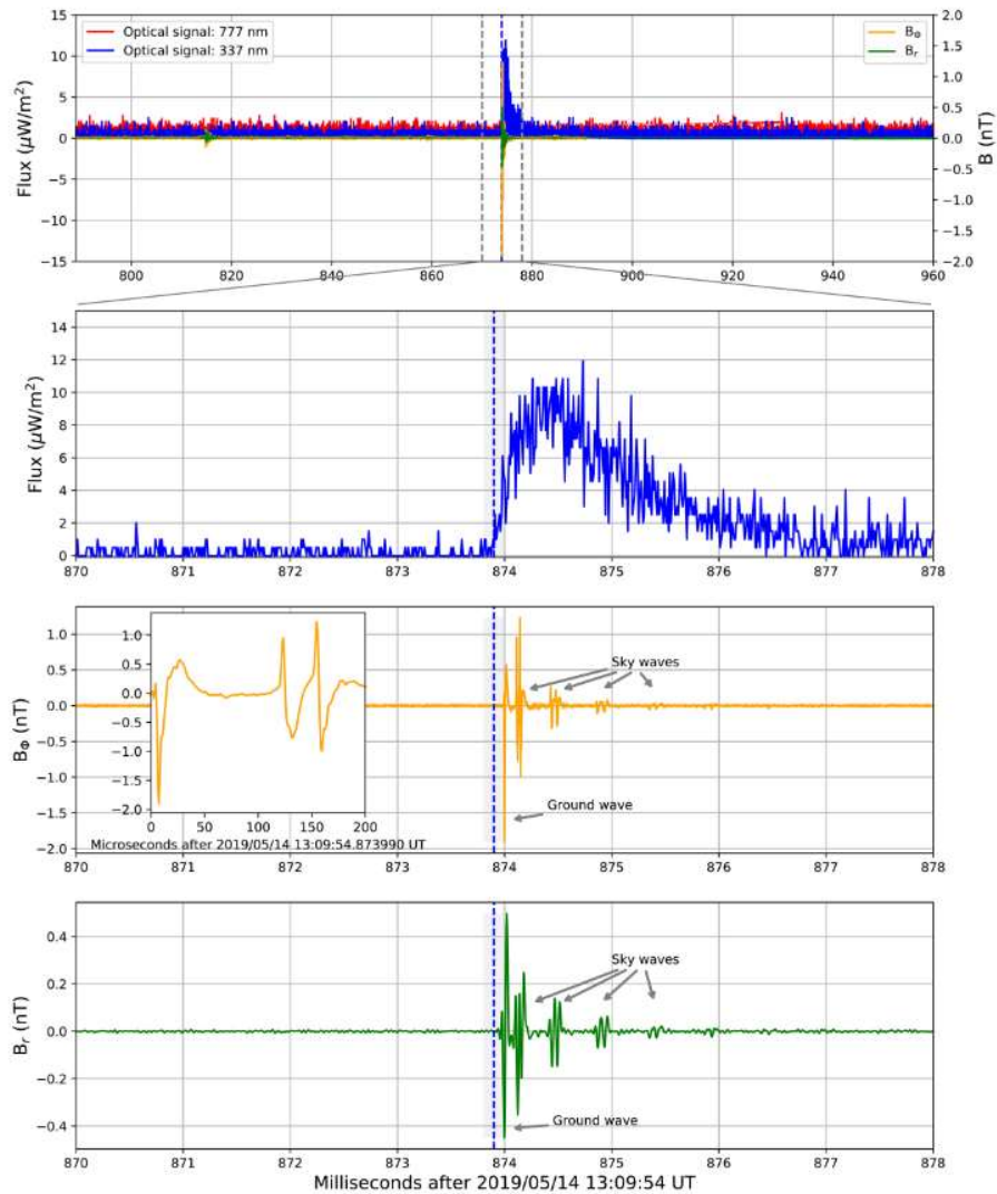
Figure 9. (Top panel) Comparison between the narrow single-pulse blue flash (blue line) detected by MMIA at 13:09:54.8739 UTC (source) \pm 0.1 ms (shadowed region in the three bottom panels) and the VLF spheric waveforms - B_r (green line) and B_\phi (orange line) magnetic field components - associated to the positive NBE detected at 13:09:54.87398350 UTC (source) \pm 50 ns by the Melaka VLF / LF station. Note that the 777.4 nm optical signal is at the noise level. Details of the optical signal and VLF series of this positive NBE can be seen in the three bottom panels where it is shown the zoomed-in of the top panel region around the spheric of the positive NBE. The inset in the B_\phi panel shows the \mu\text{s} time scale of the detected +NBE. The bipolar waveform of the +NBE ground wave lasts for about 25 \mu\text{s} .
