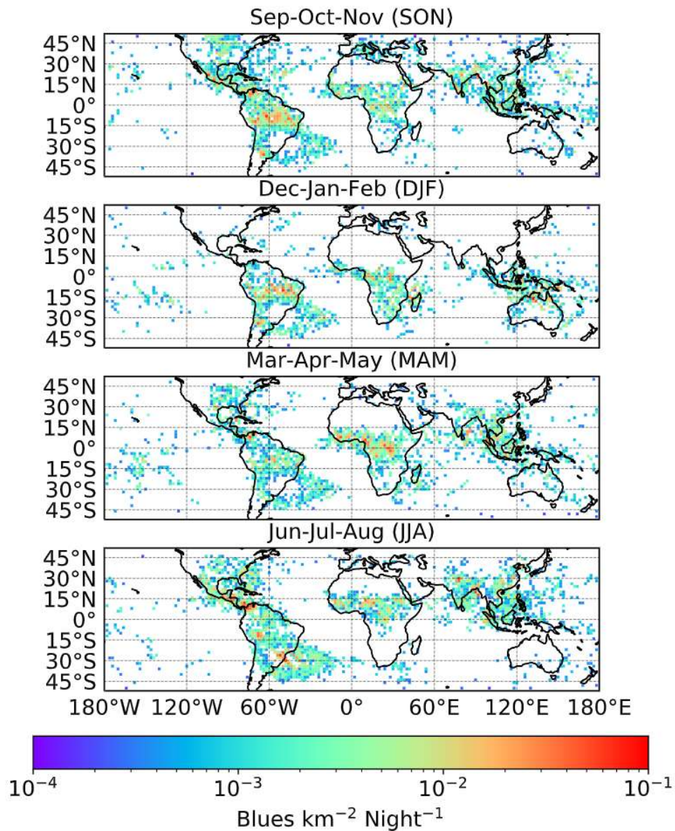
Figure 29. Nighttime seasonal distribution of BLUE electrical activity in thunderclouds associated to GD-1 in Figure 27. The global nighttime seasonal BLUE rates are: 6.7 (SON), 4.7 (DJF), 5.9 (MAM) and 6.8 (JJA) BLUEs s -1 . These maps are generated using 2° × 2° grid cells. The BLUEs shown can have any temporal shape, that is, no distinction has been made here among BLUEs with a single (impulsive or not) pulse, multiple pulses or any other irregular pulse shape.
