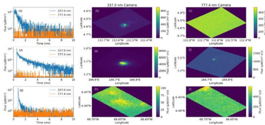
Figure 10. Three representative types of BLUEs investigated in this global study. The top, middle and bottom panels display the temporal shape, duration and intensity of the 337.0 nm and 777.4 nm photometer light curves (a, d, g), and the associated BLUE images in the 337.0 nm (b, e, h) and 777.4 nm (c, f, i) cameras (with 400 m pixel resolution). The impulsive behaviour of the 337.0 nm is clearly seen in the three cases while noise level signals are simultaneously detected in the 777.4 nm photometer and camera of common BLUEs (a, b, c and g, h, i panels). The (d, e, f) panels present the case of a possible Blue Starter, which include measurable 777.4 nm signals due to its leader and a 337.0 nm camera image that is saturated. The 337.0 nm light (photometer) curve of the Blue Starter hardly lasts beyond 4 ms, while the duration of the 777.4 nm light curve is about 2 ms. The three BLUEs shown occurred (from top to bottom) on 14 April 2019 at 04:49:41 UTC, 26 Feb 2019 15:10:41 UTC and 23 July 2019 at 08:15:36 in Lon, Lat ( 131.25^{\circ}\text{W} , 4.99^{\circ}\text{S} ) middle of Pacific ocean, ( 164.60^{\circ}\text{E} , 3.11^{\circ}\text{S} ) east of Solomon Islands, and ( 67.58^{\circ}\text{W} , 6.01^{\circ}\text{N} ) north of Puerto Ayacucho in Colombia very close to the border with Venezuela, respectively.
