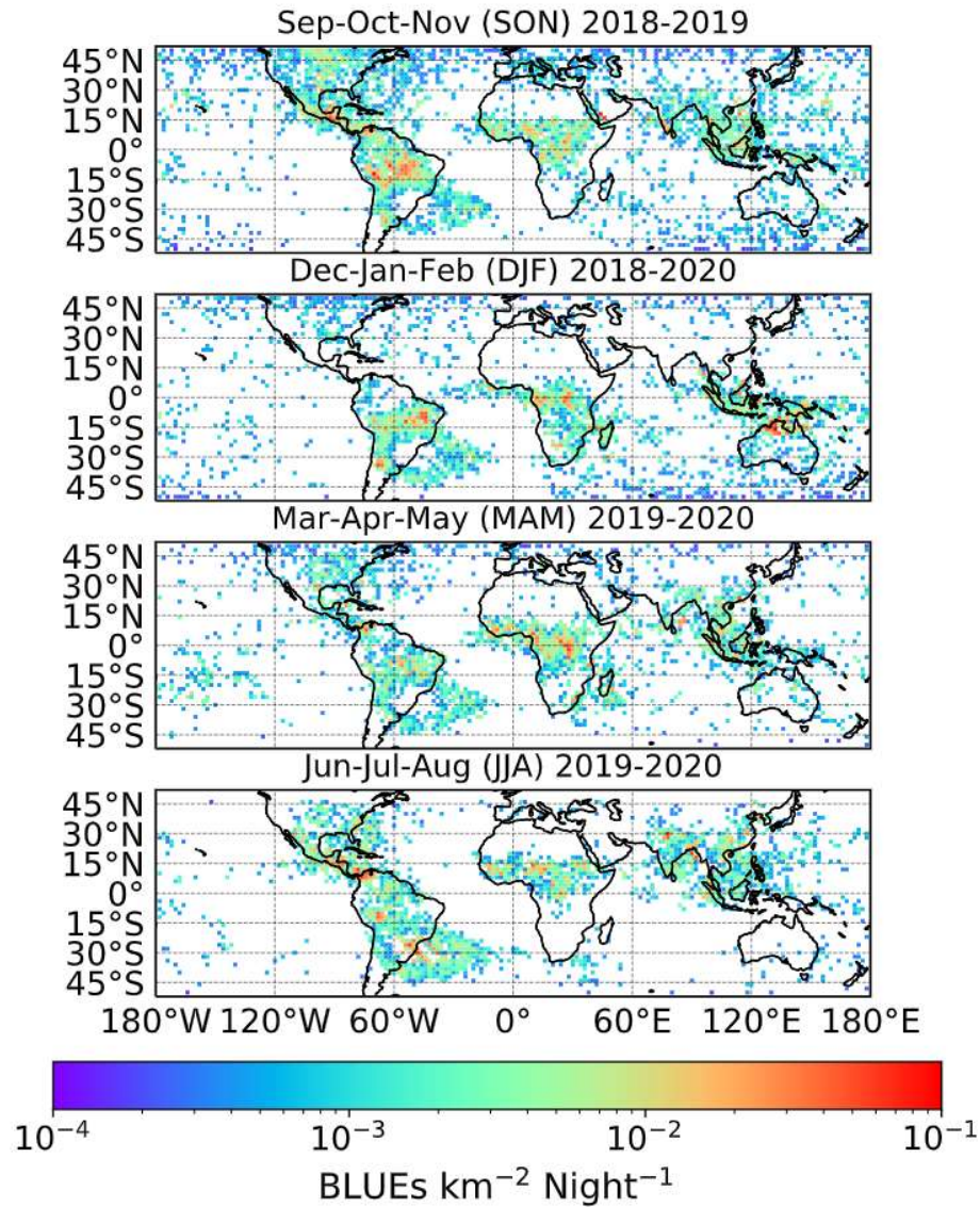
Figure 25. Non smooth nighttime seasonal distribution of BLUE electrical activity in thunderclouds. September to November (top panel), December to February (second panel from top), March to May (third panel from top), June to August (bottom panel). These non smooth maps are generated using 2^\circ \times 2^\circ grid cells. Note that the scale in the colorbar is the same as that in Figure 11 of the main paper.
