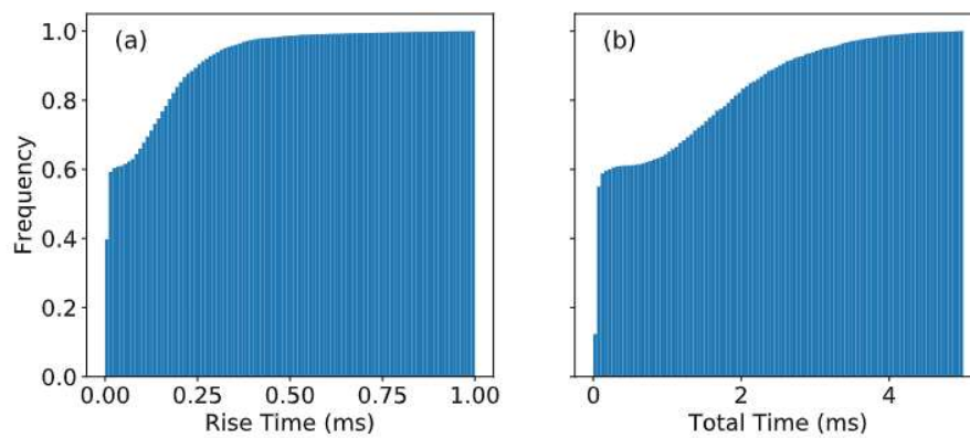
Figure 49. Frequency histograms showing the cumulative frequency of impulsive single pulse BLUEs (with R^2 > 0.75 ) in GD-1 (see Figure 27 of main paper) with different (a) Rise Times (ms) (bin = 0.01 ms) and (b) Total times (ms) (bin = 0.05 ms). These histograms indicate that, for instance, 60 % of impulsive single pulse BLUEs among all BLUEs in GD-1 have rise times and durations \leq 30 \mu\text{s} and \leq 300 \mu\text{s} , respectively. Note that GD-1 (in Figure 1 of main paper) represents the geographical distribution of BLUEs with all sort of temporal shapes, not only impulsive single pulse ones. Please note that the word bin is used with the meaning of step.
