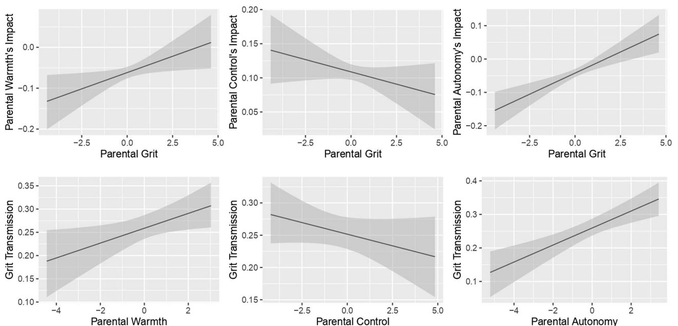
Fig. 1 Marginal Effects for the Interactions based on Models 7–9. Note. Y axis shows the effect of parenting dimensions (first row) given all levels of grit and the effect of parental grit (grit variation)
