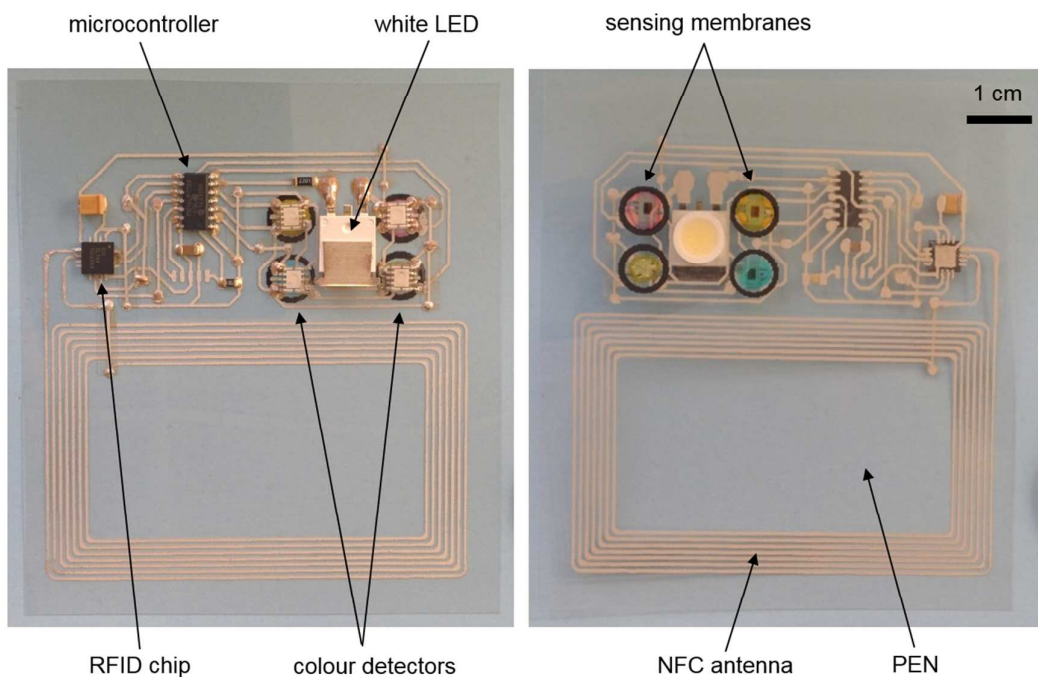
Figure 3. Photography of both sides of the developed tag.
