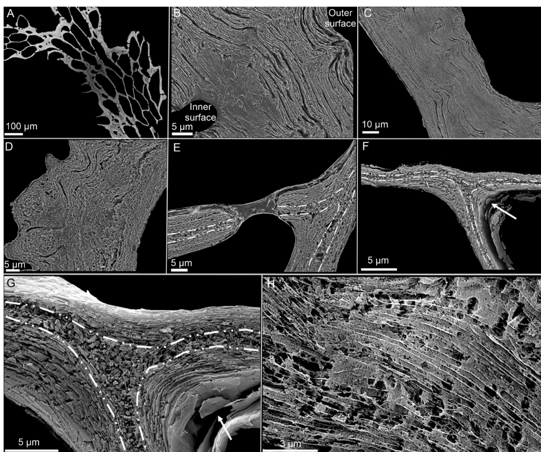
Figure 5. Morphology and microstructure of H. robusta (A). Polished and partly decalcified colony. (B–D) External wall section showing the multi-layered undulating patterning that flattens progressively toward the inner surface. The peaks correspond to the external protuberances. (E–G) Cross section of an inner wall. The sections are entirely composed of tabular calcite (arrow in F), except for the central granular layer (marked with dashed lines). (H) Details showing the organic membranes running uninterruptedly between the lamellae of polygonal tablets.
