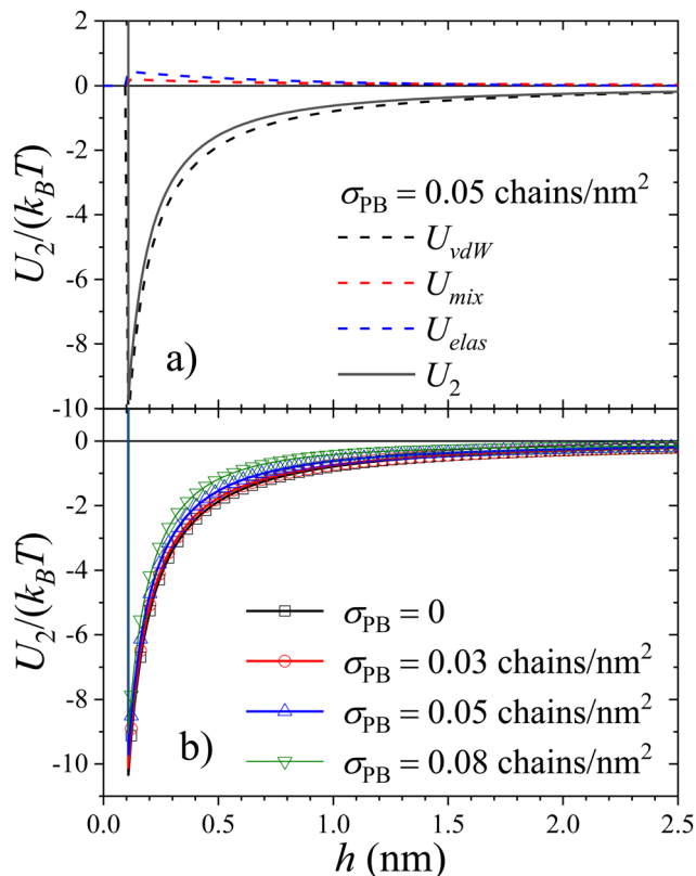
Fig. 3 (a) van der Waals, mixing, and elastic contribution to the total pair interaction potential, U_2 , evaluated for \sigma_{\text{PB}} = 0.05 chains per nm 2 . (b) Total pair interaction potential for different surface density of grafted PB polymers.
