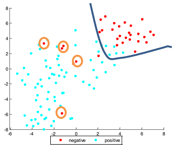
(b) Echo
