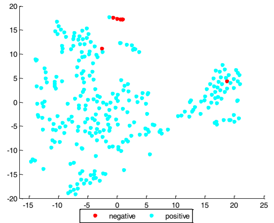
(b) Ecoli 0_1_3_7 vs 2_6
