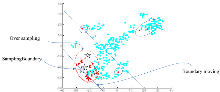
Fig. 4. Ecoli0147vs2356.
