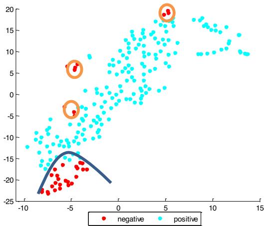
(c) newthyroid1
