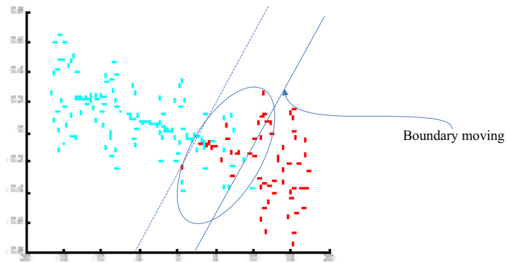
Fig. 3. Wine1.
