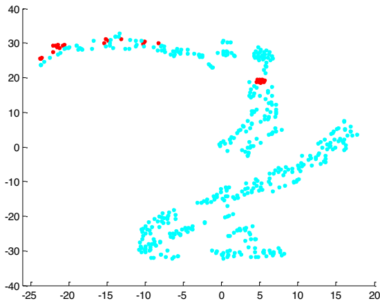
(a) Pageblocks13vs4
