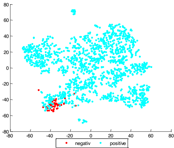
(a) Yeast 5
