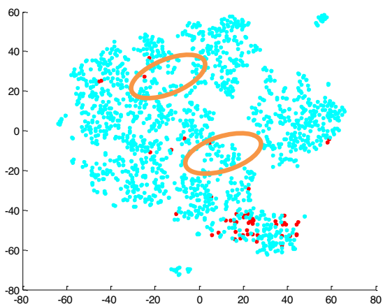
(a) Yeast 4
