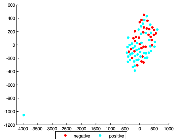
(b) Hepatitis
